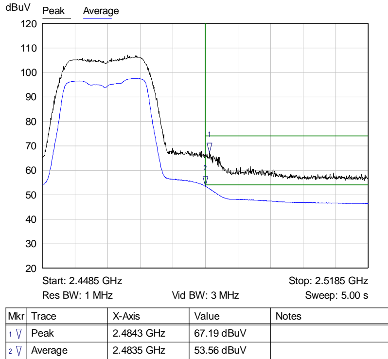
Graph 45: Radiated Upper Band Edge Plot
