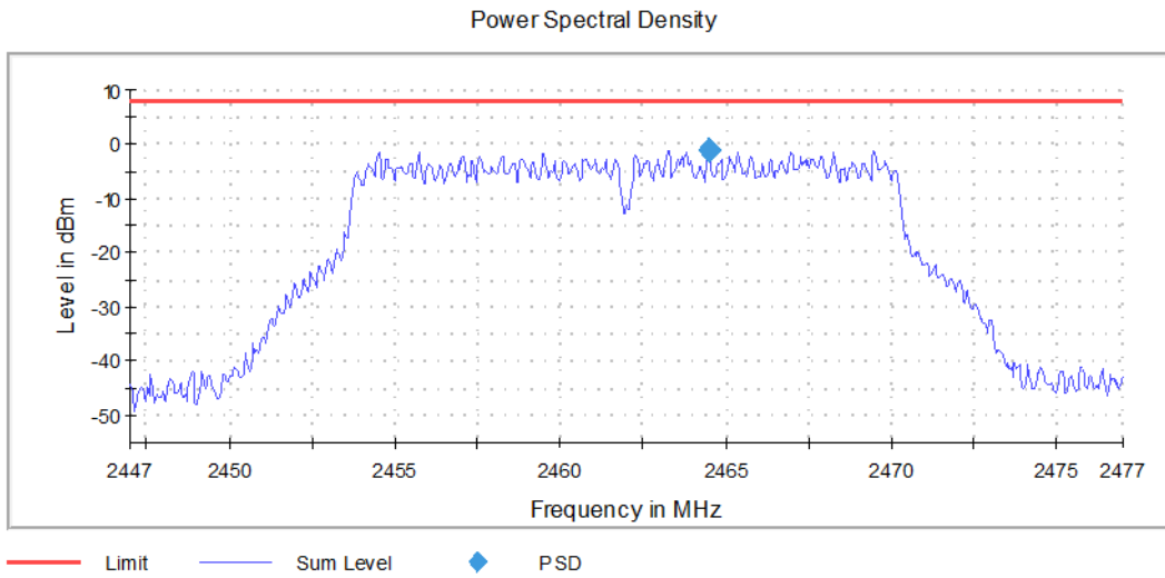
Graph 32: Highest Channel PSD
