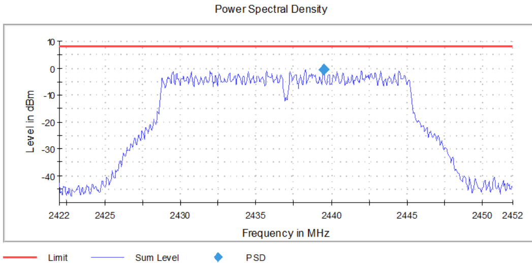
Graph 31: Middle Channel PSD
