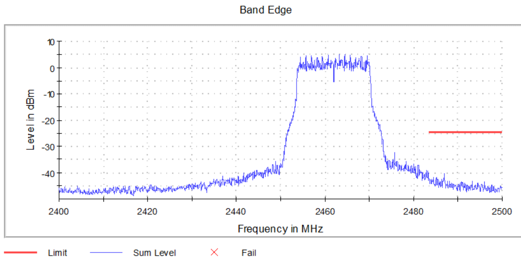
Graph 27: Upper Band Edge Plot
