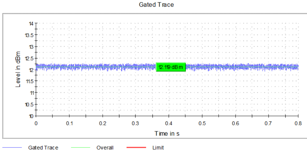
Graph 36: Lowest Channel Output Power
