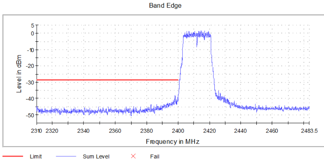
Graph 42: Lower Band Edge Plot
