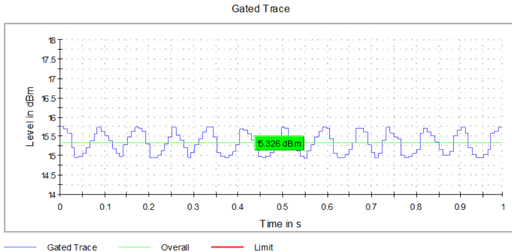
Graph 6: Highest Channel Output Power
