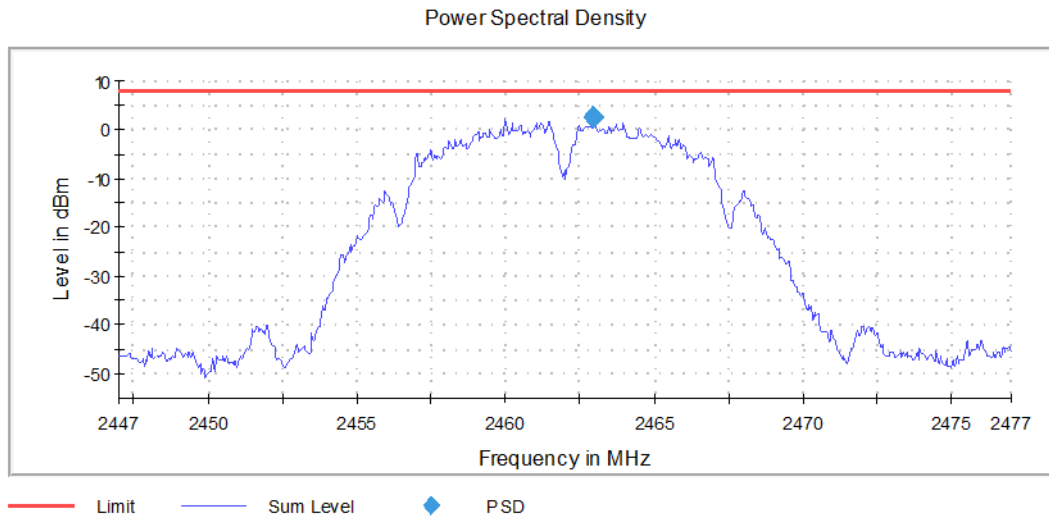
Graph 16: Highest Channel PSD
