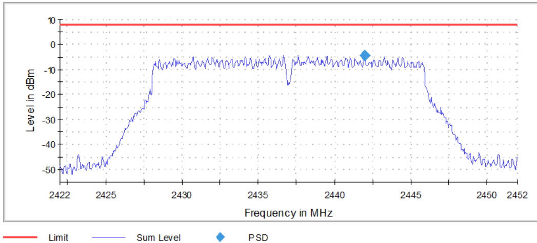
Graph 47: Middle Channel PSD
