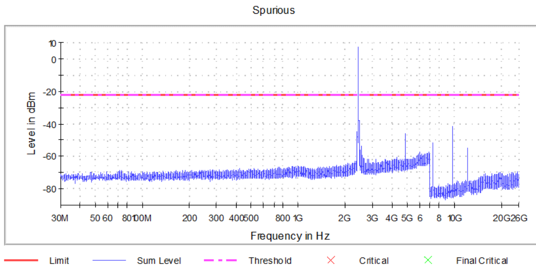
Graph 8: Transmitting on the Middle Channel
