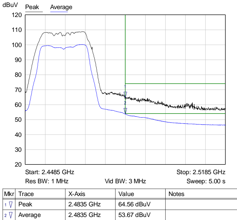
Graph 29: Radiated Upper Band Edge Plot
