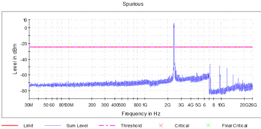
Graph 23: Transmitting on the Lowest Channel
