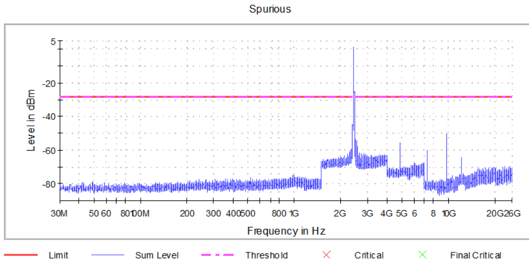
Graph 41: Transmitting on the Highest Channel
