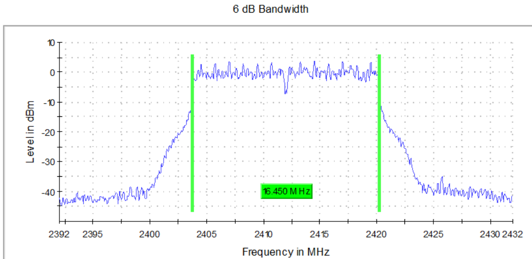
Graph 17: Lowest Channel Bandwidth
