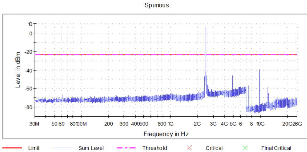
Graph 9: Transmitting on the Highest Channel
