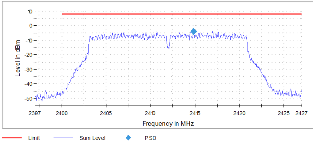
Graph 46: Lowest Channel PSD
