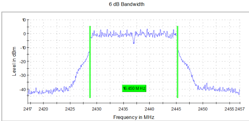
Graph 18: Middle Channel Bandwidth
