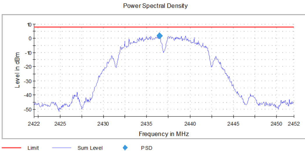
Graph 15: Middle Channel PSD
