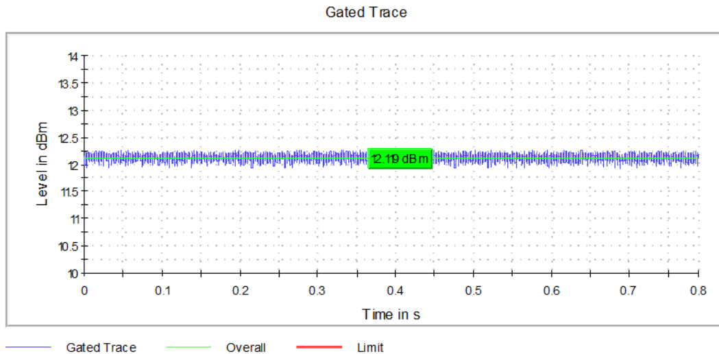
Graph 38: Highest Channel Output Power
