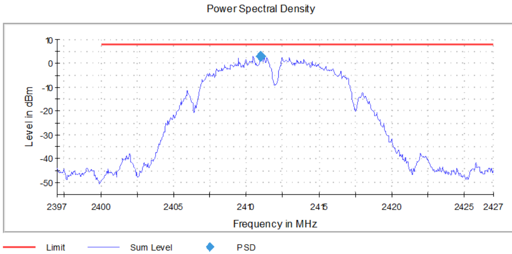
Graph 14: Lowest Channel PSD
