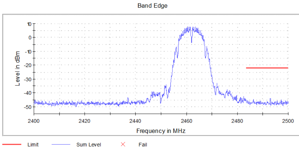
Graph 11: Upper Band Edge Plot
