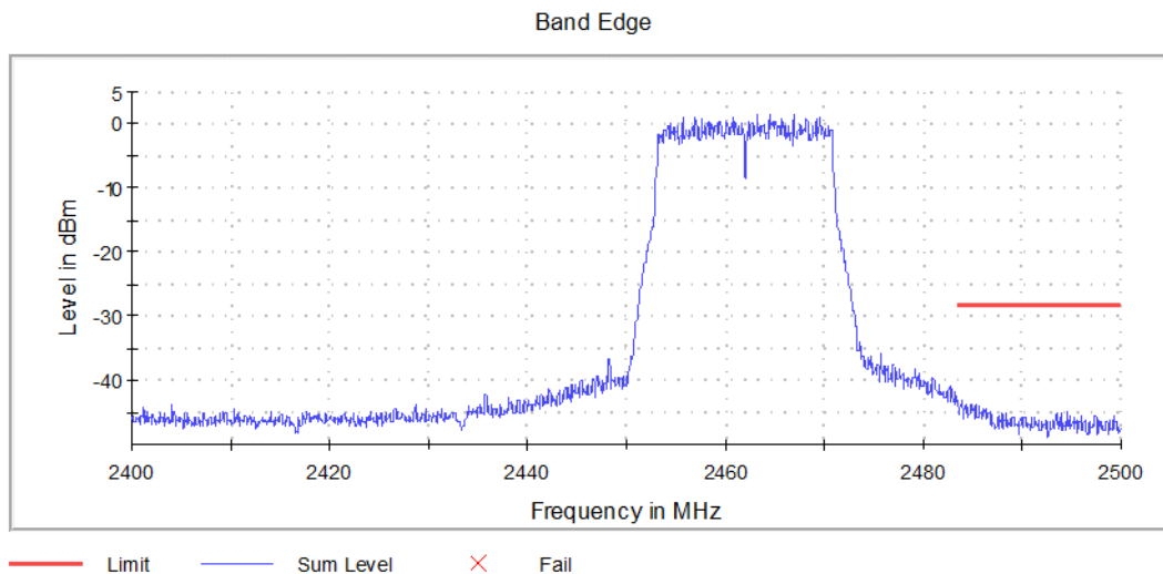
Graph 43: Upper Band Edge Plot
