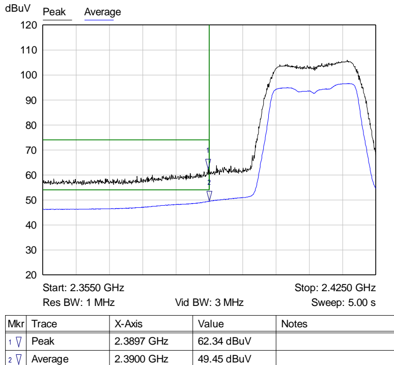
Graph 44: Radiated Lower Band Edge Plot
