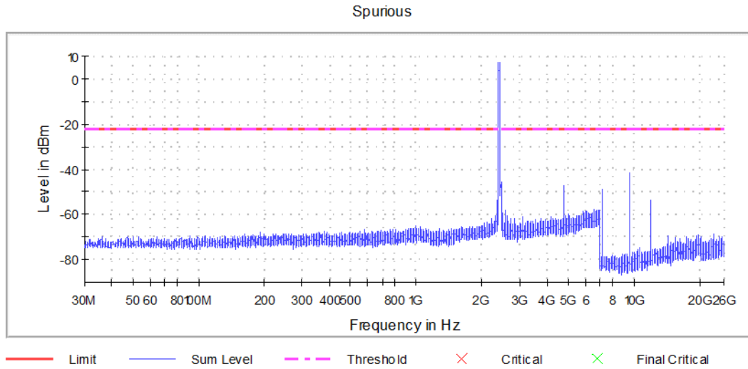
Graph 7: Transmitting on the Lowest Channel
