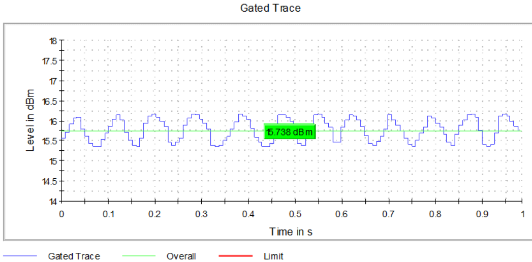
Graph 4: Lowest Channel Output Power
