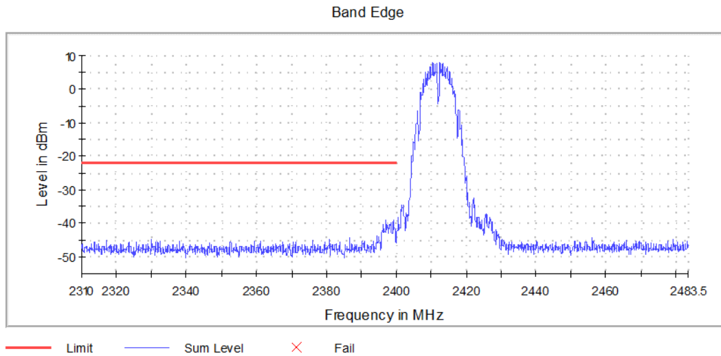
Graph 10: Lower Band Edge Plot
