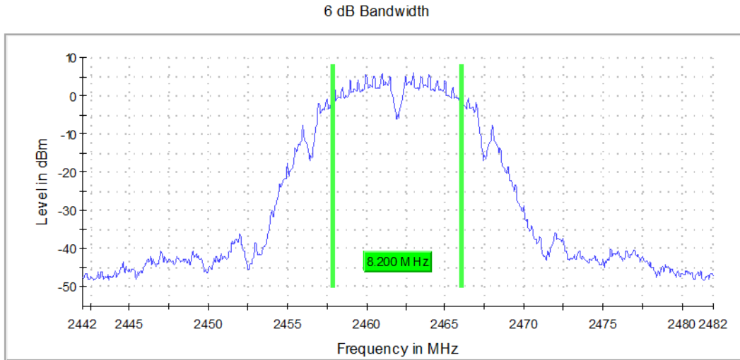
Graph 3: Highest Channel Bandwidth
