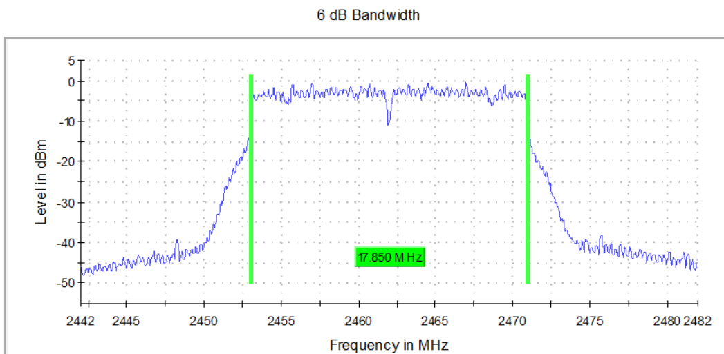
Graph 34: Middle Channel Bandwidth
