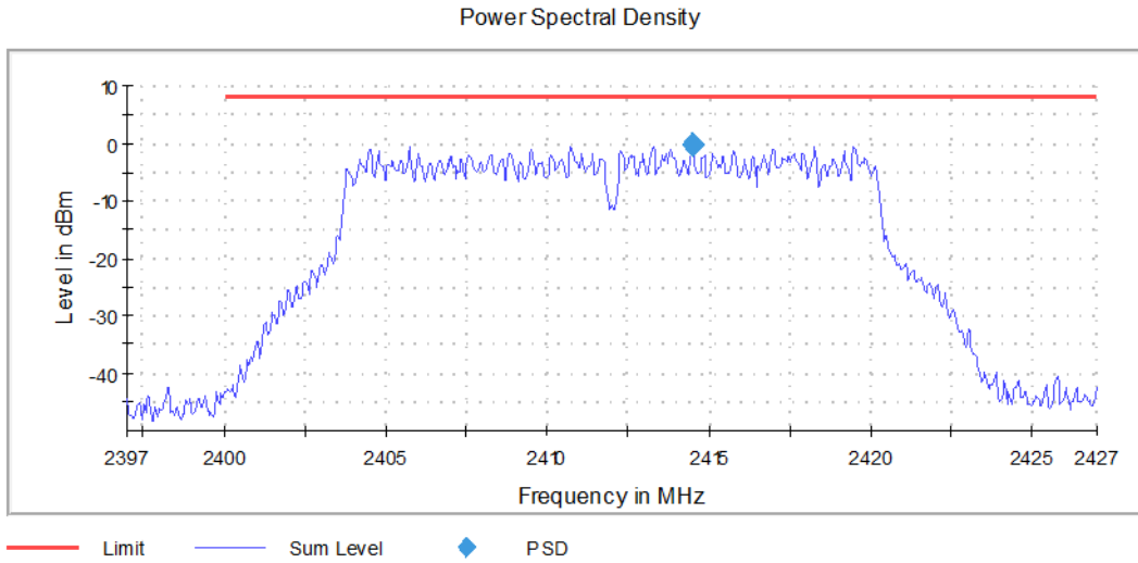
Graph 30: Lowest Channel PSD
