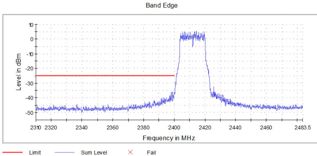
Graph 26: Lower Band Edge Plot
