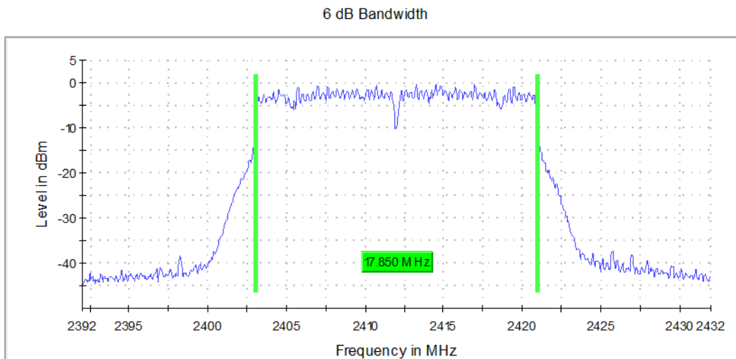
Graph 33: Lowest Channel Bandwidth
