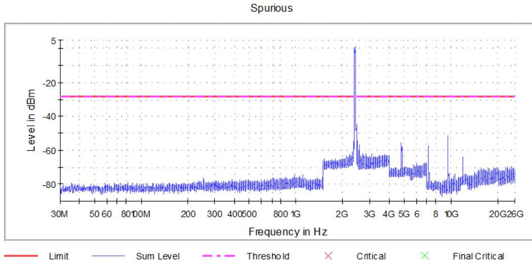
Graph 39: Transmitting on the Lowest Channel
