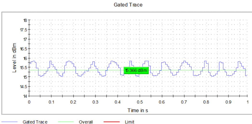
Graph 5: Middle Channel Output Power
