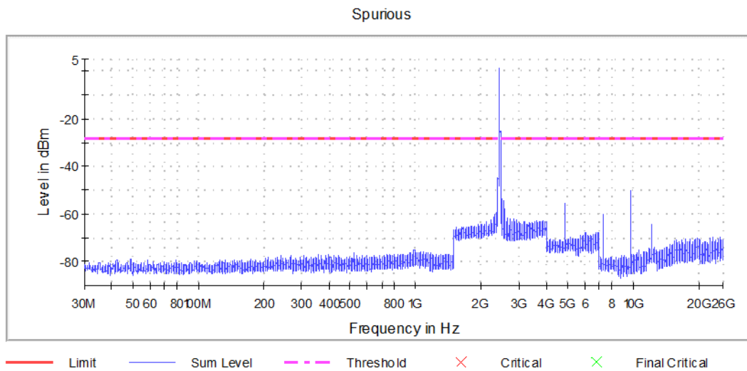
Graph 40: Transmitting on the Middle Channel
