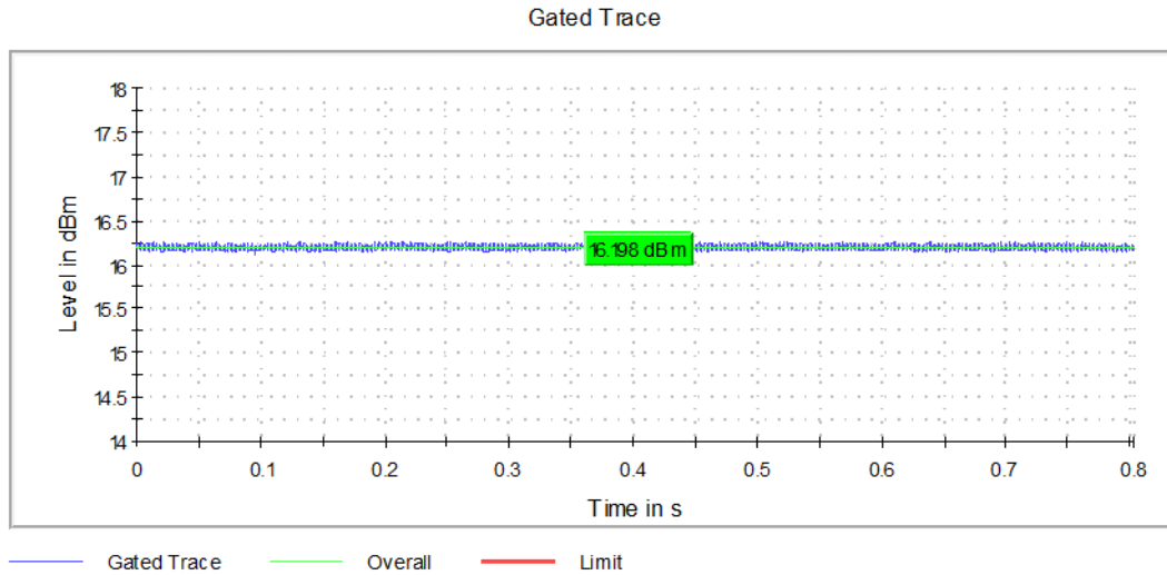
Graph 20: Lowest Channel Output Power
