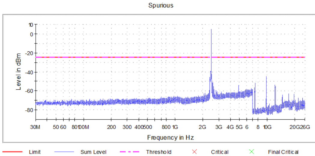
Graph 25: Transmitting on the Highest Channel
