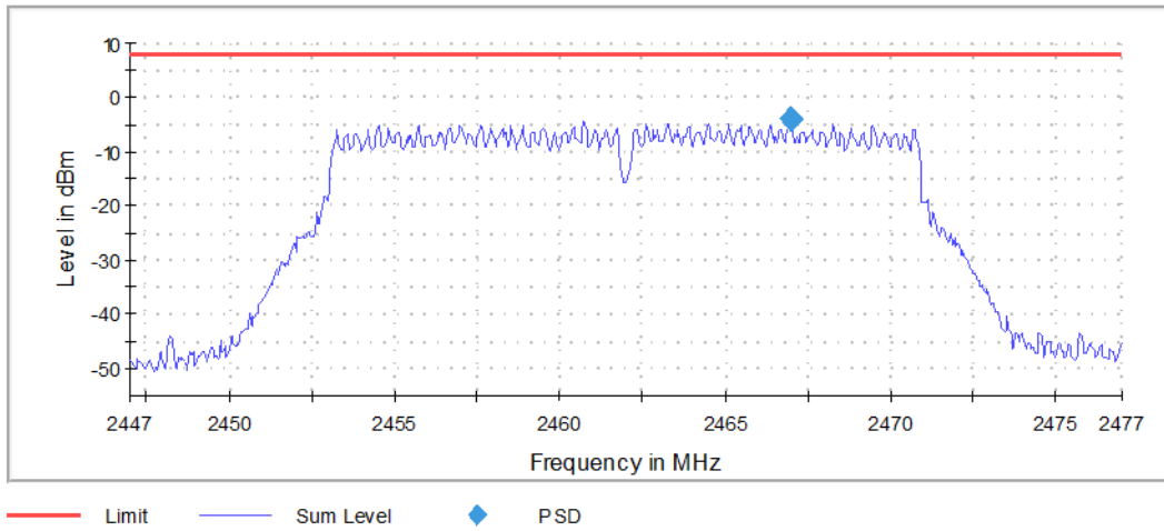
Graph 48: Highest Channel PSD
