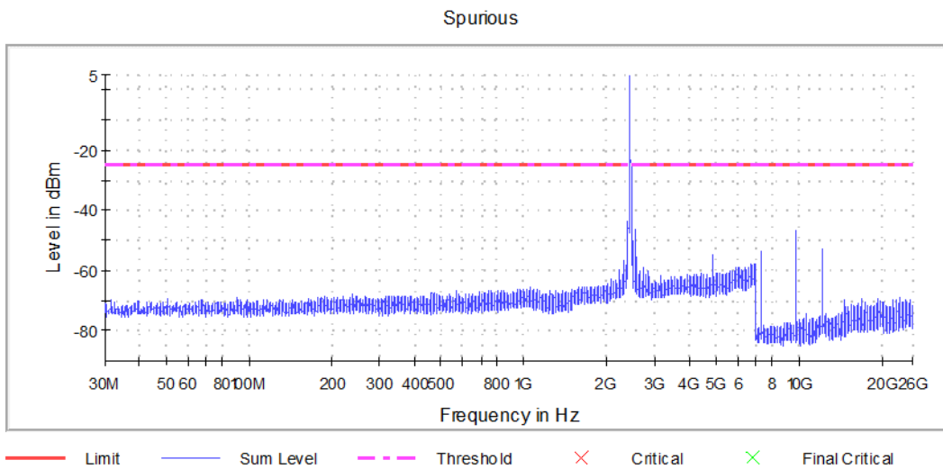
Graph 24: Transmitting on the Middle Channel
