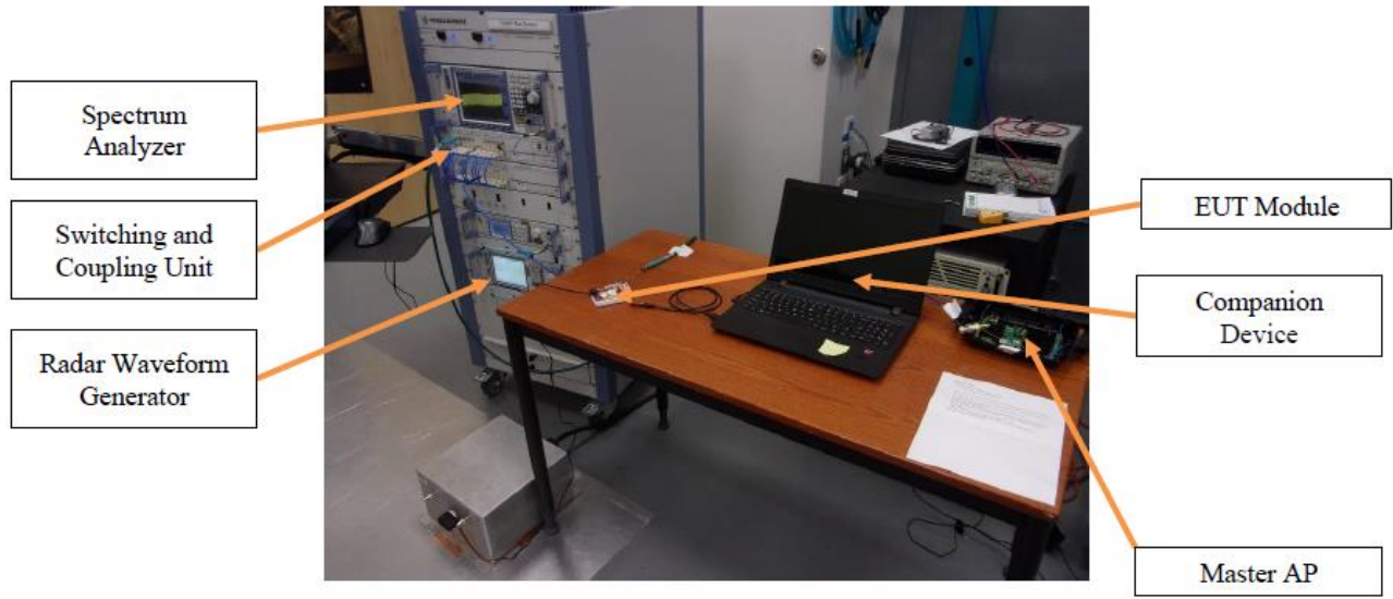
Photograph 9: DFS Test Setup
