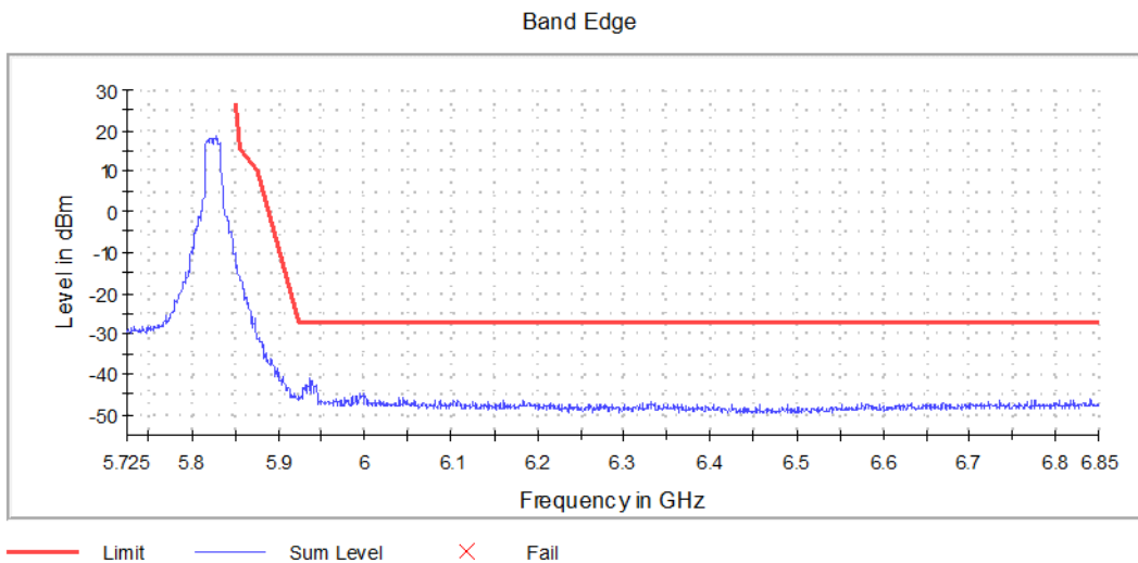
Graph 8: Upper Band Edge Channel 165 Transmitting (5825 MHz)
