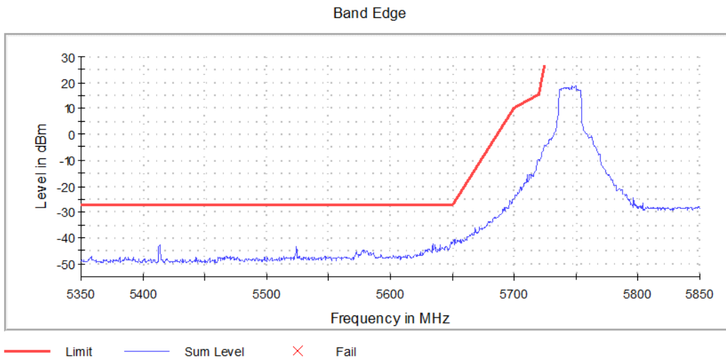
Graph 7: Lower Band Edge Channel 149 Transmitting (5745 MHz)
