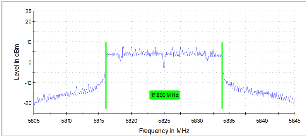
Graph 6: 6 dB Emissions Bandwidth Transmitting at 5825 MHz
