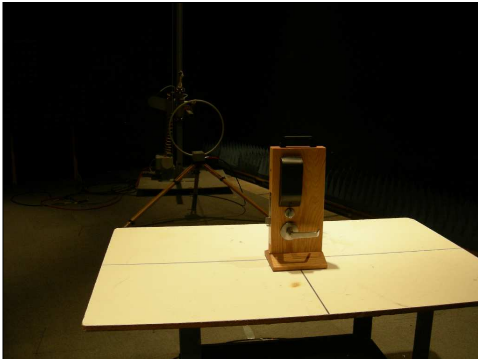
Figure 3: Radiated Emissions – 125kHz Prox
