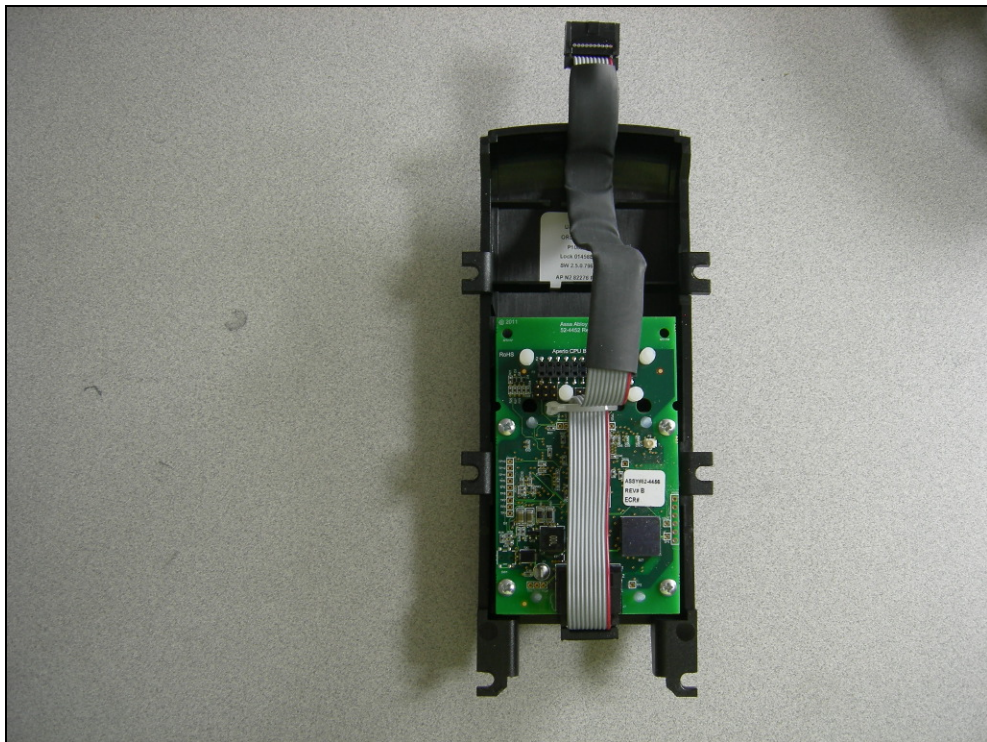
Figure 2: Internal Photo – Boards Installed
