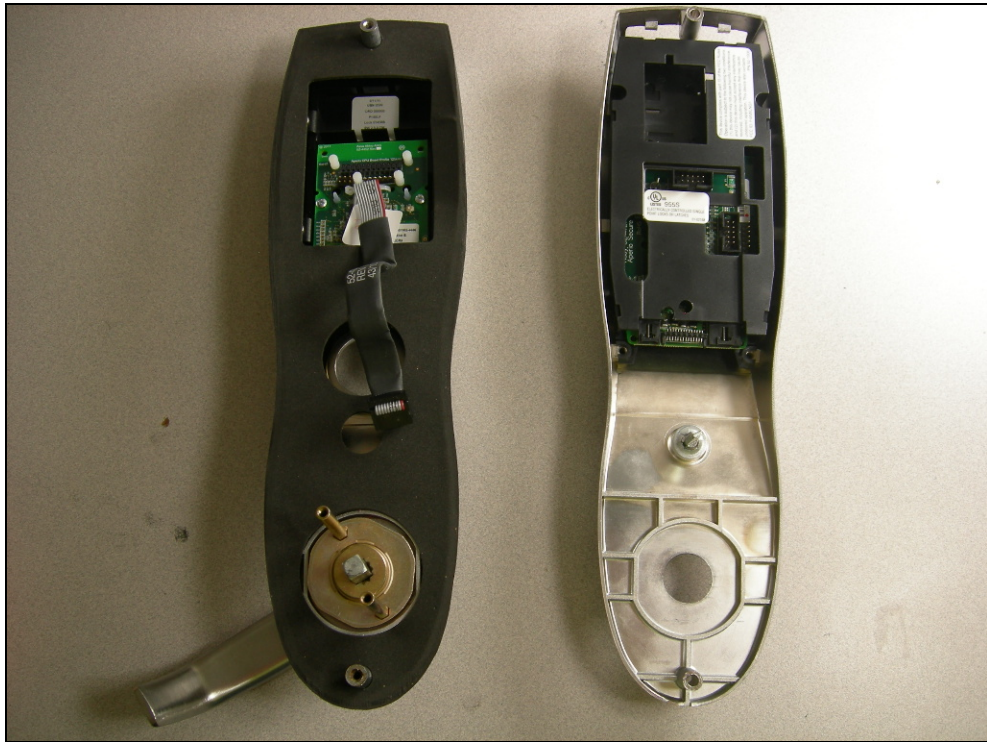
Figure 1: Internal Photo – Boards Installed
