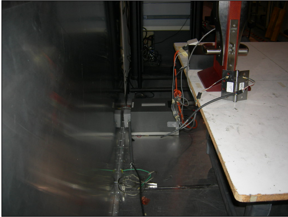
Figure 17: Conducted Emissions – TCW11-M802/M803 (Aux PWR)
