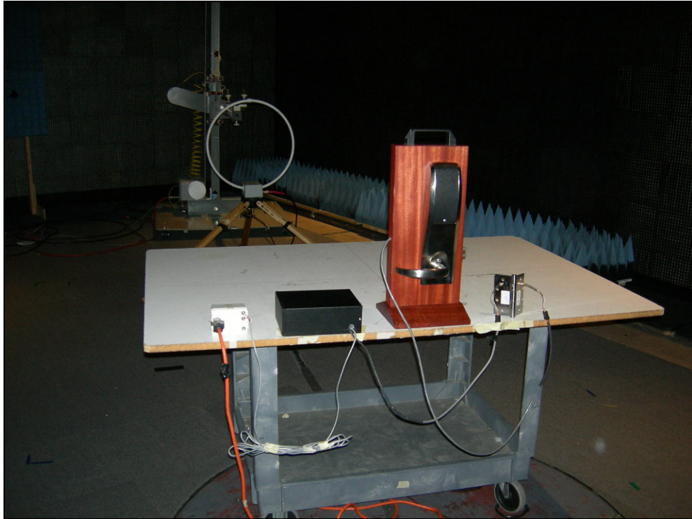
Figure 10: Radiated Emissions – TCWI1-M802/M803 (Aux PWR)
