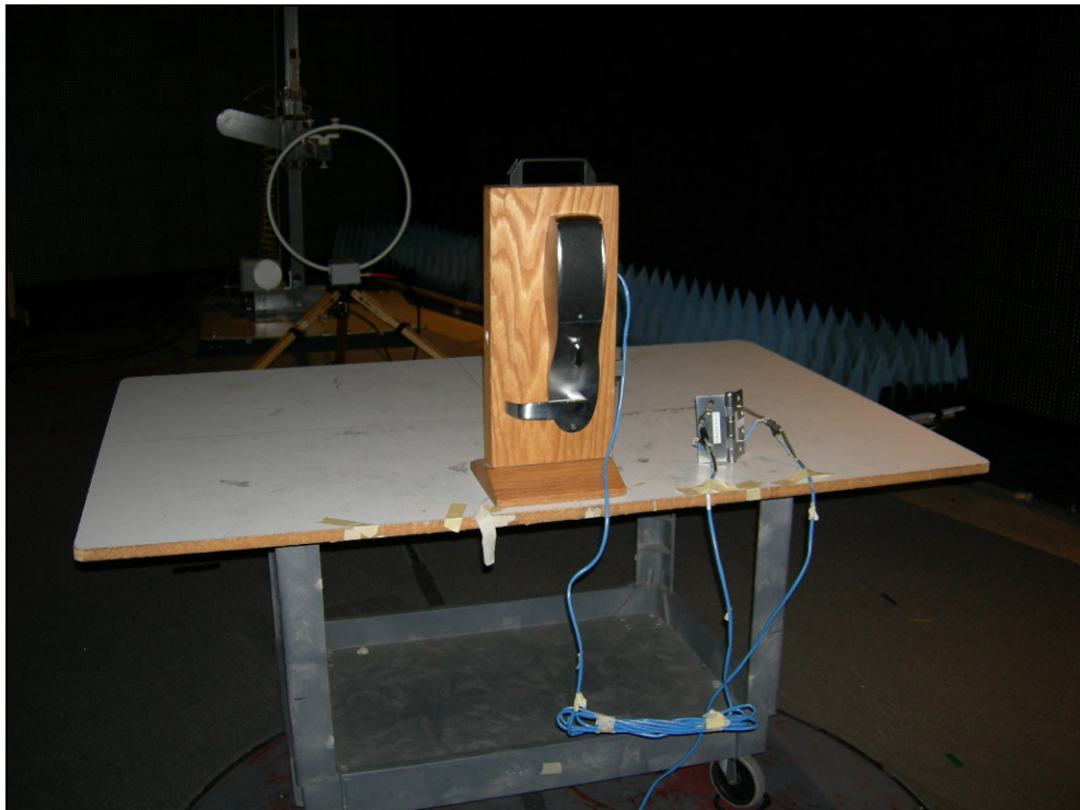
Figure 2: Radiated Emissions – S1-PA/PK
