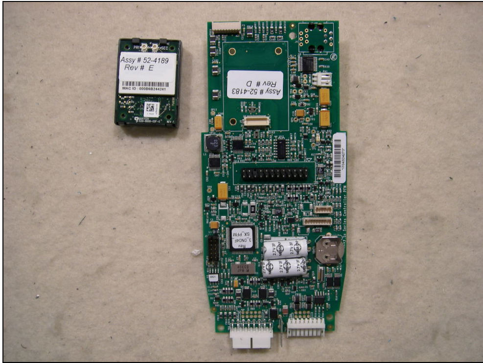
Figure 5: Controller PCB (Including Wifi Option)
