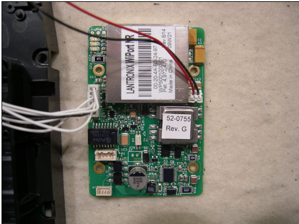
Figure 2: Ethernet PCB
