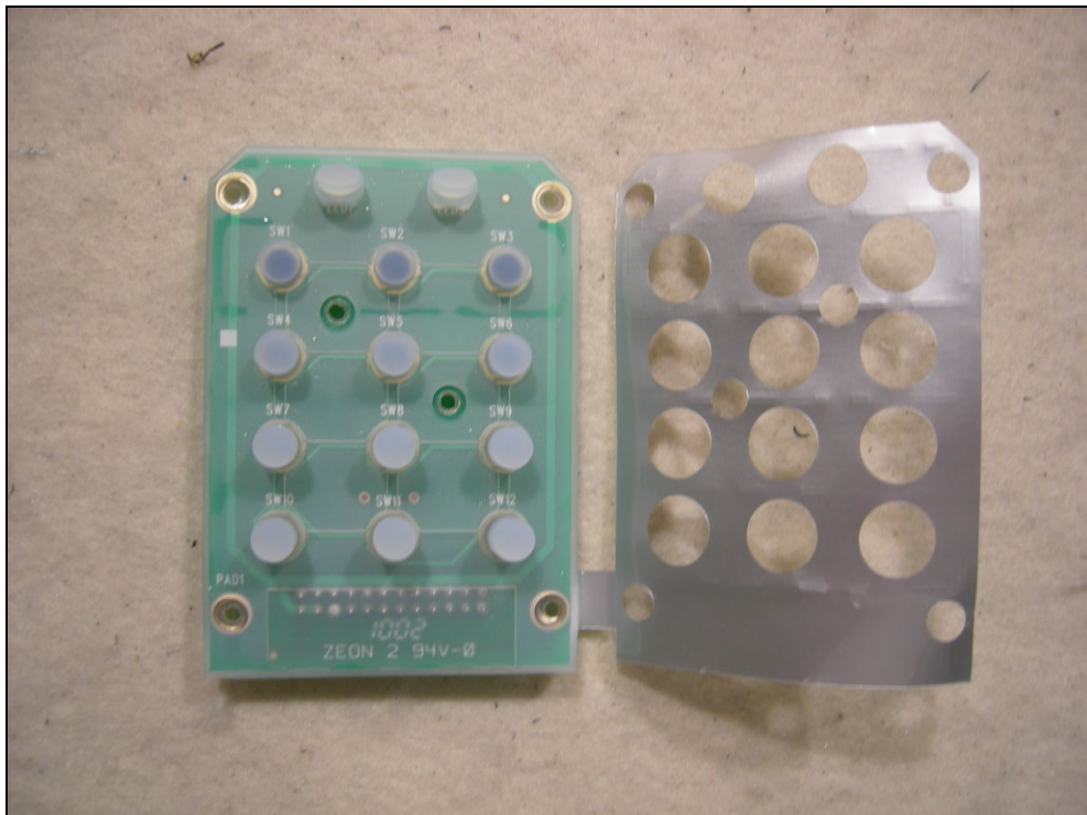
Figure 10: Keypad
