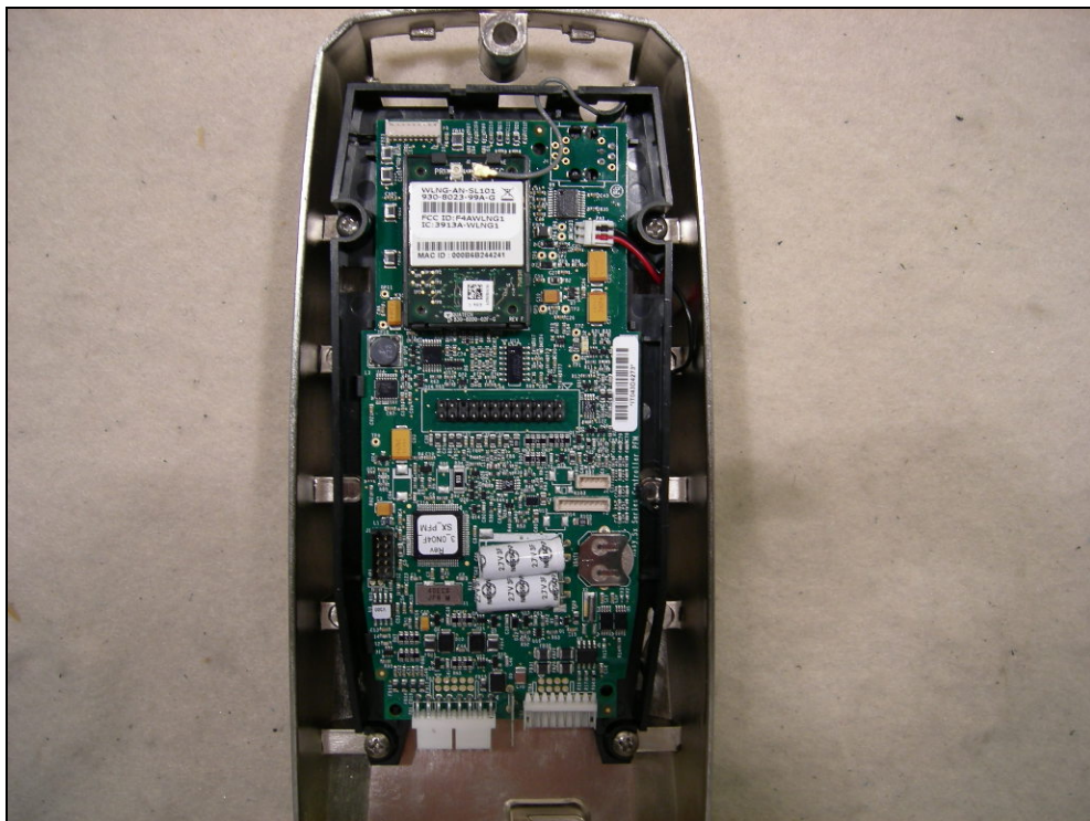
Figure 4: Controller PCB (Including Wifi Option)
