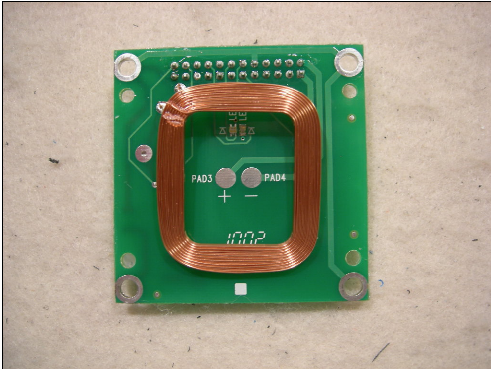
Figure 9: Coil Antenna
