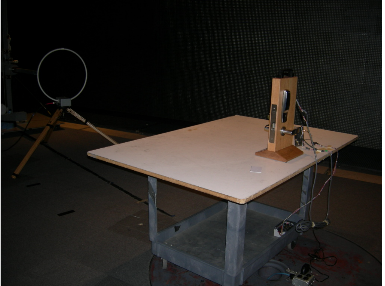
Figure 2: Radiated Emissions - Mortise
