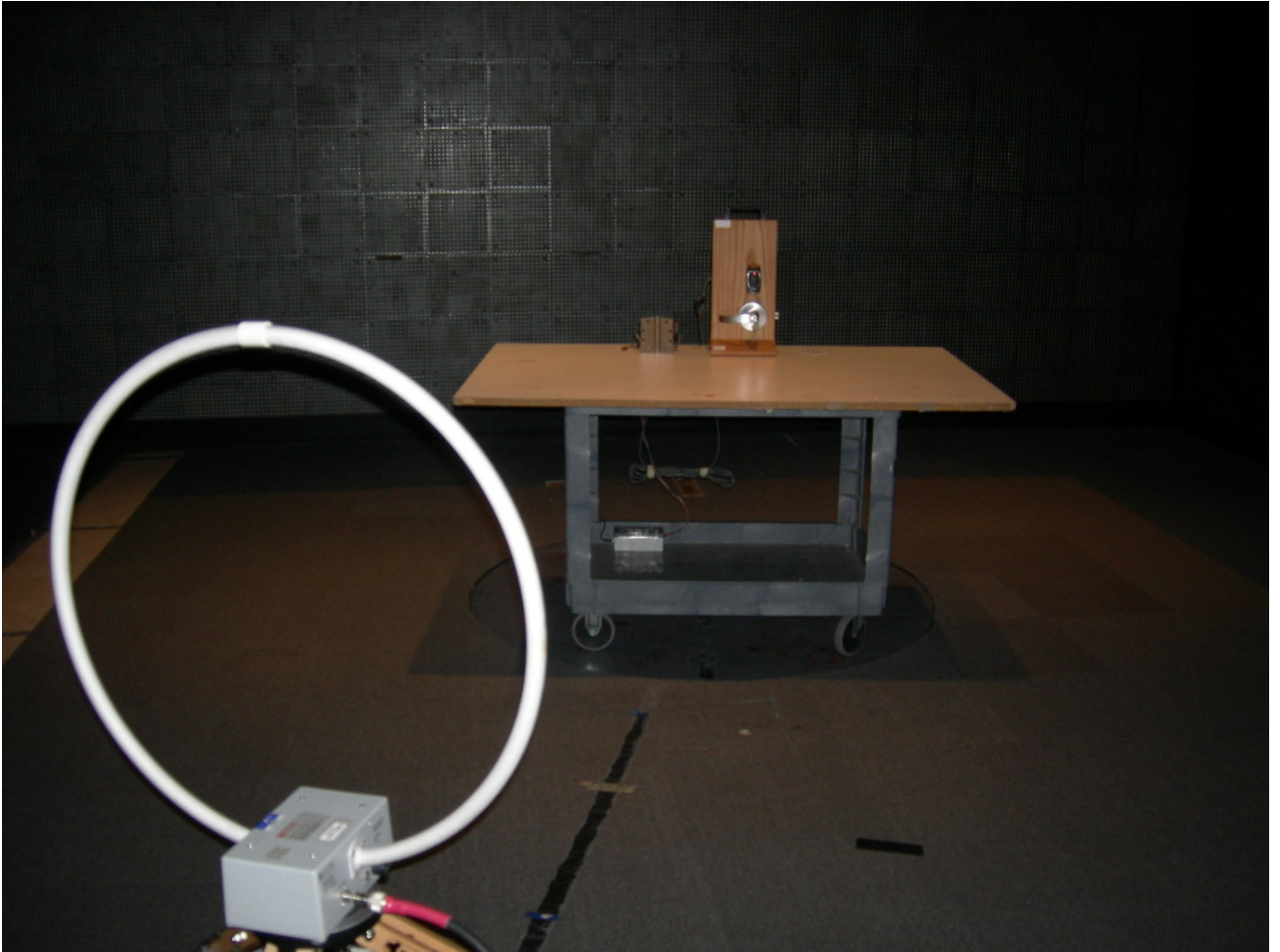
Figure 3: Radiated Emissions – Bored/Exits
