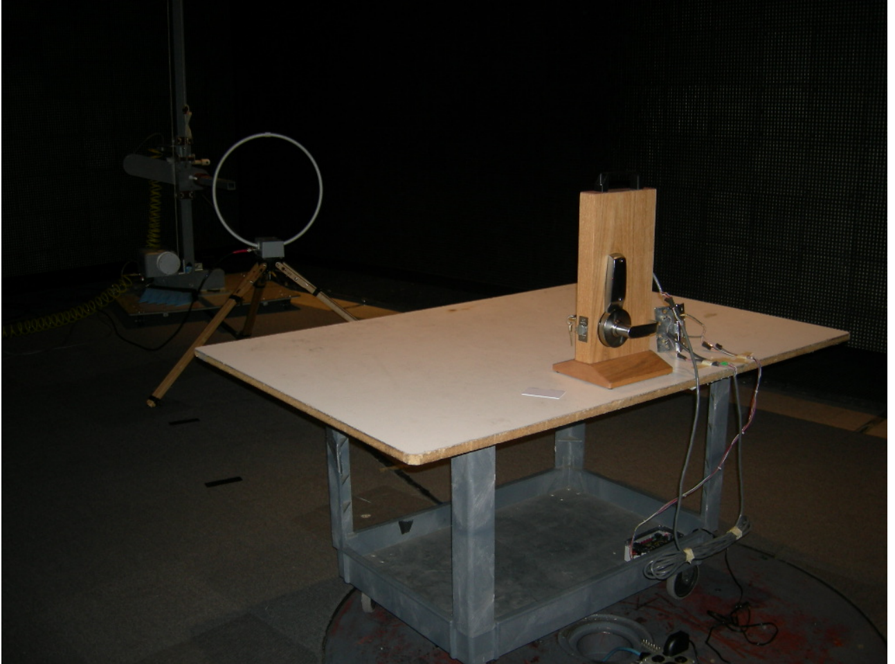
Figure 4: Radiated Emissions – Bored/Exits
