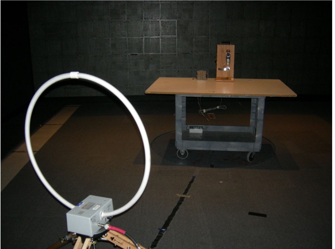
Figure 1: Radiated Emissions - Mortise
