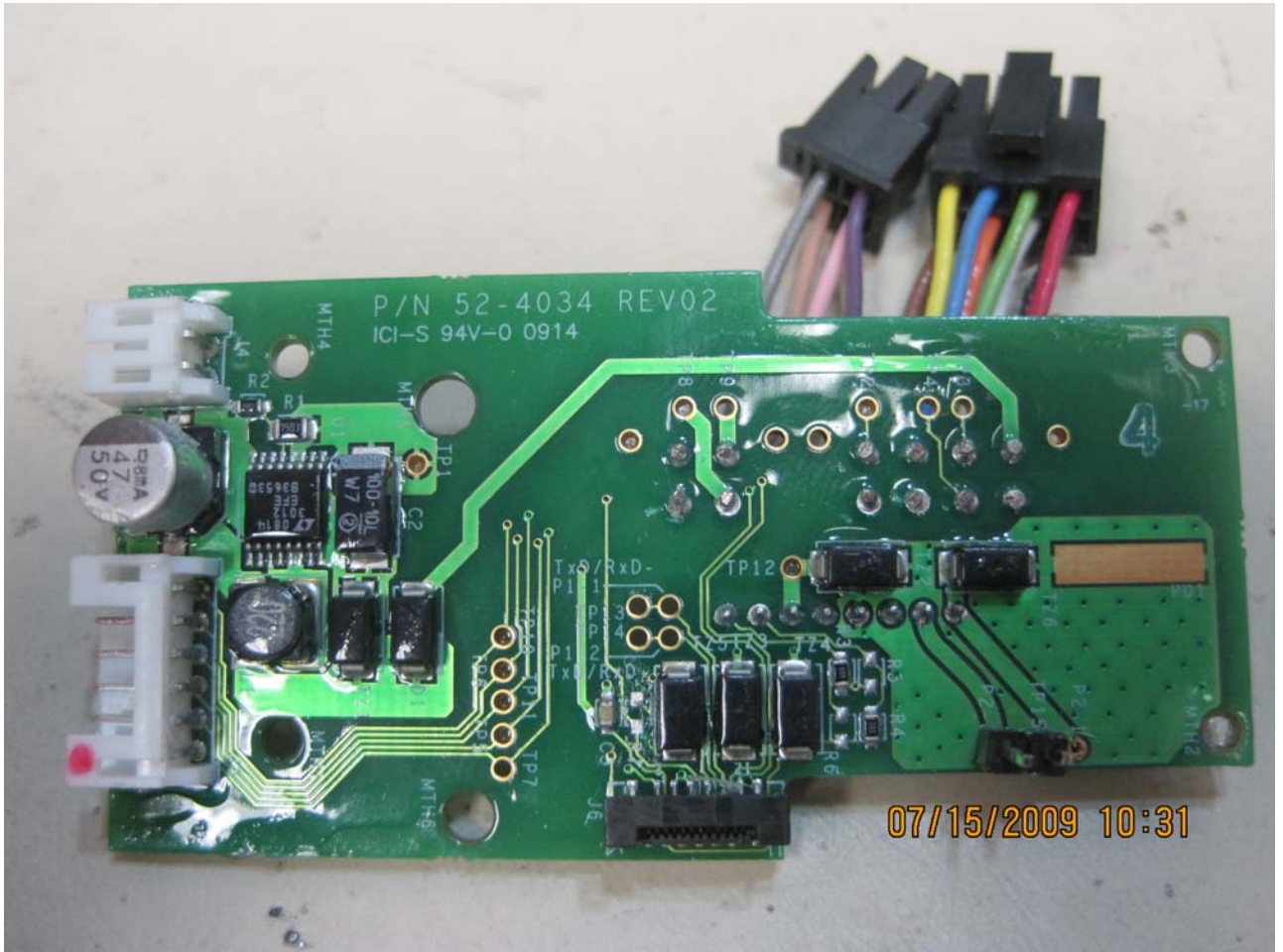
Figure 5: Interface PCB - Front
