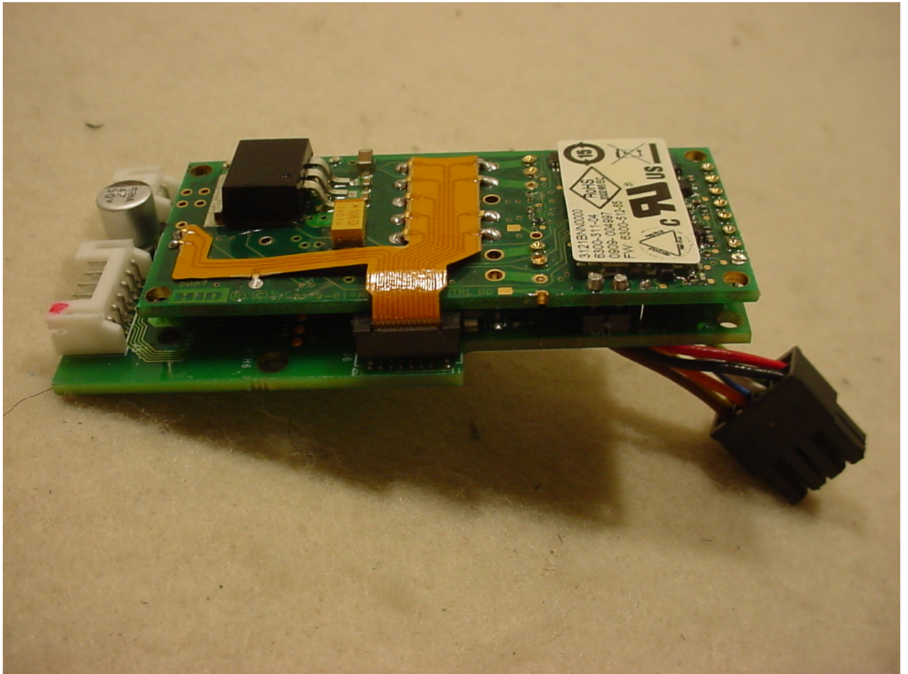
Figure 2: RF and Interface PCB Stackup
