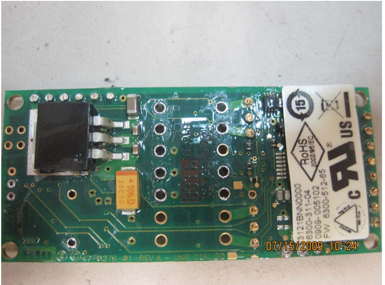
Figure 3: RF PCB - Front
