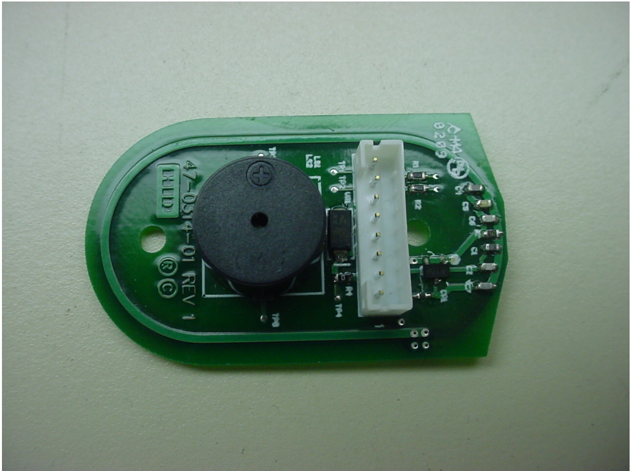
Figure 7: Antenna PCB - Front
