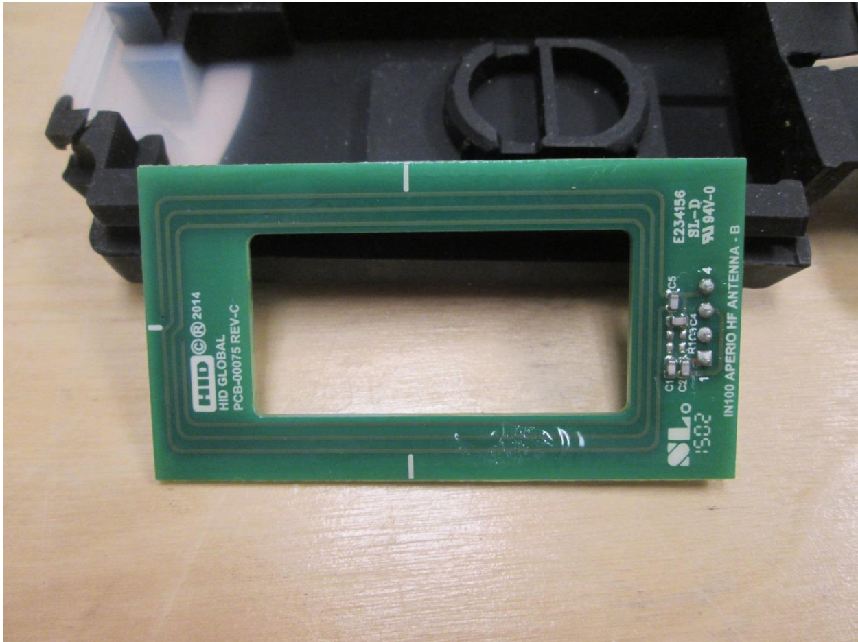
13.56MHz PCB loop antenna
