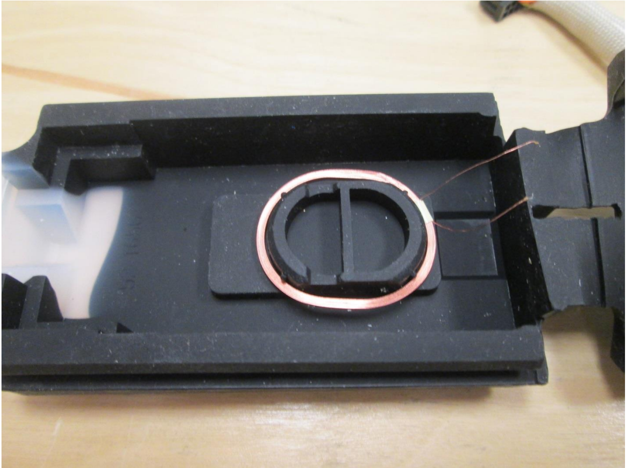
125kHz wire loop antenna
