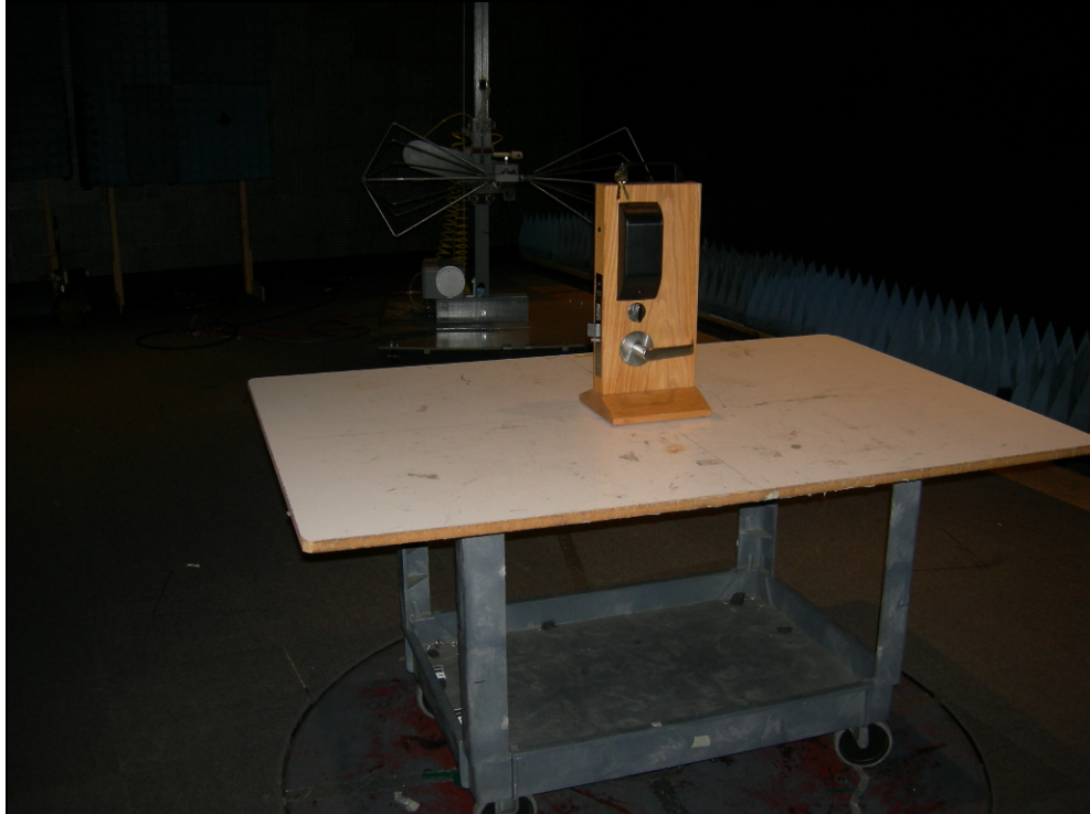
Figure 4: Radiated Emissions
