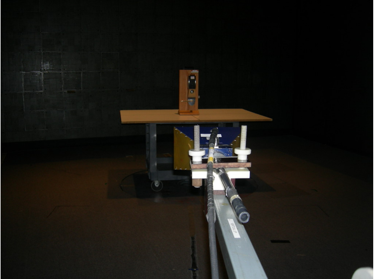
Figure 5: Radiated Emissions
