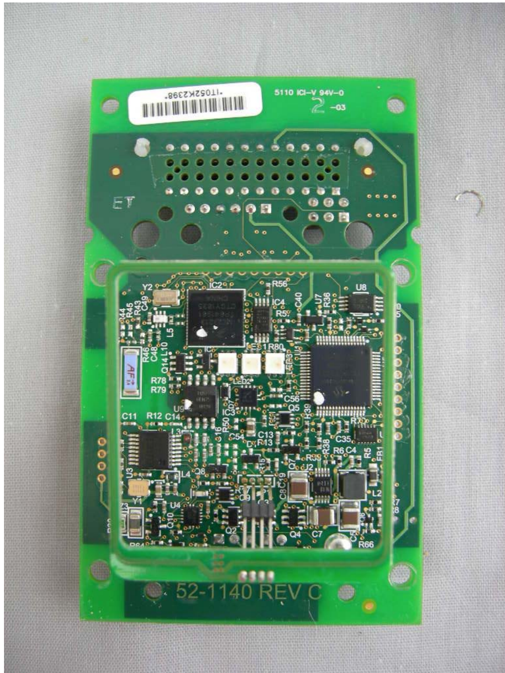
Figure 4: Main Controller PCB Back
