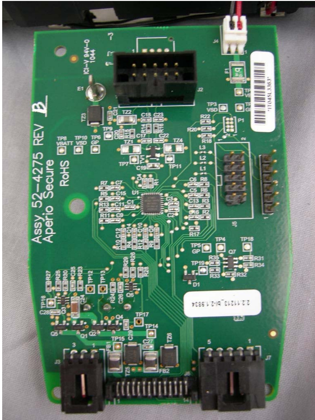
Figure 5: Secure PCB Front
