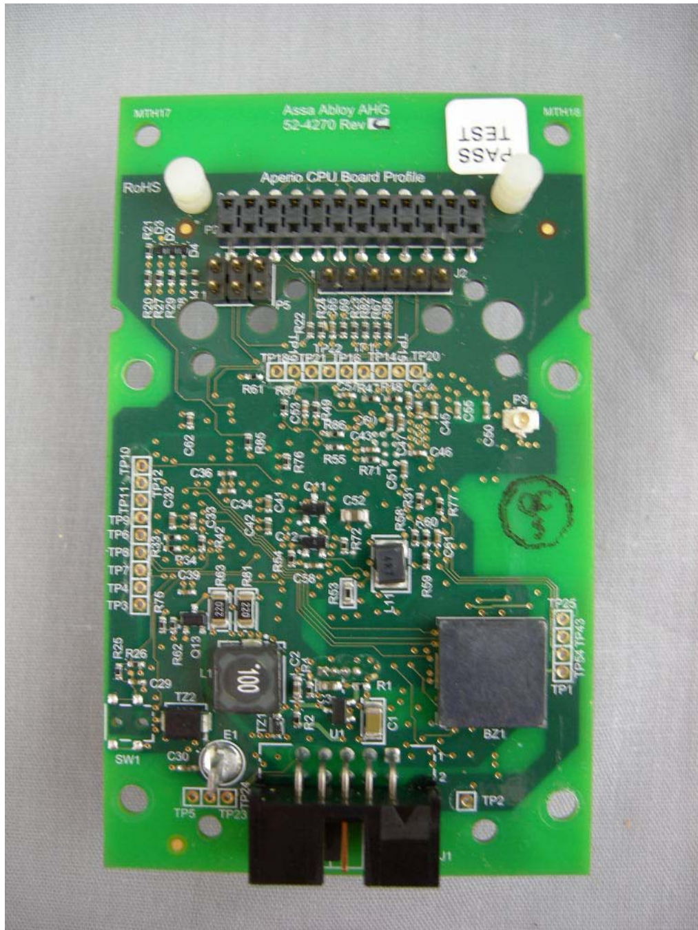
Figure 2: Main Controller PCB Front
