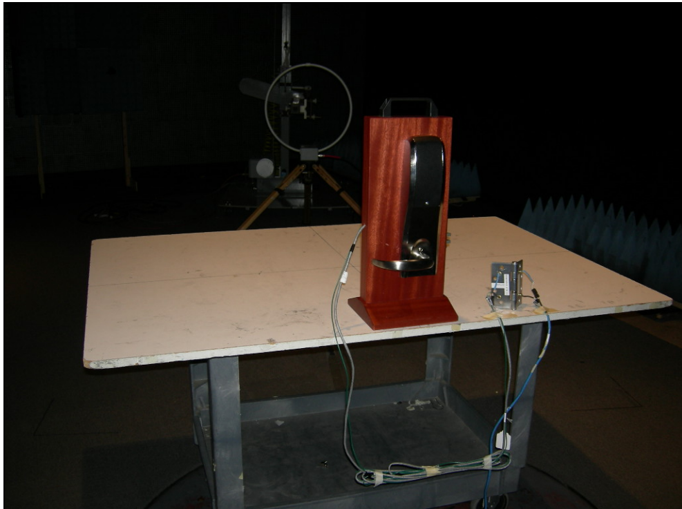
Figure 6: Radiated Emissions - PoE
