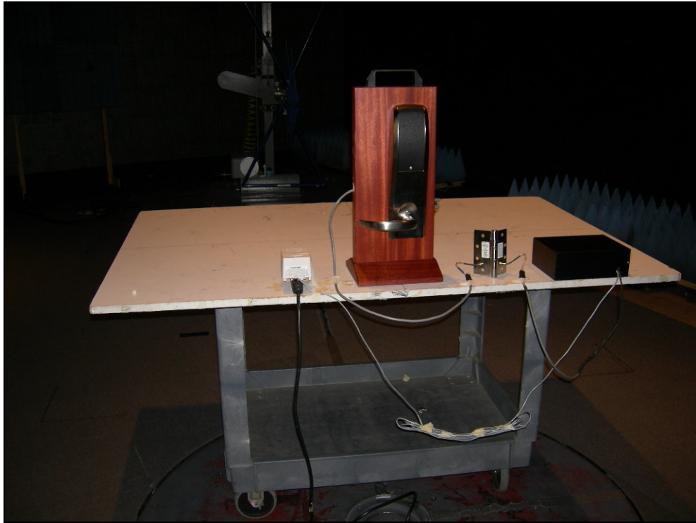
Figure 1: Radiated Emissions - AUX Power
