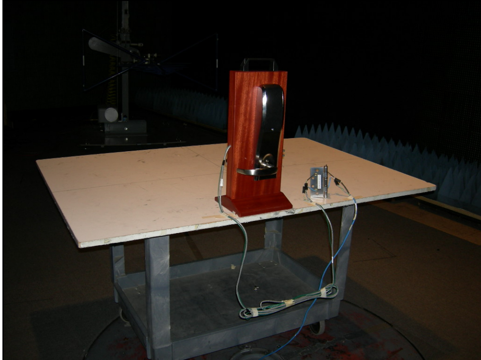
Figure 5: Radiated Emissions - PoE
