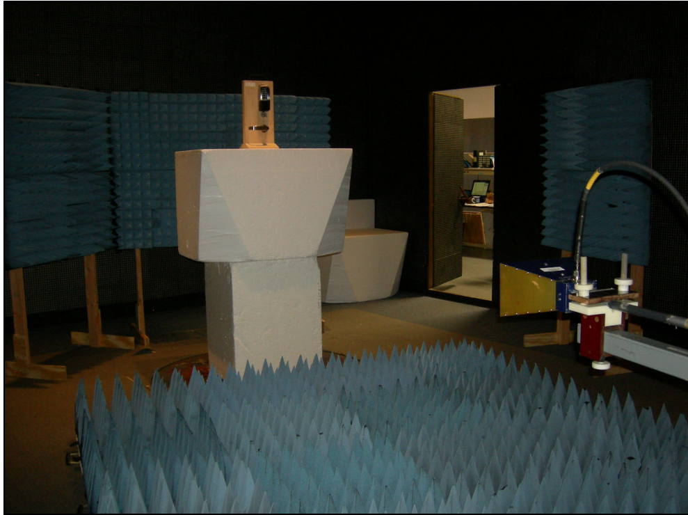
Figure 3: Radiated Emissions – ACCESS700 PWI1-BIMPSK\C ML20700 Battery Powered
