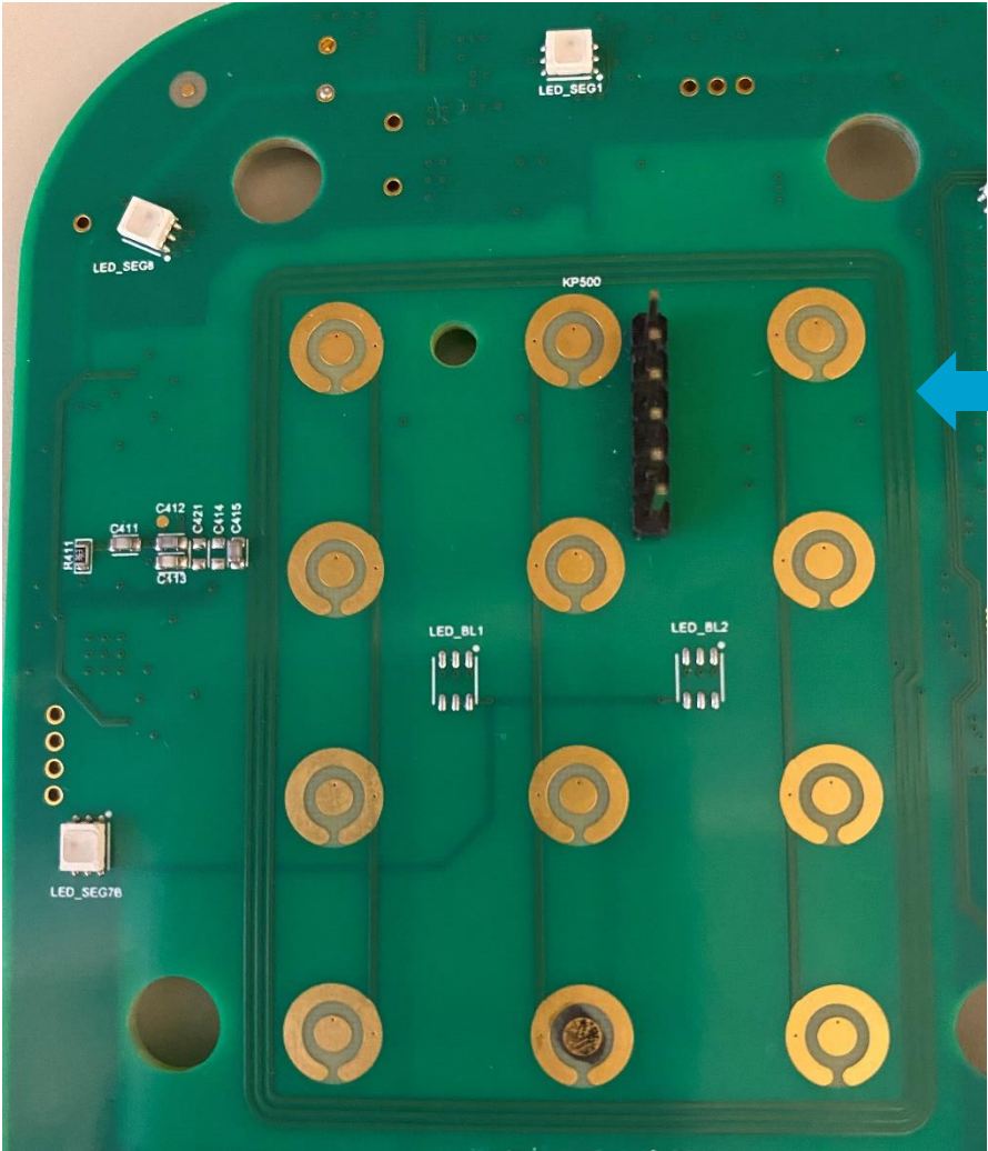
RFID 3 Loop Trace Antenna
