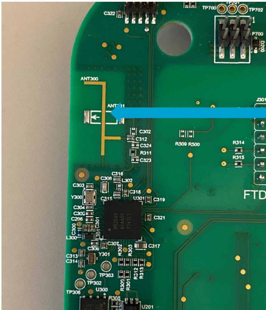
BLE/ZigBee Trace Antenna
