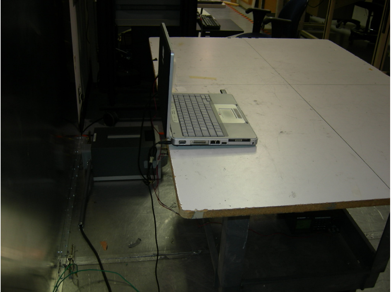
Figure 8: Conducted Emissions
