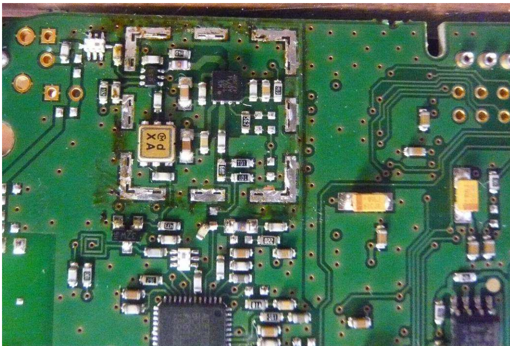
RF shielding can removed
