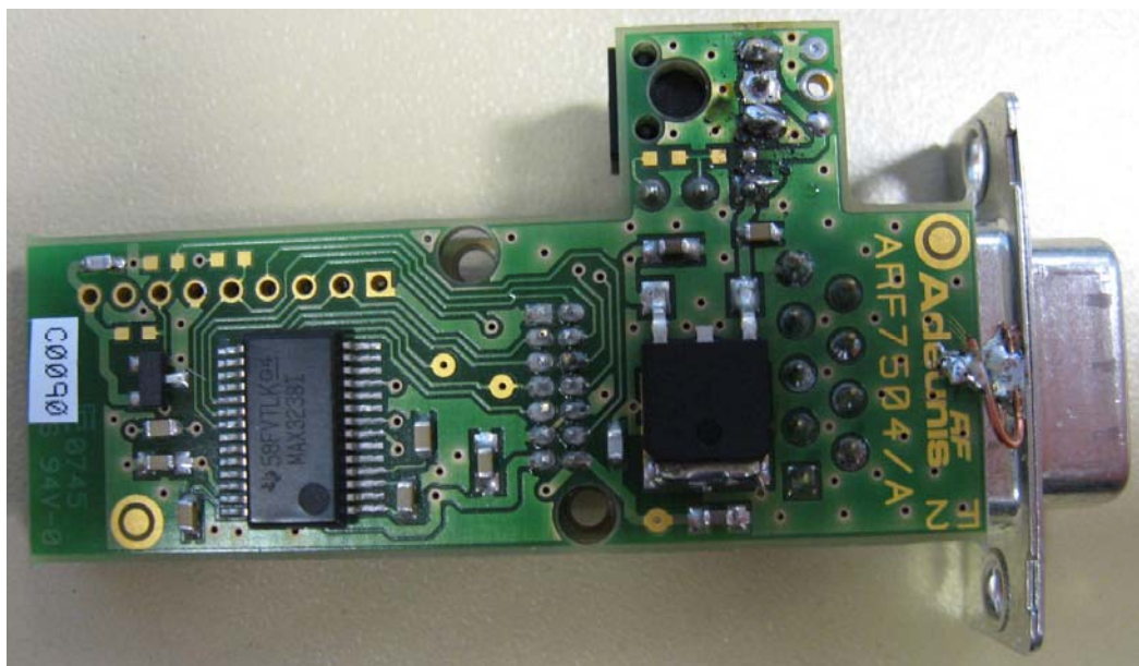
Rear board view
