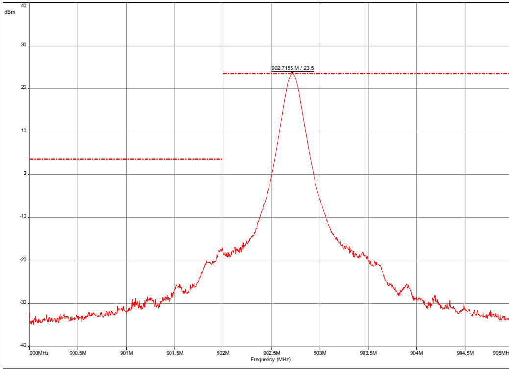
Band Edge CH0 (902.75MHz) - 07/04/2012 09:44 - 960
