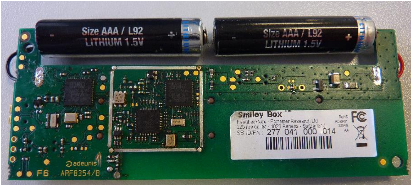
Figure 3: 8354B-Back without shielding
