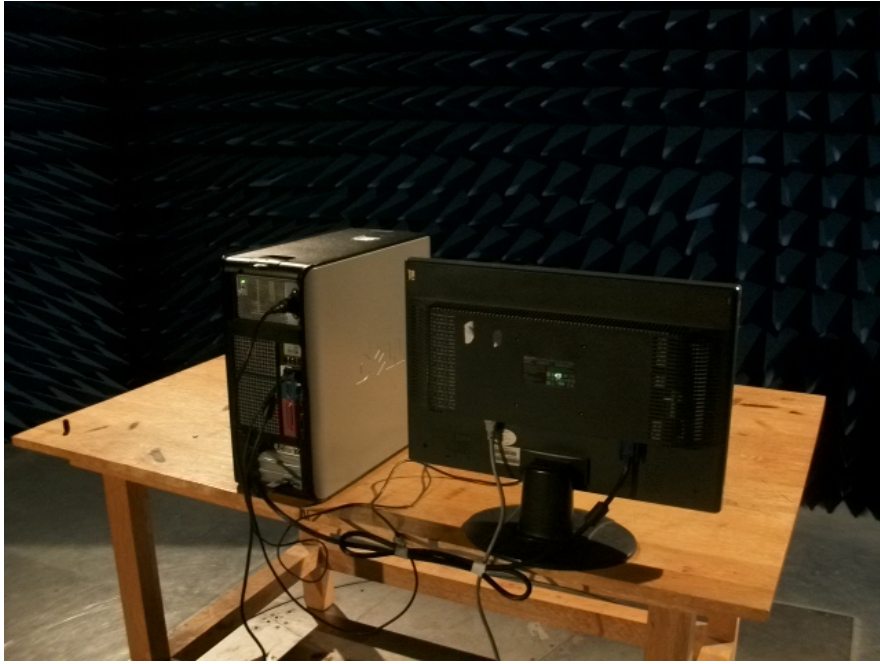
Test photo of radiated emission
