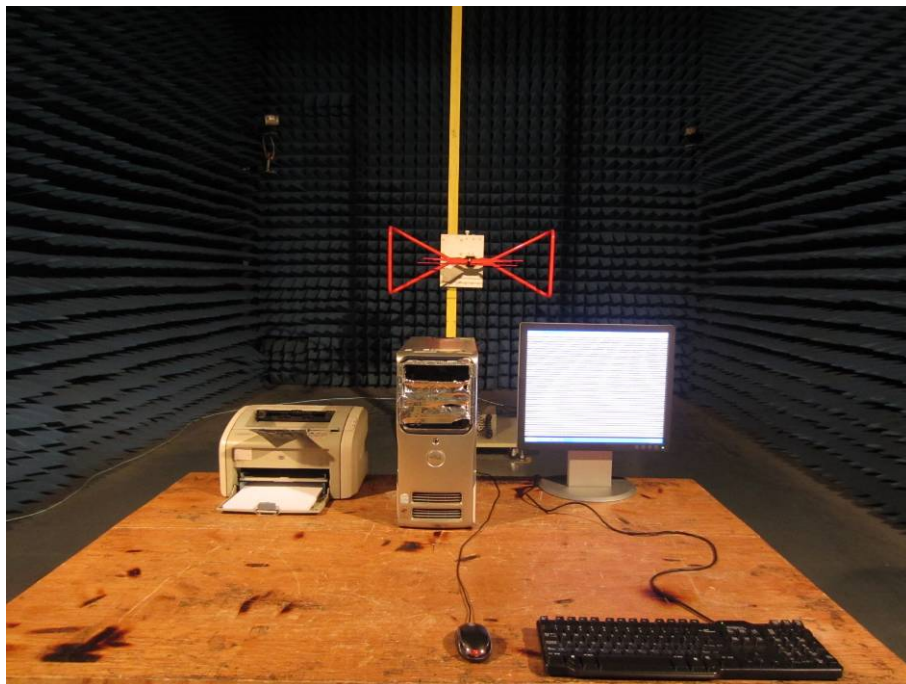
RE TEST SETUP OF ENW02B-3
