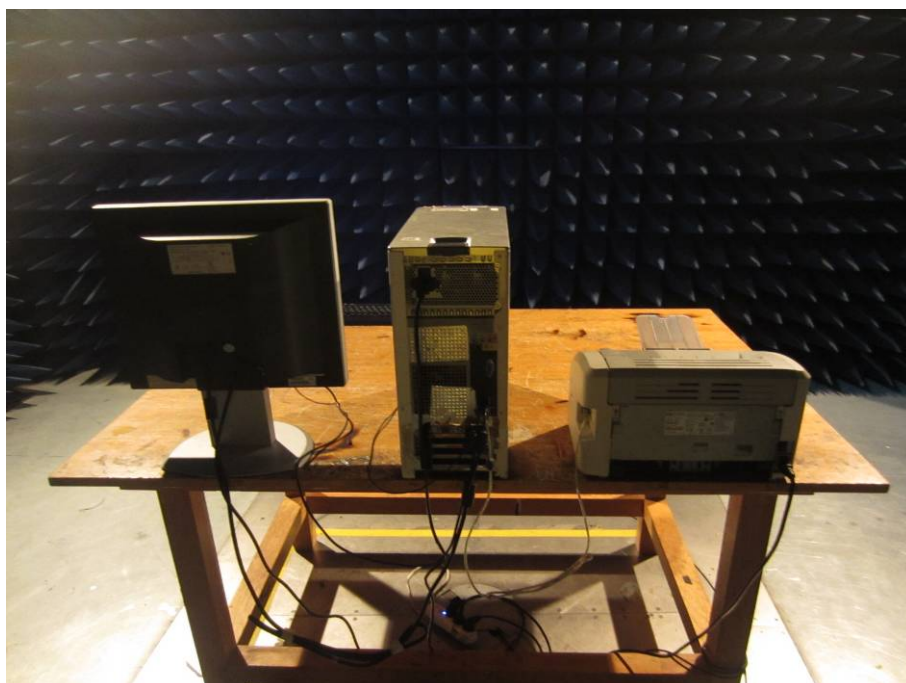
RE TEST SETUP OF ENW02B-4
