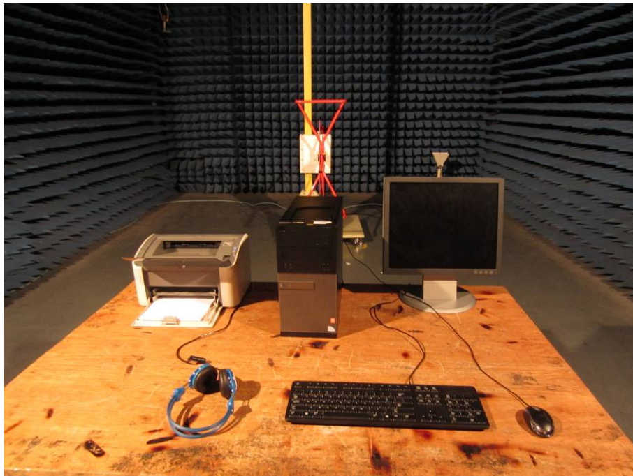
RE TEST SETUP OF EAU02A-3
