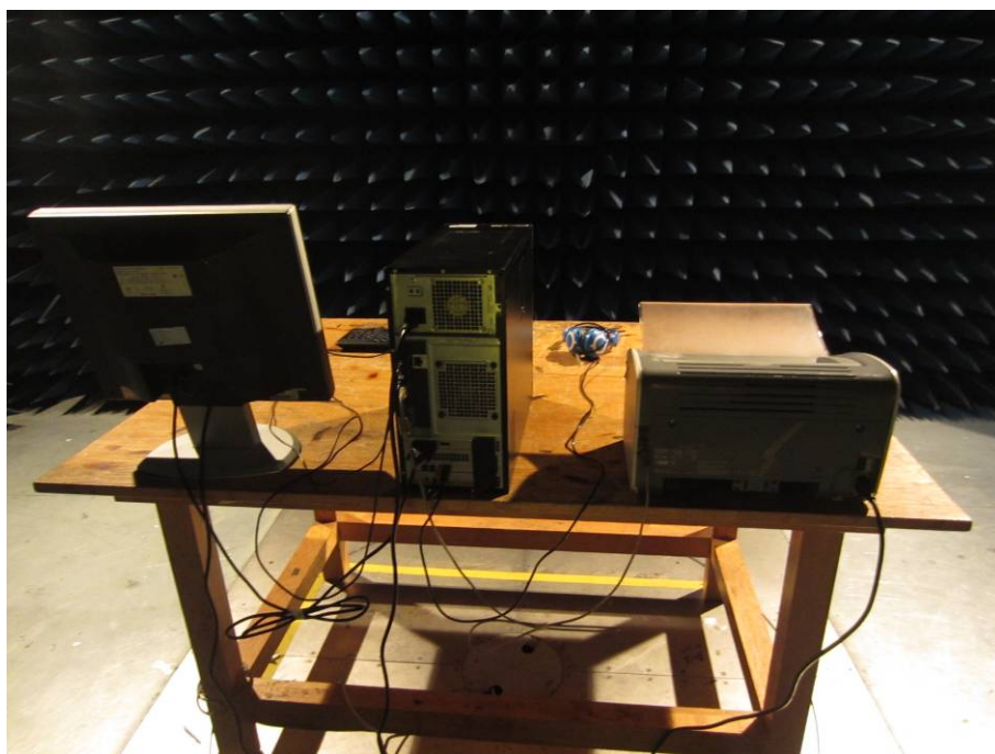
RE TEST SETUP OF EAU02A-4
