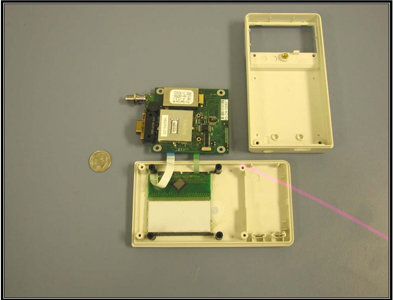
Photograph 8: EUT Unassembled
