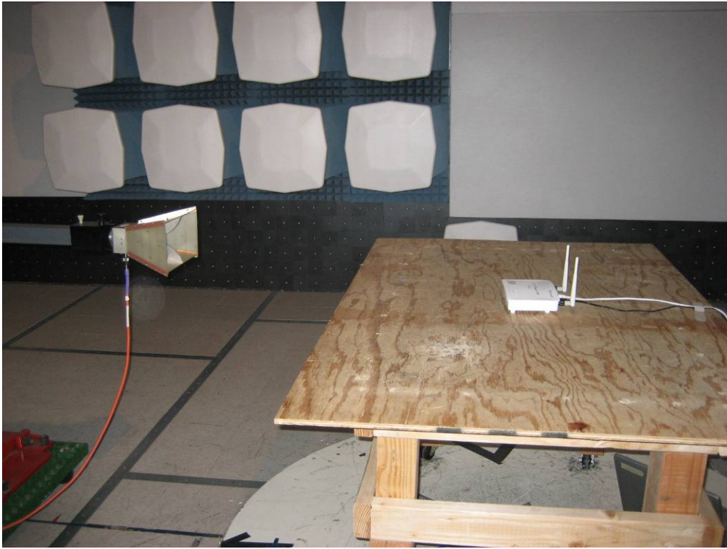
Radiated Emission setup > 1 GHz
