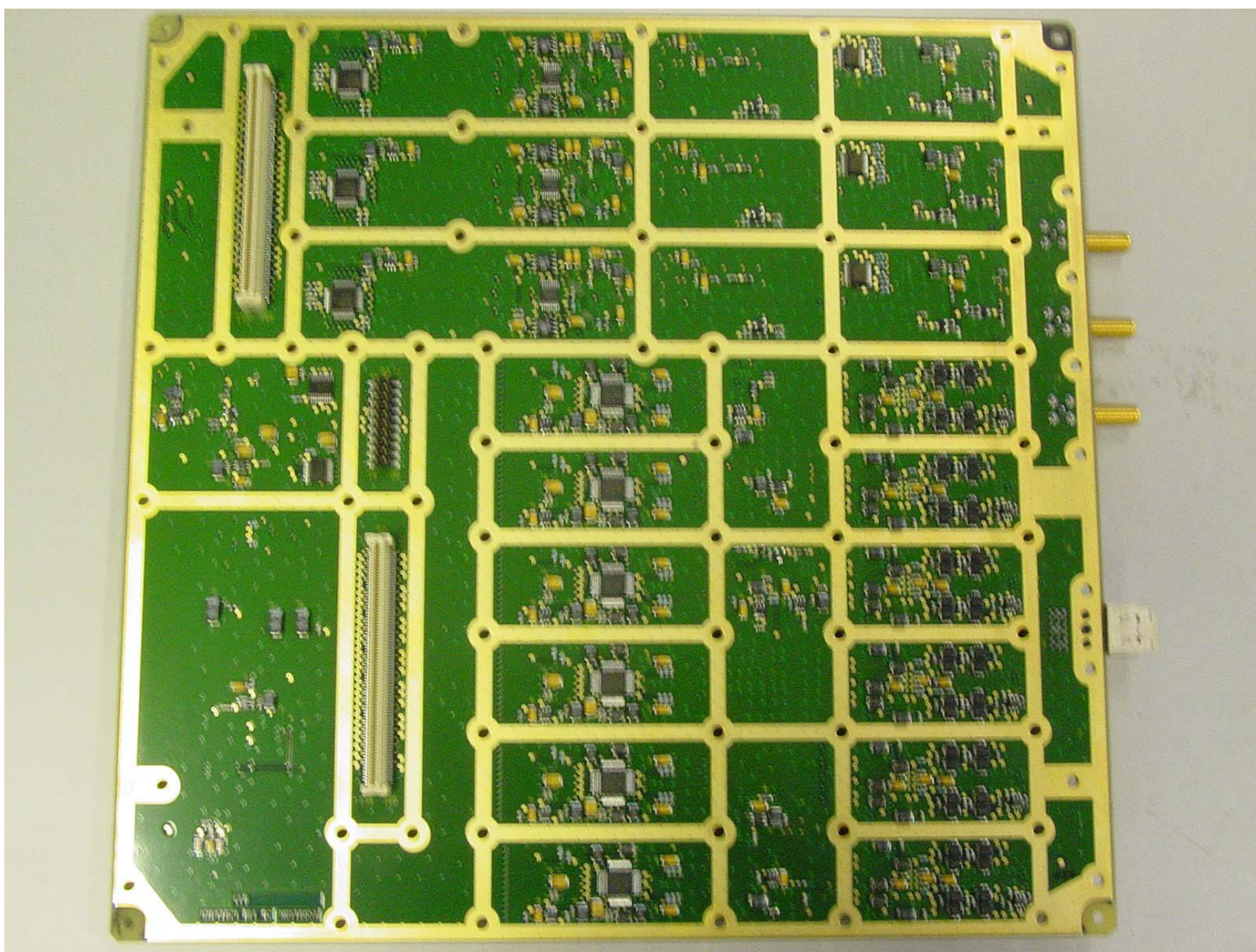
xTRM Radio Board (Bottom)
