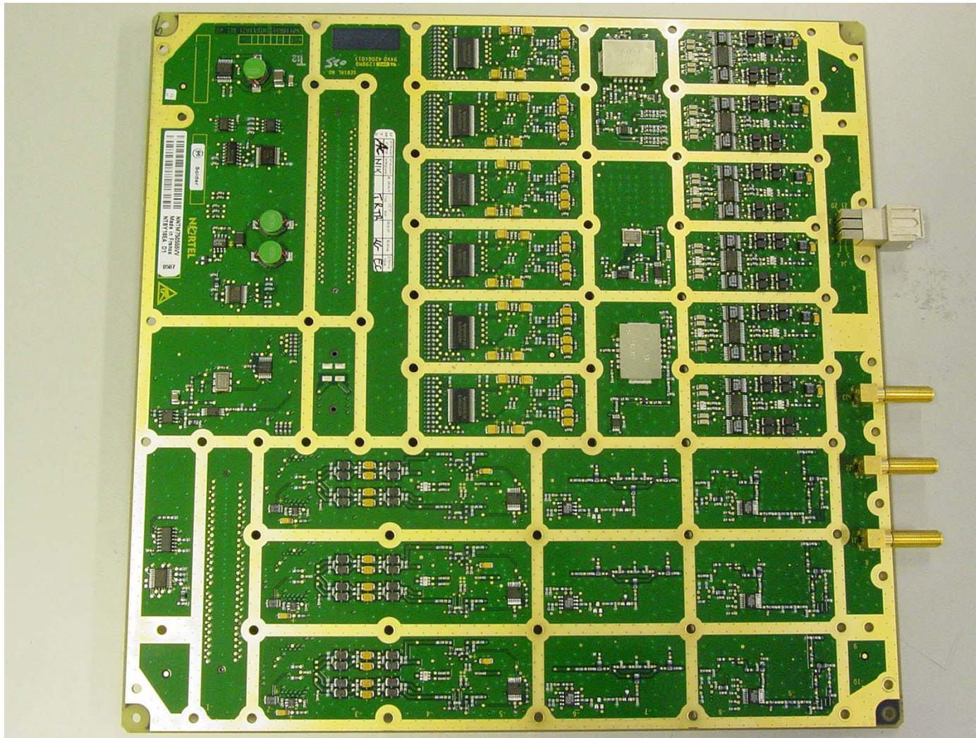
xTRM Radio Board (Top)
