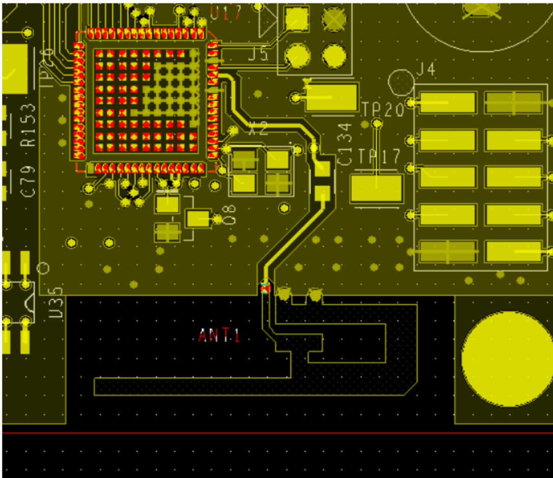
Fig 1. RF circuitry layout showing with ground plan in layout design.
