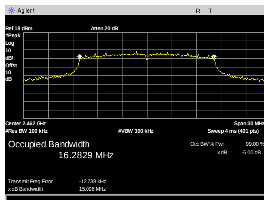
Figure 11: 6dB Occupied Bandwidth, G mode 20M Bw high channel
