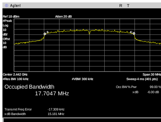
Figure 13: 6dB Occupied Bandwidth, N mode 20M Bw mid channel
