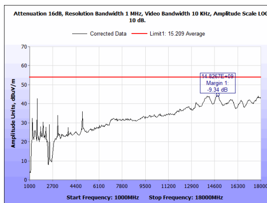
Figure 56: Radiated Spurious Emissions, G mode 20M mid channel RE 1-18GHz Average.
