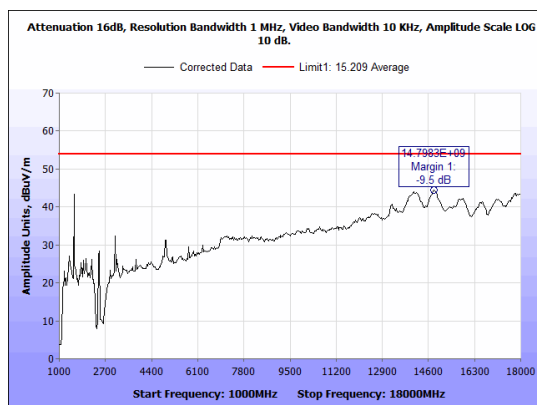
Figure 60: Radiated Spurious Emissions, N mode 20M high channel RE 1-18GHz Average.
