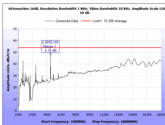
Figure 38: Radiated Spurious Emissions, B mode 20M low channel RE 1-18GHz Average.
