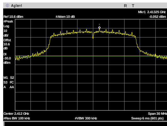
Figure 104: Conducted Spurious Emissions, G mode 20M Bw, AVGSA-2 low channel Reference Level
