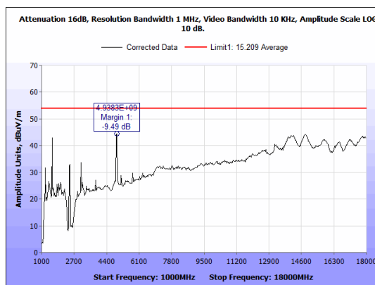
Figure 36: Radiated Spurious Emissions, B mode 20M high channel RE 1-18GHz Average.
