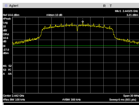
Figure 106: Conducted Spurious Emissions, G mode 20M Bw, AVGSA-2 mid channel Reference Level
