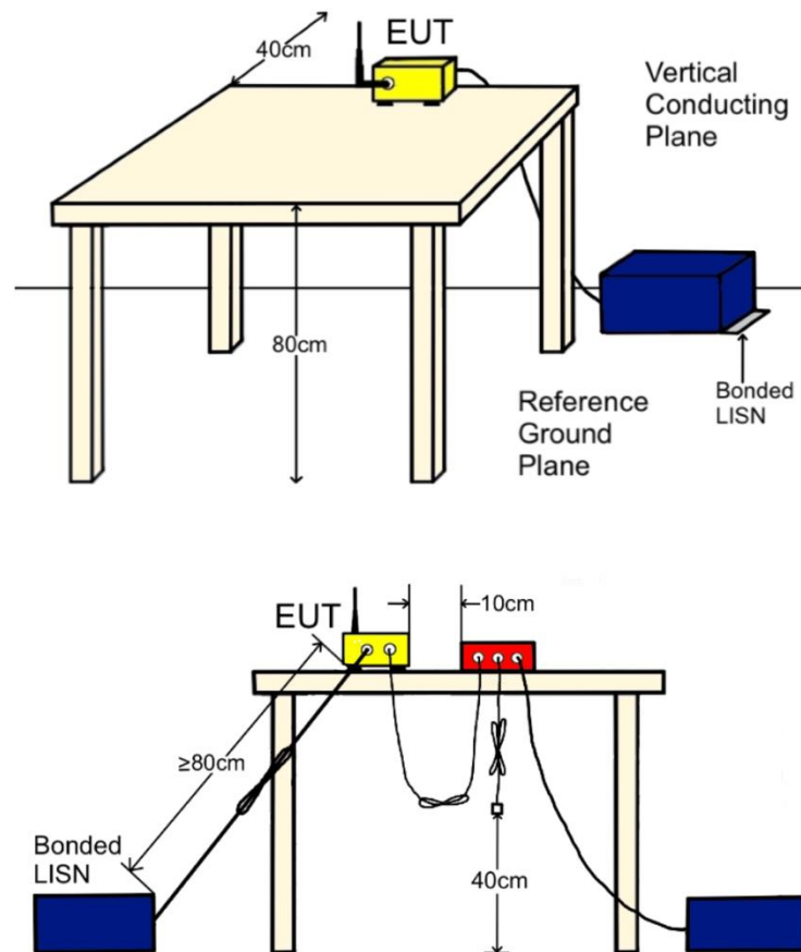
Figure 4. Conducted Emissions, 15.207(a), Test Setup
