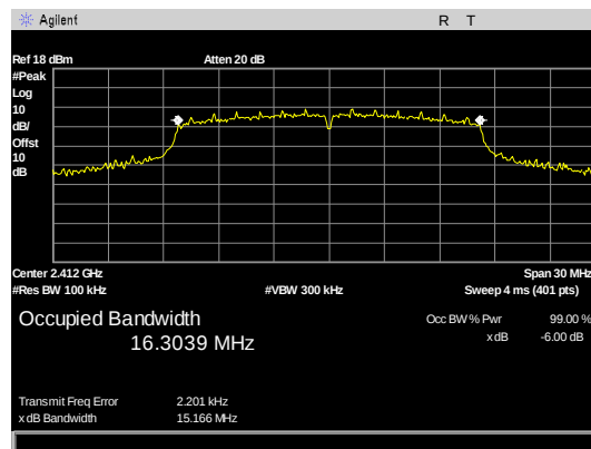
Figure 9: 6dB Occupied Bandwidth, G mode 20M Bw low channel
