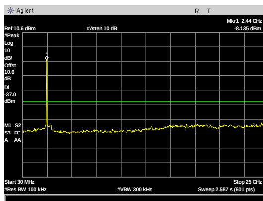
Figure 118: Conducted Spurious Emissions, N mode 40M Bw 30MHz-25GHz, AVGSA-2 high channel
