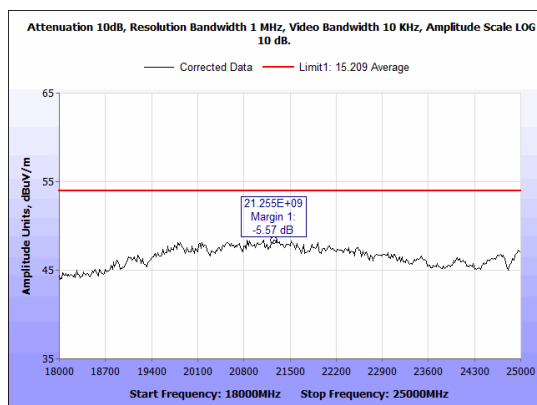
Figure 61: Radiated Spurious Emissions, N mode 20M high channel RE 18-25GHz Average.
