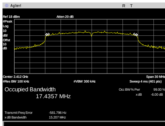
Figure 12: 6dB Occupied Bandwidth, N mode 20M Bw low channel
