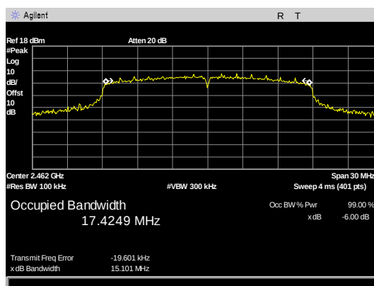
Figure 14: 6dB Occupied Bandwidth, N mode 20M Bw high channel
