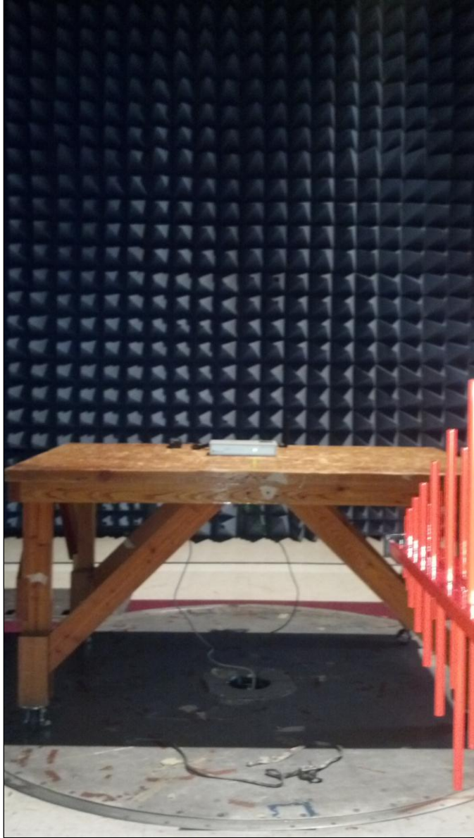
Photograph 2. Radiated Emission, Test Setup, 30 MHz – 1 GHz
