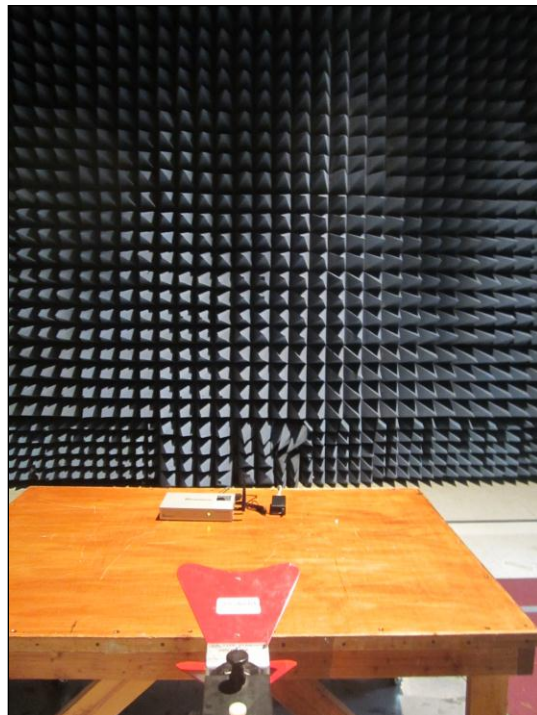
Photograph 6. Radiated Spurious Emissions, Test Setup, 1 GHz – 18 GHz
