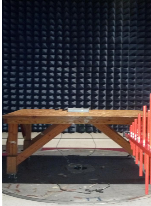
Photograph 5. Radiated Spurious Emissions, Test Setup, 30 MHz – 1 GHz
