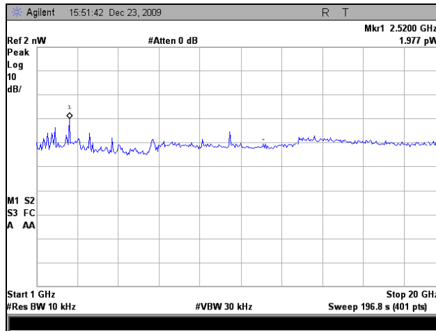
Plot 76. Conducted Receiver Spurious Emissions, Port 2, 1 GHz – 20 GHz
