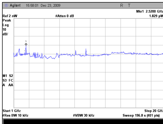
Plot 78. Conducted Receiver Spurious Emissions, Port 3, 1 GHz – 20 GHz
