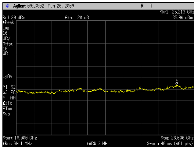
Plot 43. Conducted Spurious Emissions, Low Channel, 10 MHz (18 GHz – 26 GHz)
