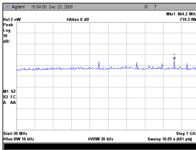
Plot 77. Conducted Receiver Spurious Emissions, Port 3, 30 MHz – 1 GHz
