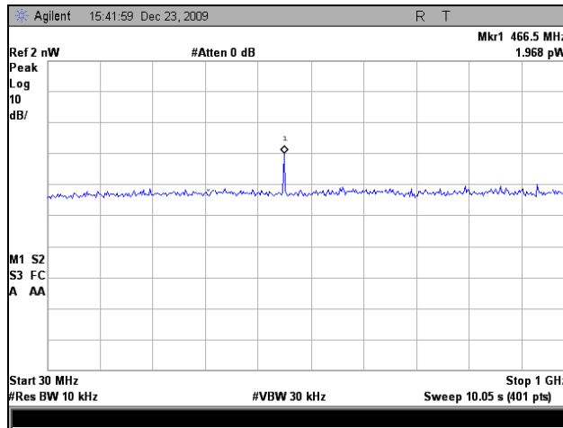
Plot 73. Conducted Receiver Spurious Emissions, Port 1, 30 MHz – 1 GHz
