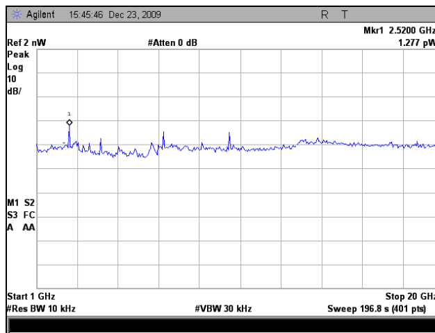
Plot 74. Conducted Receiver Spurious Emissions, Port 1, 1 GHz – 20 GHz
