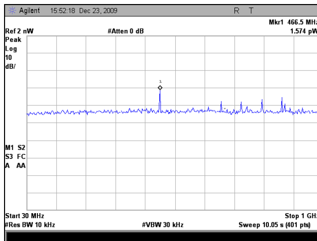
Plot 75. Conducted Receiver Spurious Emissions, Port 2, 30 MHz – 1 GHz
