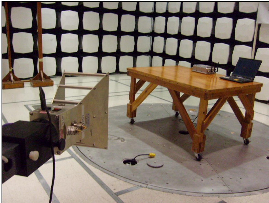
Photograph 3. Radiated Emission Test Setup 1 GHz – 6 GHz
