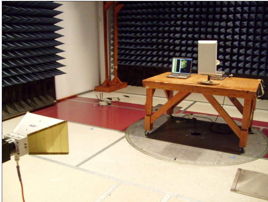
Photograph 8. Test Equipment and Setup for Various Radiated Measurements – 16 dBi Sector
