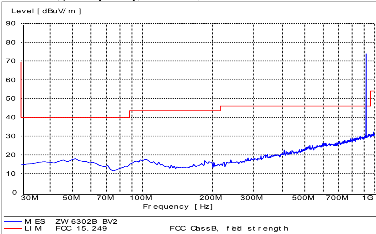
Test mode 2, power by battery, below 1GHz, Vertical
