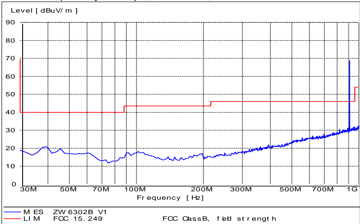
Test mode 1, power by AC adaptor, below 1GHz, Vertical
