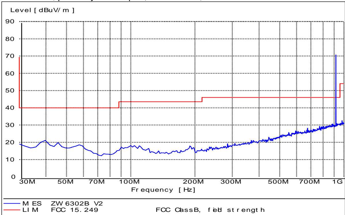
Test mode 2, power by AC adaptor, below 1GHz, Vertical
