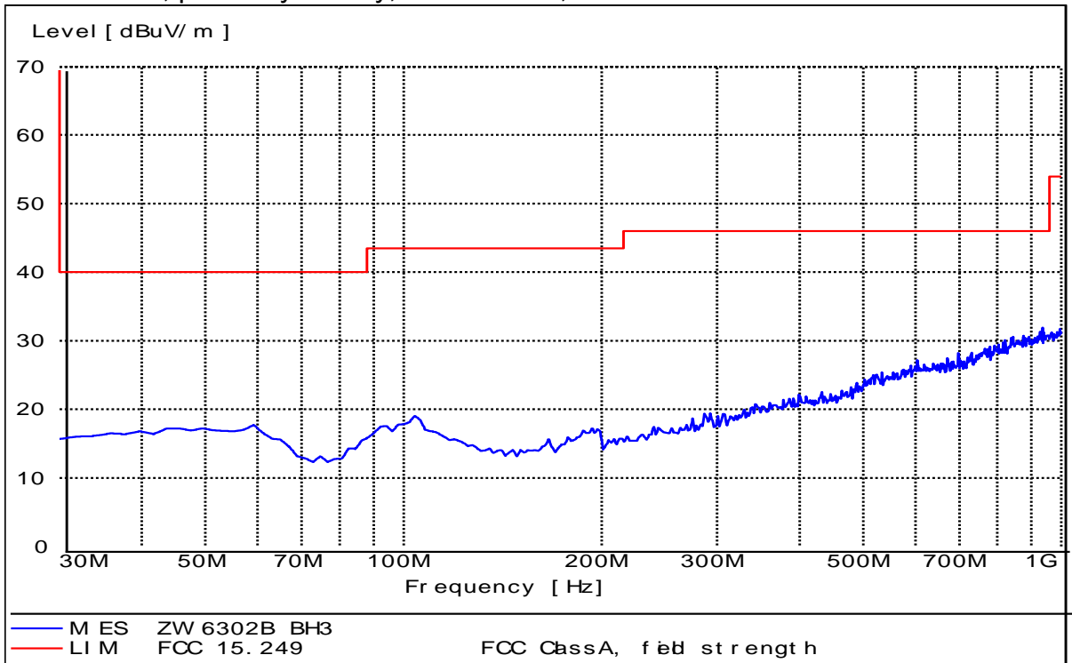
Test mode 3, power by battery, below 1GHz, Horizontal
