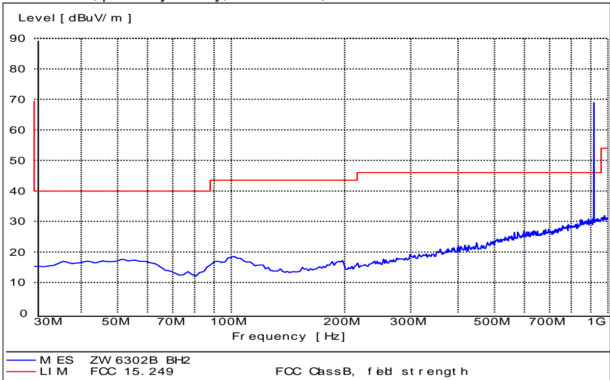
Test mode 2, power by battery, below 1GHz, Horizontal
