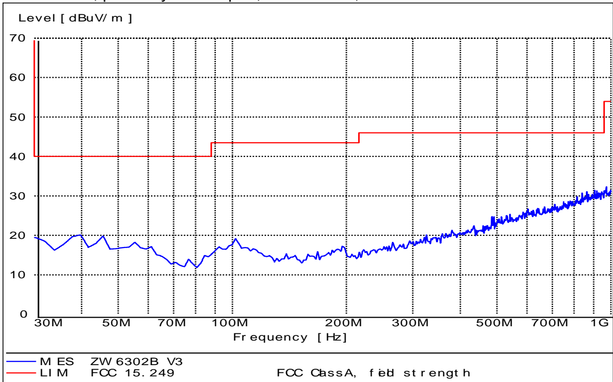
Test mode 3, power by AC adaptor, below 1GHz, Vertical
