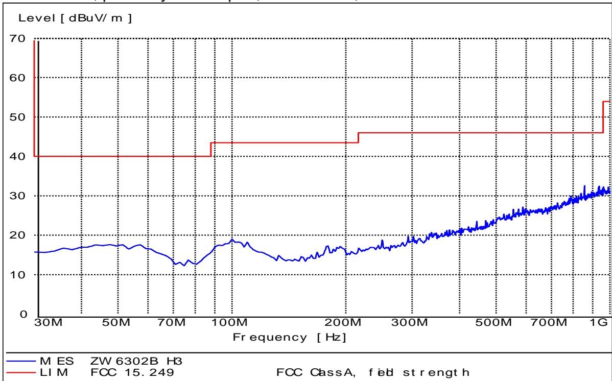
Test mode 3, power by AC adaptor, below 1GHz, Horizontal
