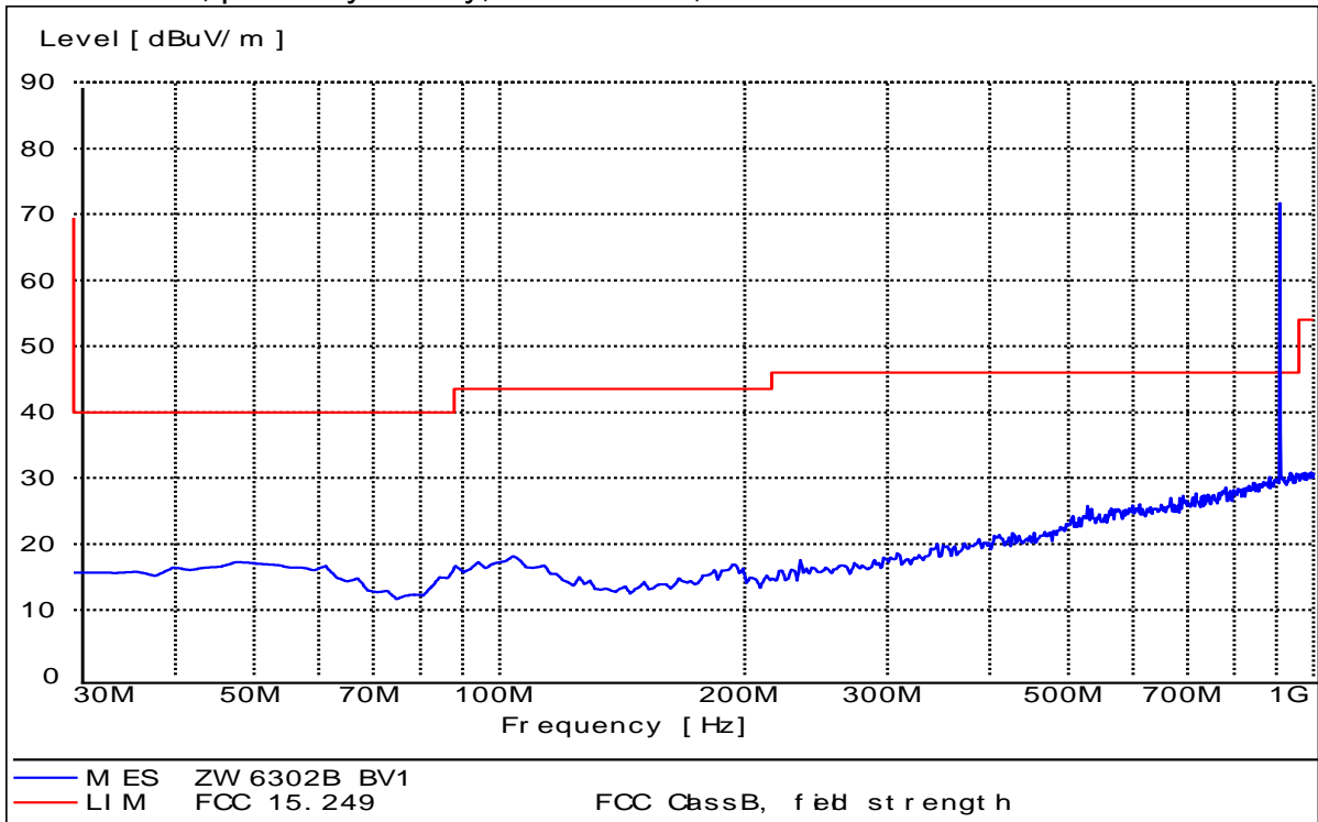
Test mode 1, power by battery, below 1GHz, Vertical
