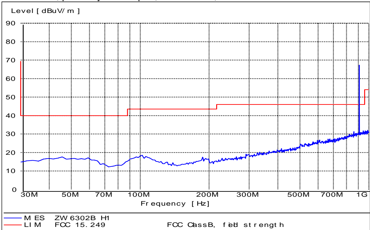
Test mode 1, power by AC adaptor, below 1GHz, Horizontal
