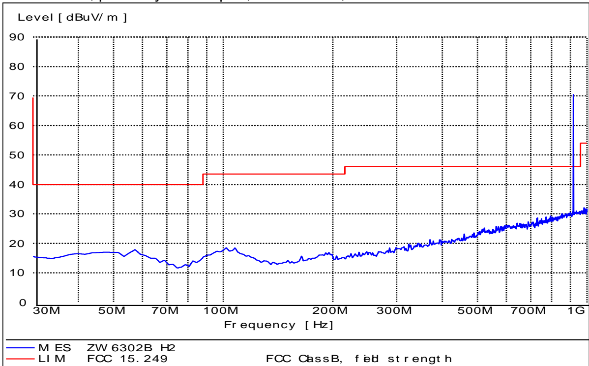
Test mode 2, power by AC adaptor, below 1GHz, Horizontal
