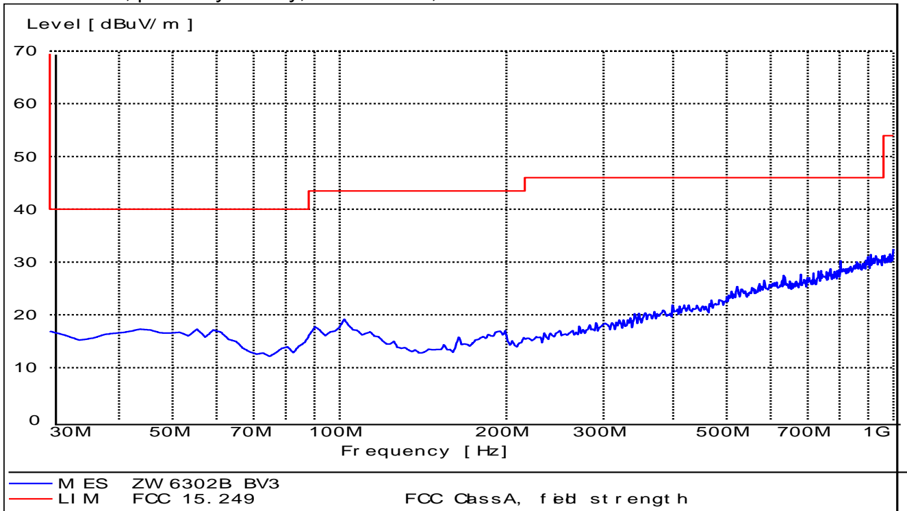
Test mode 3, power by battery, below 1GHz, Vertical
