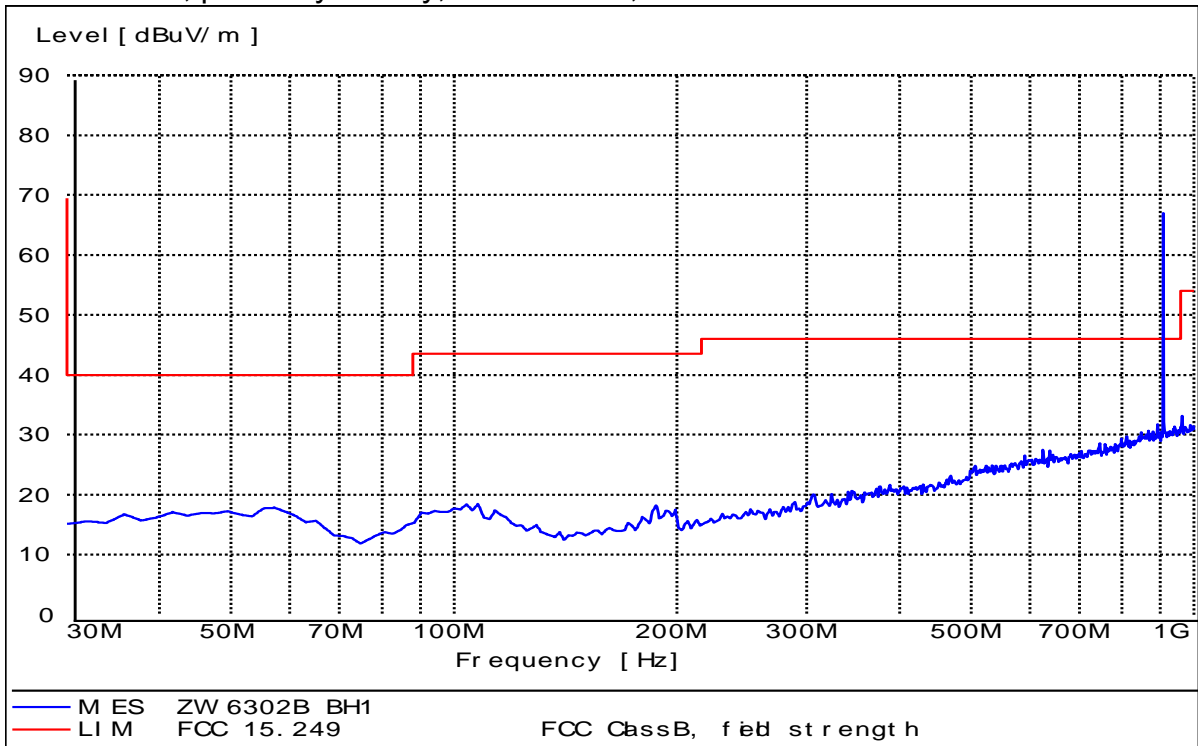
Test mode 1, power by battery, below 1GHz, Horizontal
