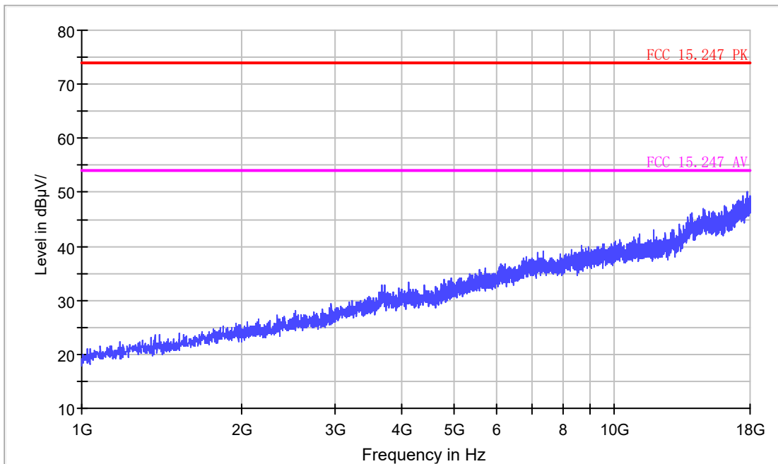
FCC Electric Field Strength 1-18GHz
