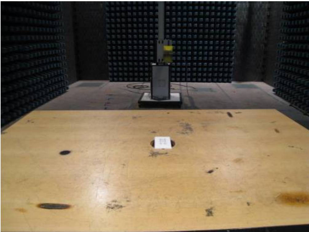
Photo 2 Radiated Disturbance Test
