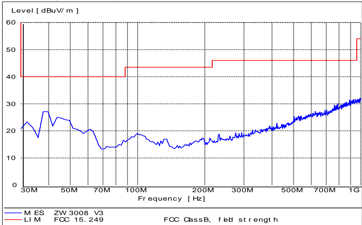
Test mode 3, below 1GHz, Vertical
