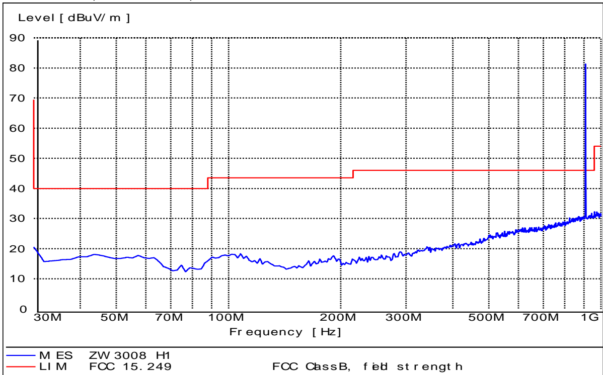
Test mode 1, below 1GHz, Horizontal
