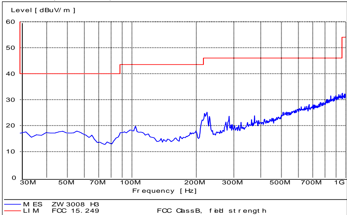
Test mode 3, below 1GHz, Horizontal
