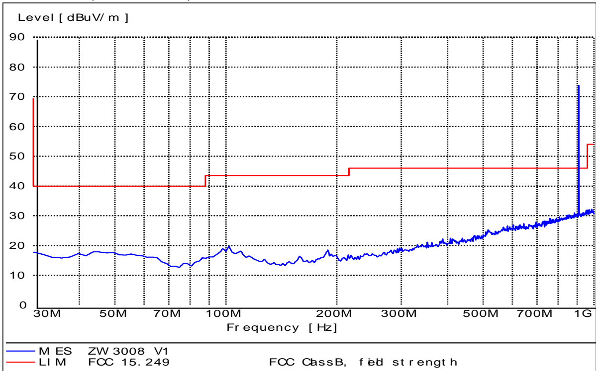
Test mode 1, below 1GHz, Vertical
