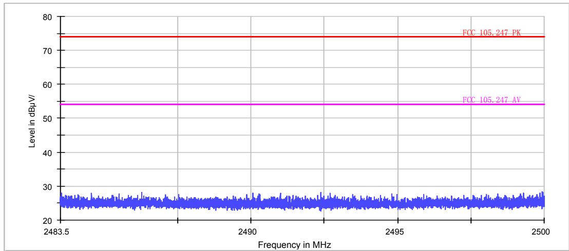
FCC Electric Field Strength 2.4GHz Bandedge-PK
