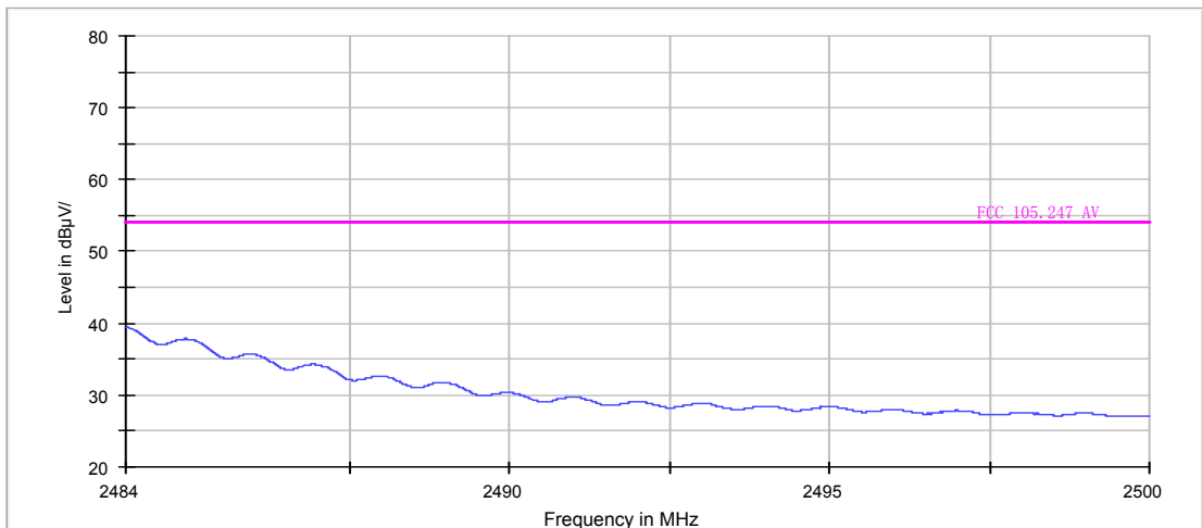
FCC Electric Field Strength 2.4GHz Bandedge-AV
