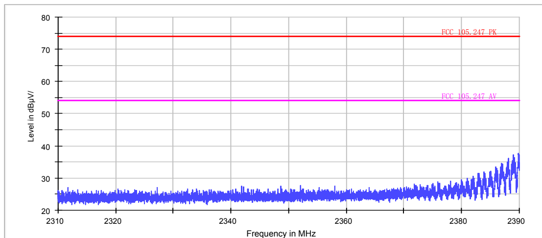
FCC Electric Field Strength 2.4GHz Bandedge-PK
