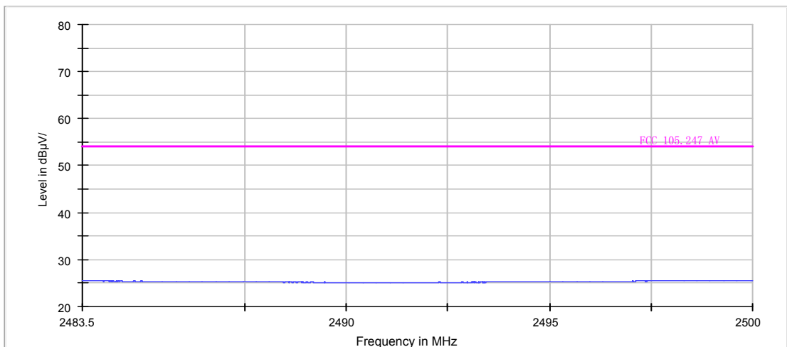
FCC Electric Field Strength 2.4GHz Bandedge-AV
