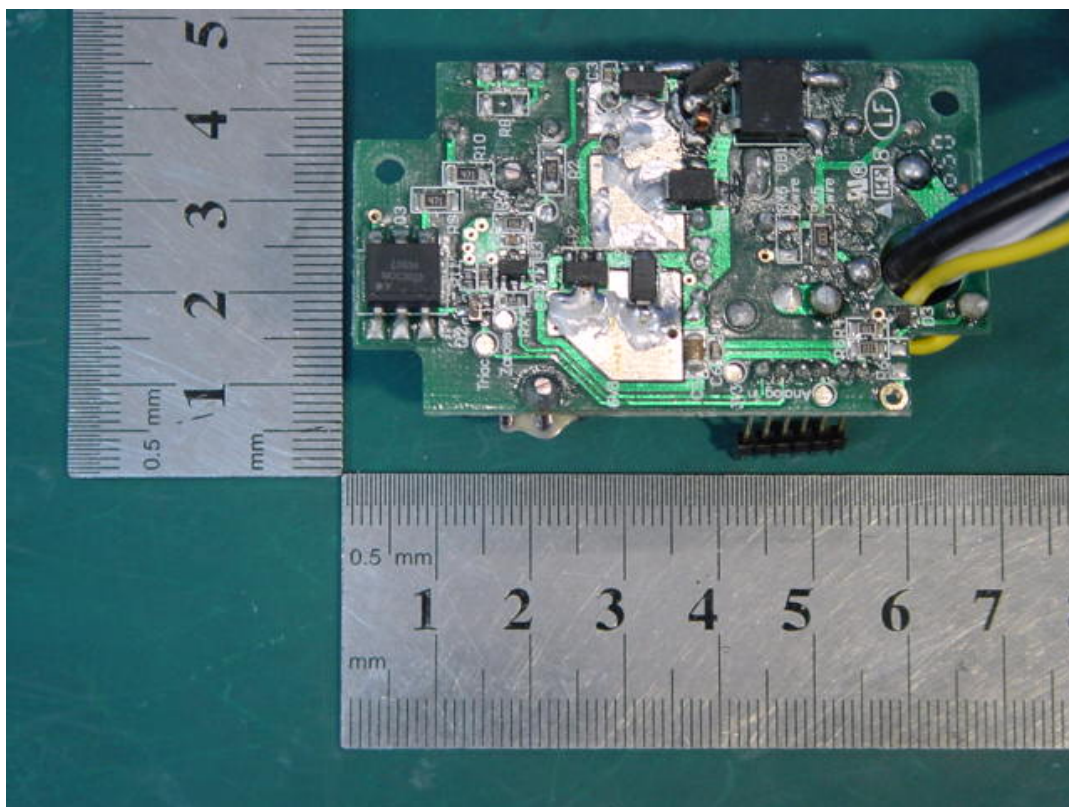
Photo 6 Inside of EUT (45607)
