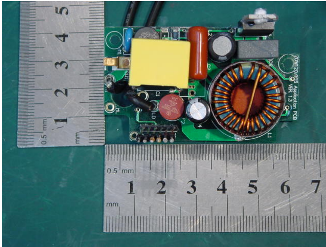
Photo 14 Inside of EUT (45606)
