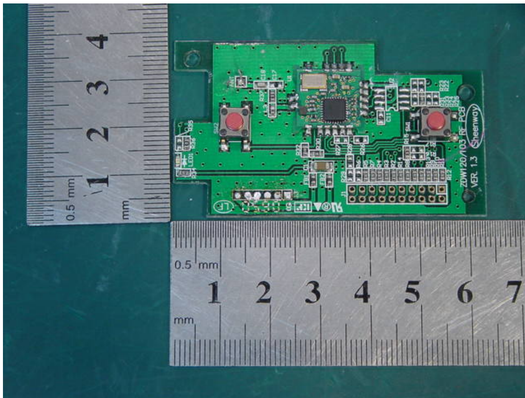
Photo 12 Inside of EUT (45606)
