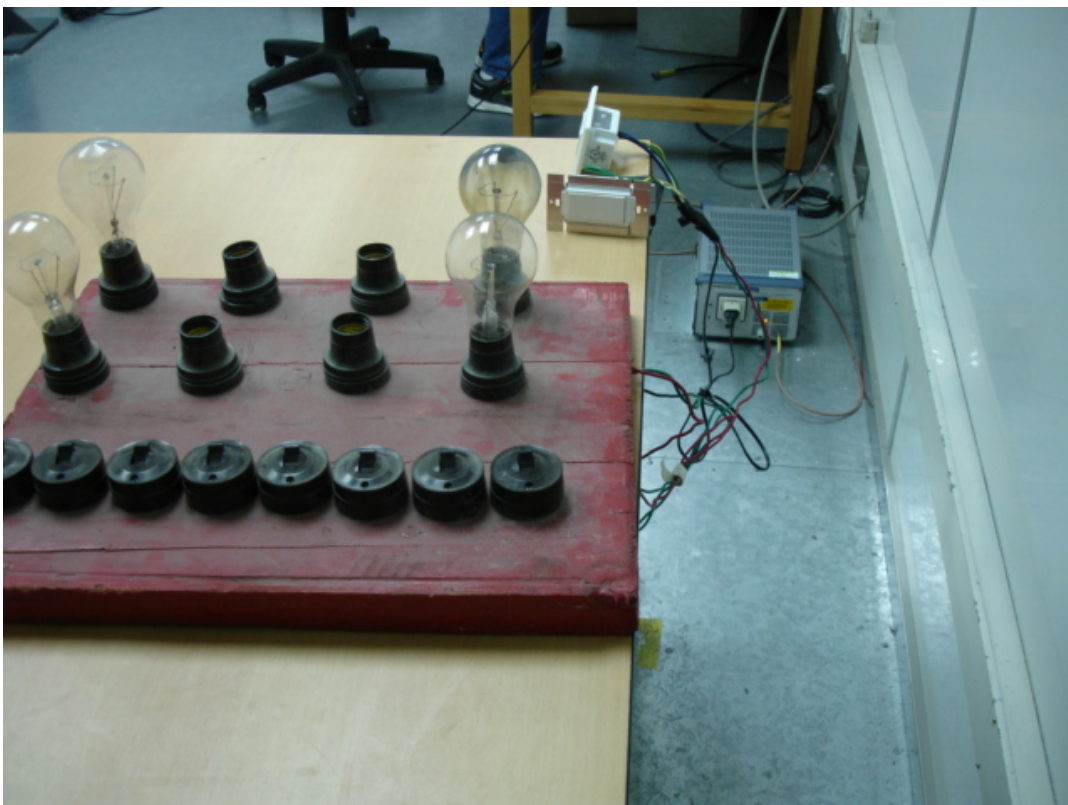
Photo 2 Conducted Emission Test (45607)
