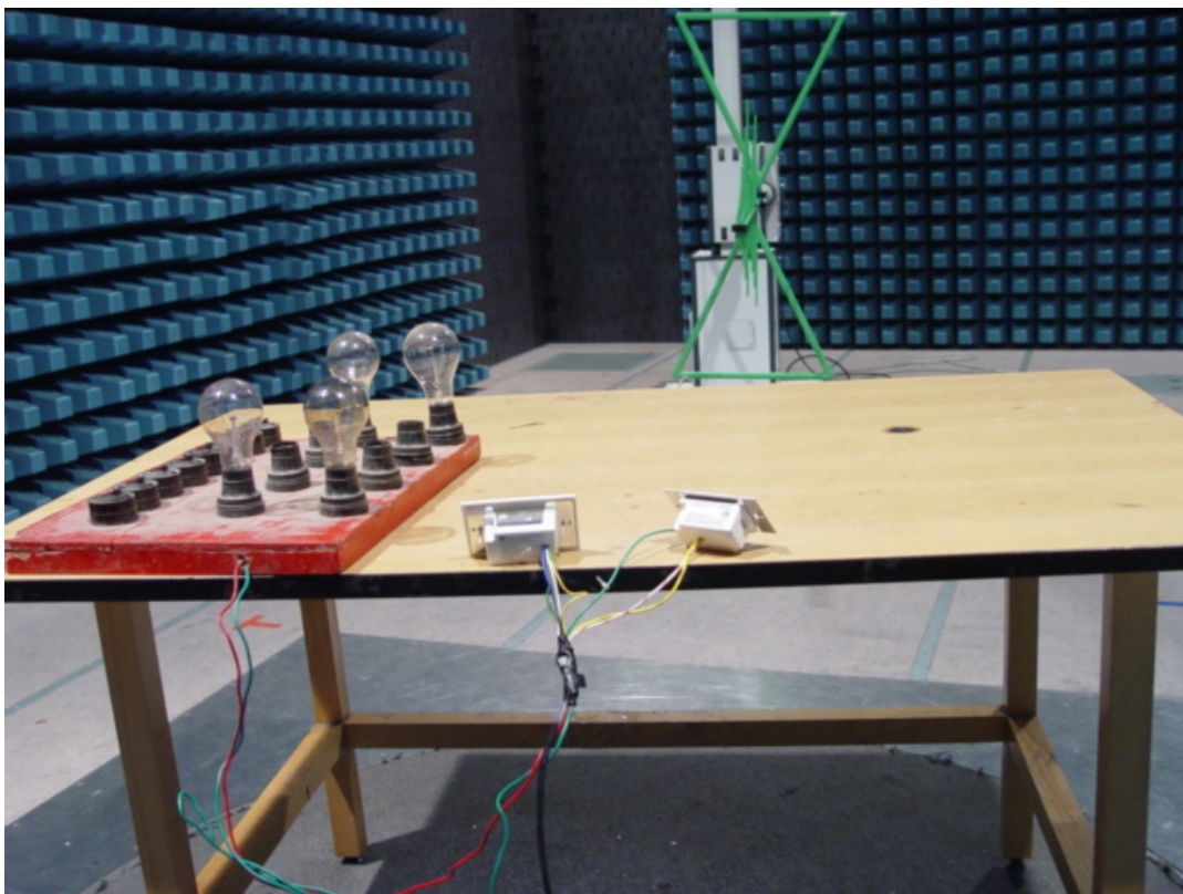
Photo 4 Radiated Emission Test (45607)
