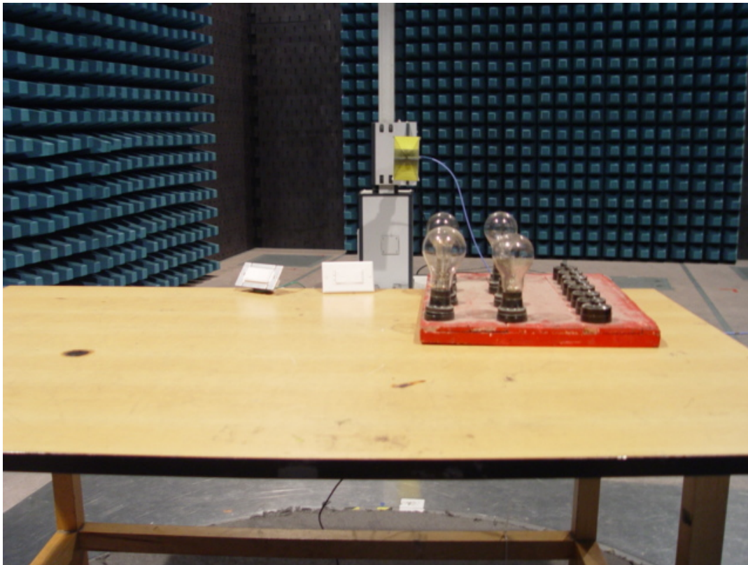
Photo 6 Radiated Emission Test (45607)
