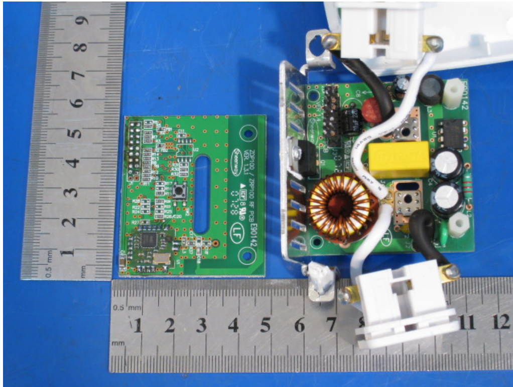
Photo 12 Inside of EUT (45602 Rev2)
