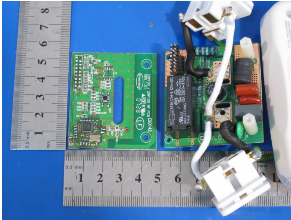
Photo 6 Inside of EUT (45603 Rev2)
