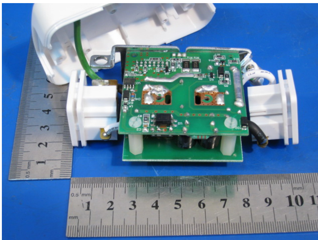
Photo 10 Inside of EUT (45602 Rev2)
