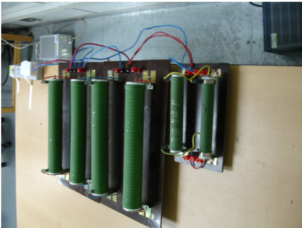
Photo 2 Conducted Emission Test (45603 Rev2)
