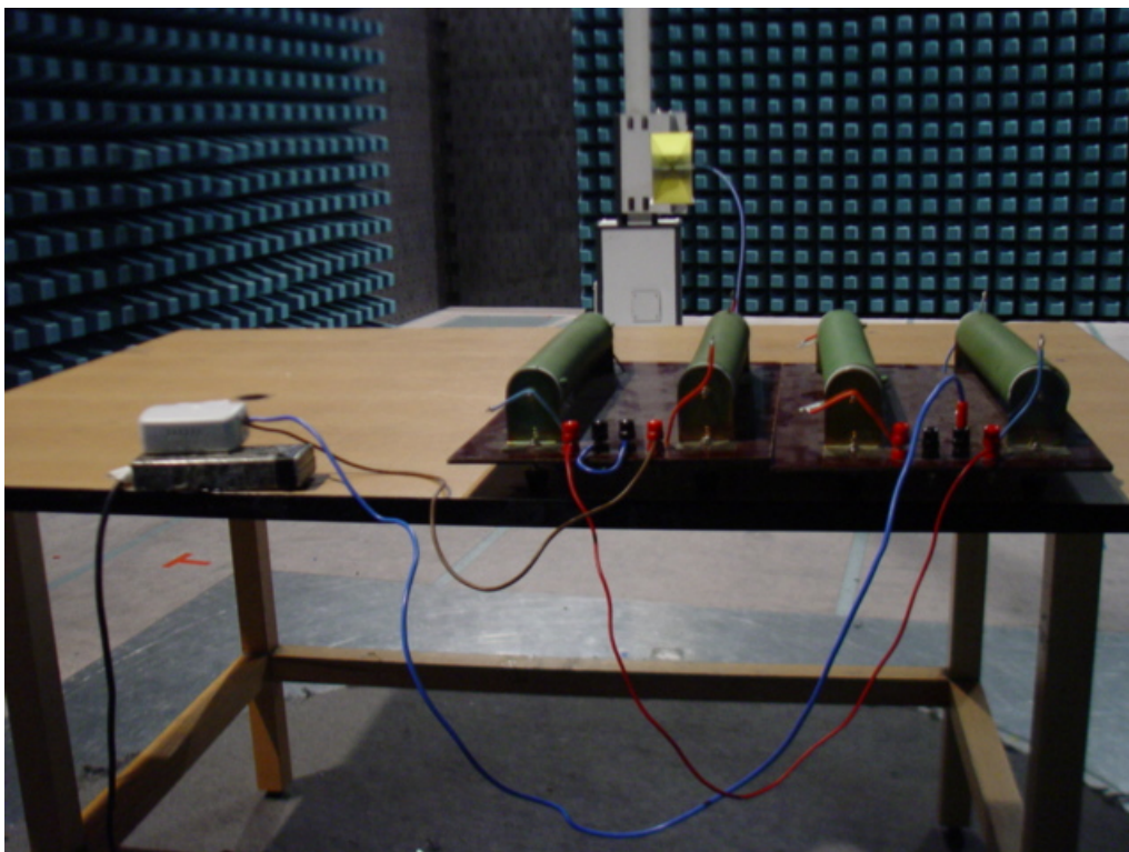
Photo 4 Radiated Emission Test (45603 Rev2)
