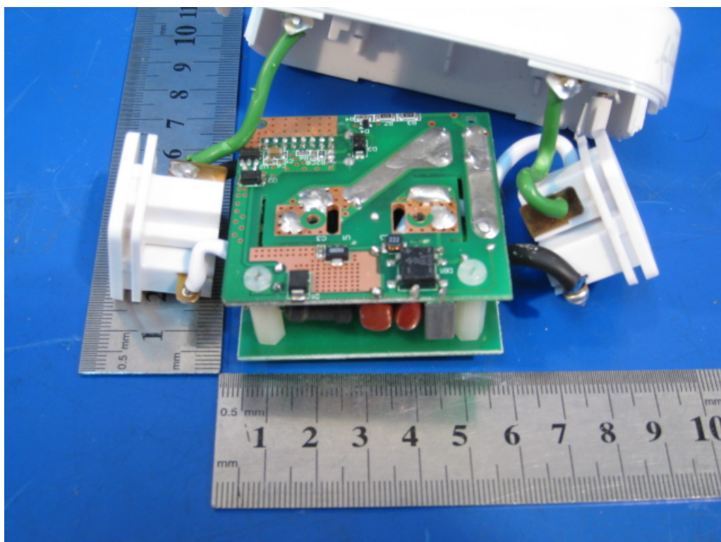
Photo 4 Inside of EUT (45603 Rev2)
