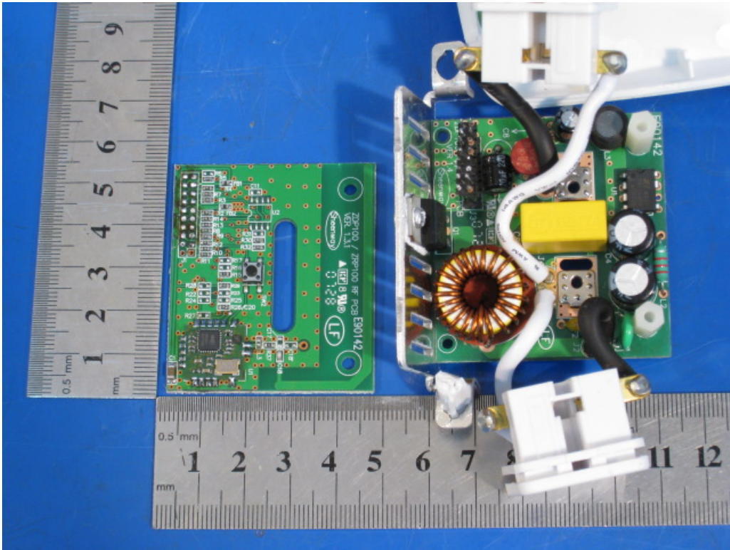
Photo 8 Inside of EUT (45602 Rev2)
