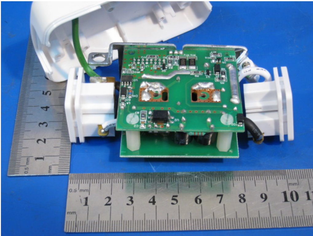
Photo 6 Inside of EUT (45602 Rev2)
