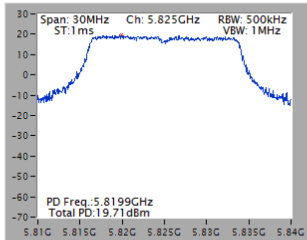
RF Power Spectral Density Plots w/o Duty Factor
