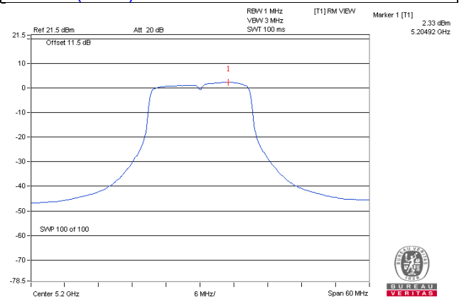
802.11n (HT20) / CH 40 / Chain 1
