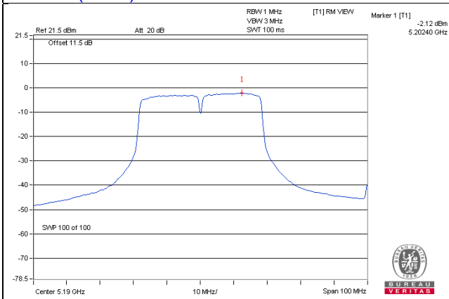
802.11n (HT40) / CH 38 / Chain 1
