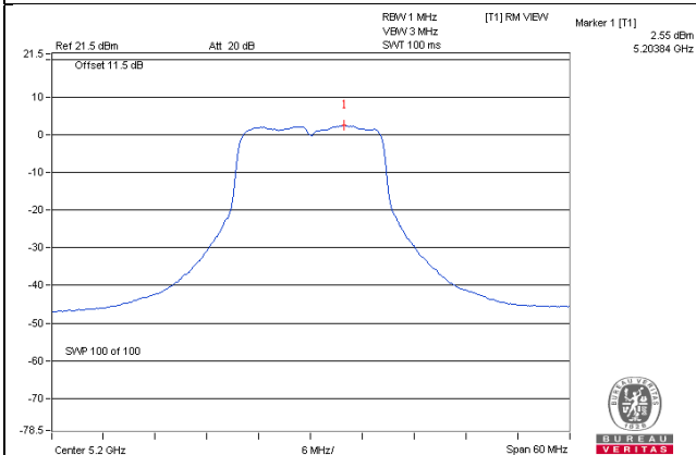
802.11n (HT40) / CH 38 / Chain 1
