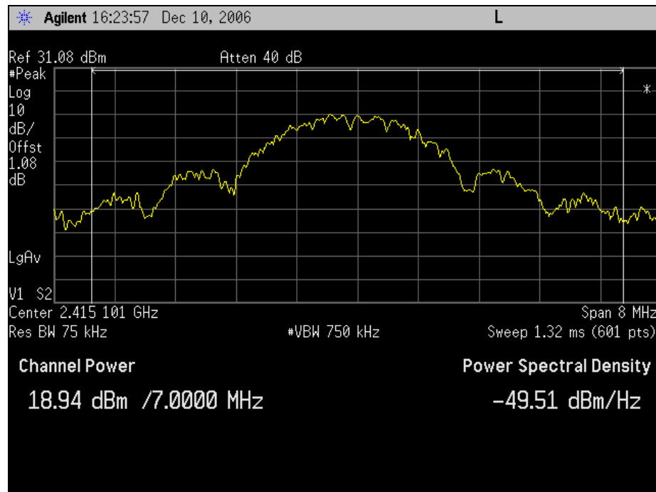
Graph 69. Peak Power Output, Channel 2
