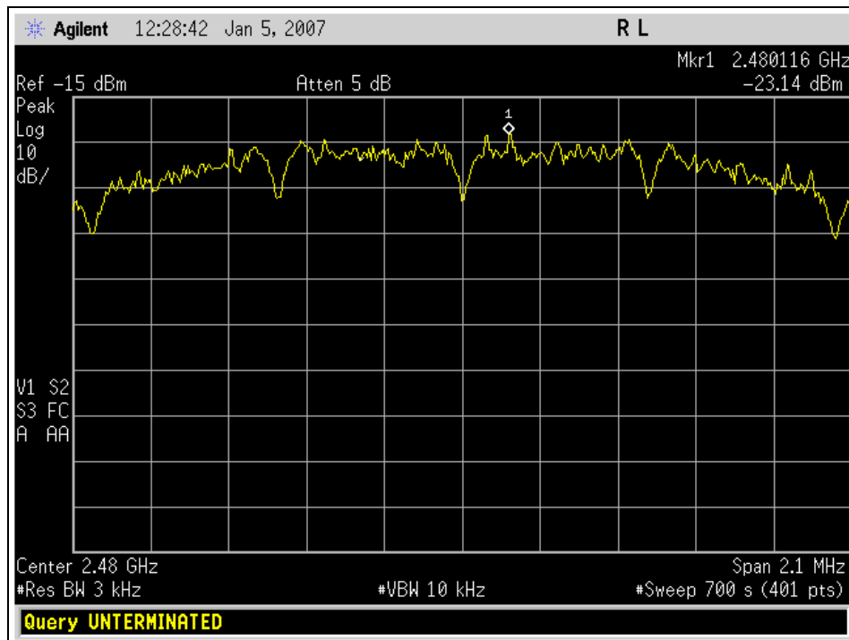
Graph 94. Peak Power Spectral Density, Channel 15
