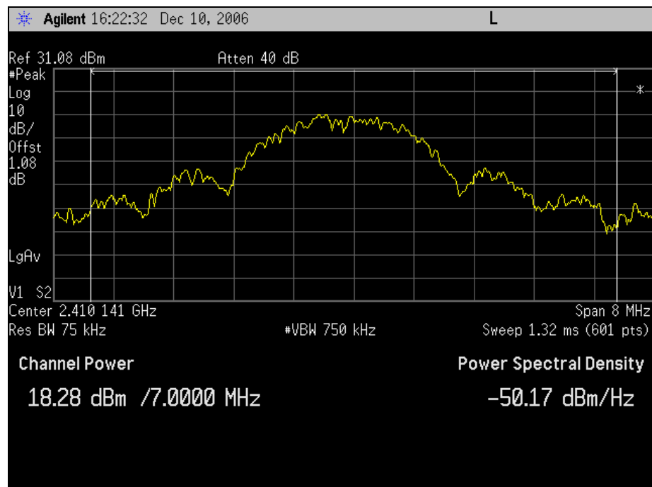
Graph 68. Peak Power Output, Channel 1
