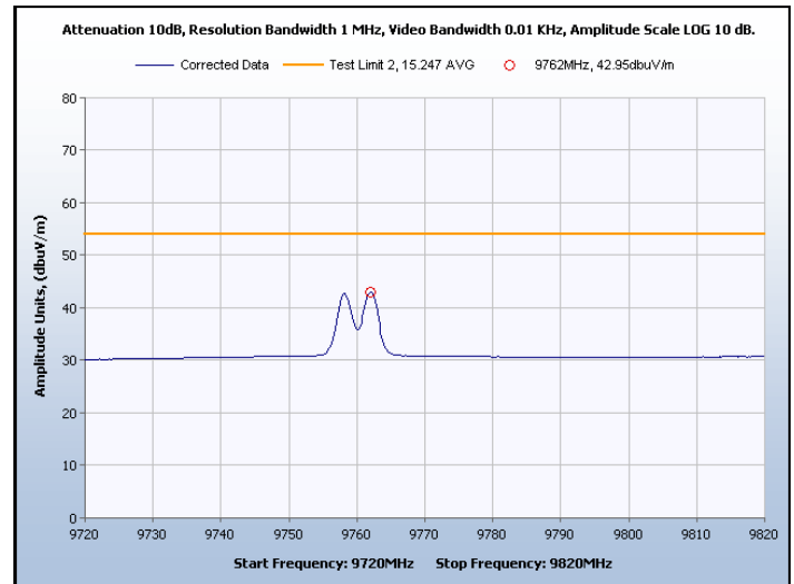
Graph 35. Spurious Radiated Emissions, Channel 7, Average
