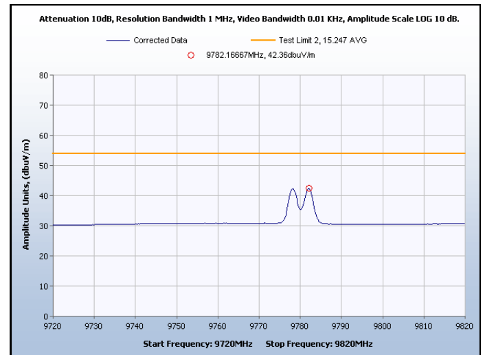
Graph 49. Spurious Radiated Emissions, Channel 8, Average
