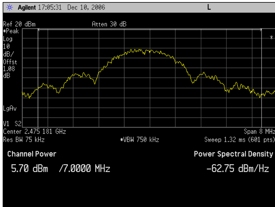
Graph 81. Peak Power Output, Channel 14
