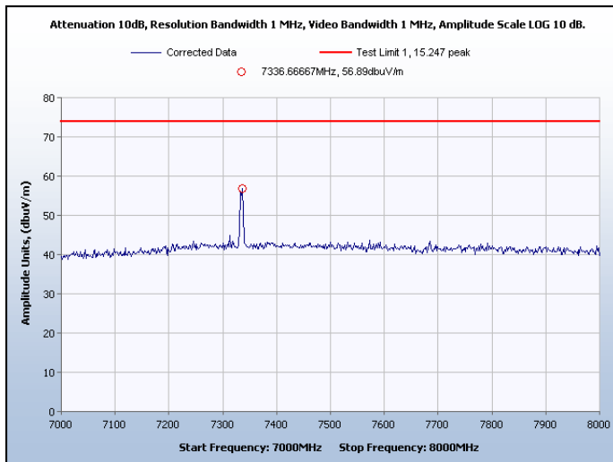
Graph 48. Spurious Radiated Emissions, Channel 8, Peak
