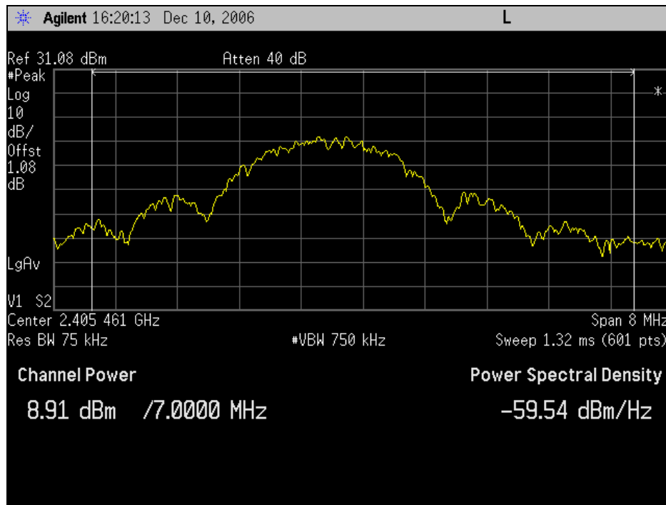
Graph 67. Peak Power Output, Channel 0
