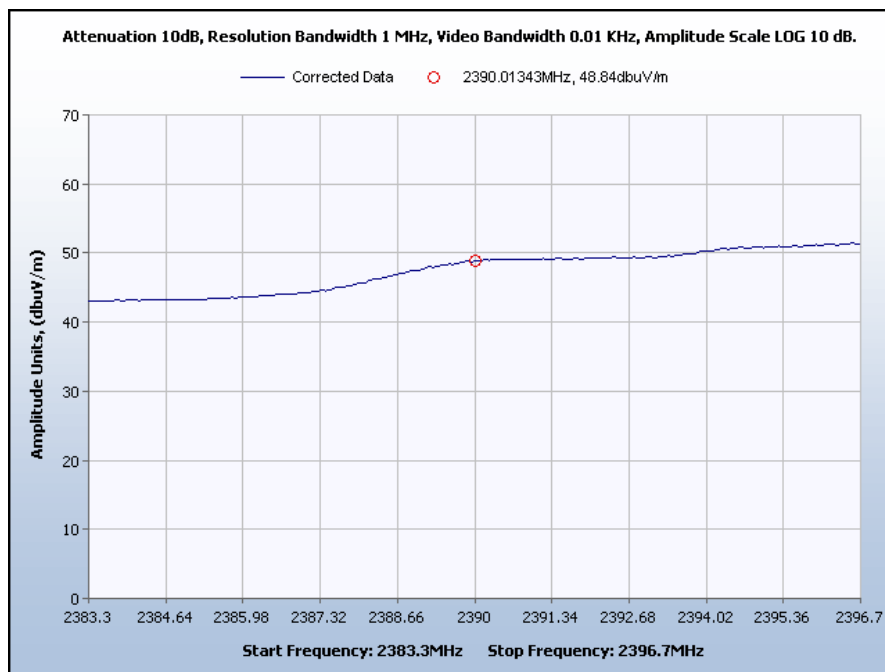
Graph 1. Band Edge Average Emissions, Channel 0
