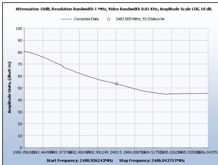
Graph 6. Band Edge Average Emissions, Channel 15
