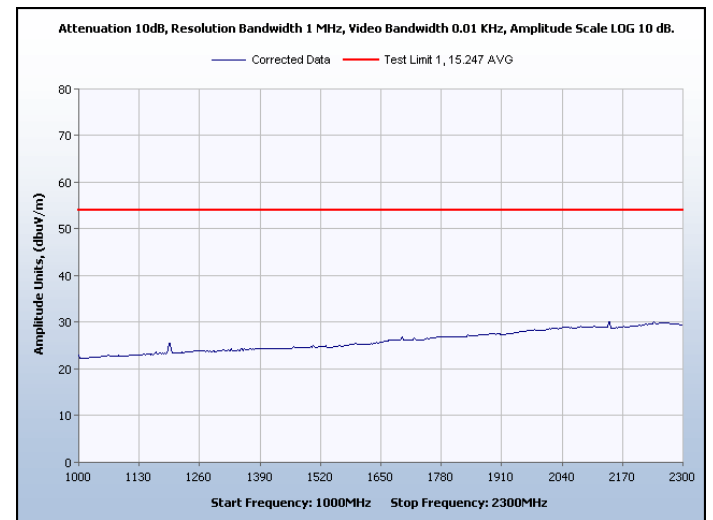
Graph 41. Spurious Radiated Emissions, Channel 8, Average
