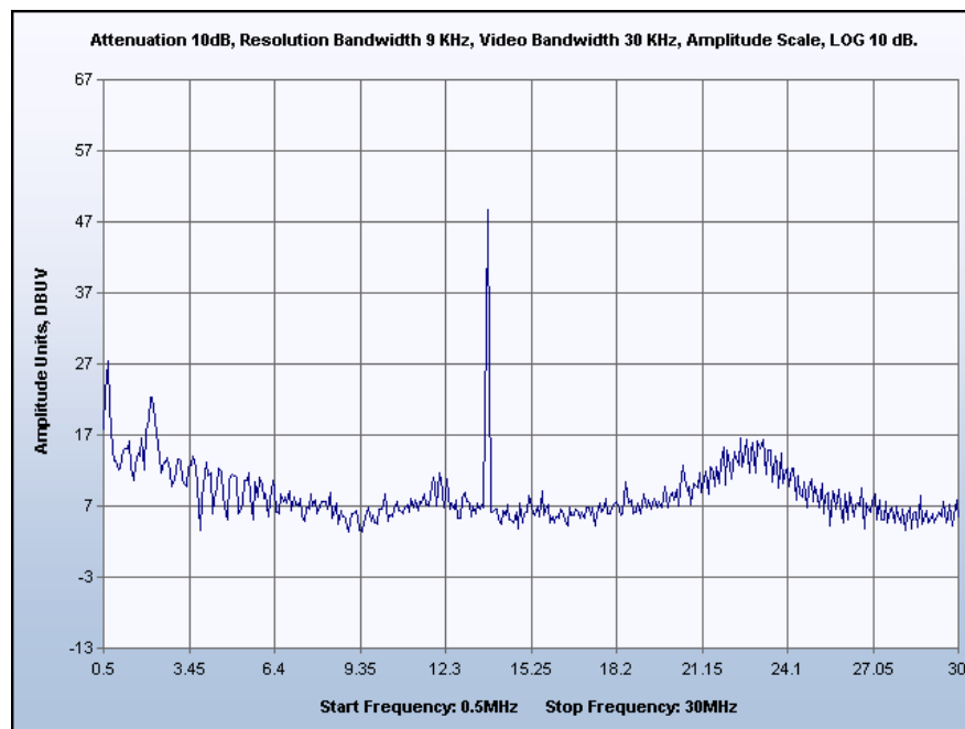
Graph 16. Conducted Emission, High Neutral
