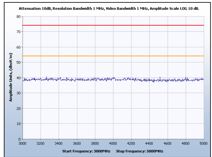
Graph 57. Spurious Radiated Emissions, Channel 15, Peak and Average
