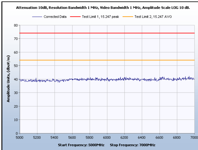
Graph 32. Spurious Radiated Emissions, Channel 7, Peak and Average
