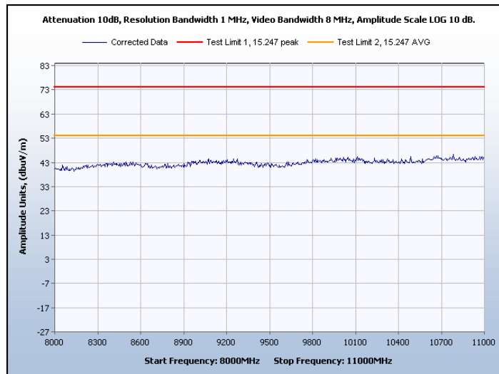
Graph 24. Spurious Radiated Emissions, Channel 0, Peak and Average
