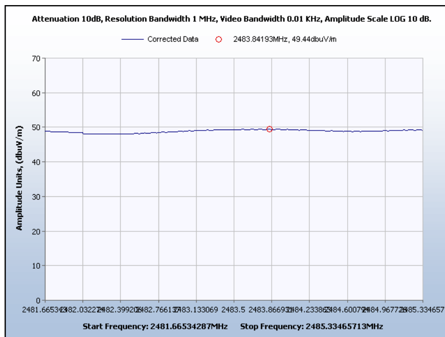
Graph 4. Band Edge Average Emissions, Channel 13
