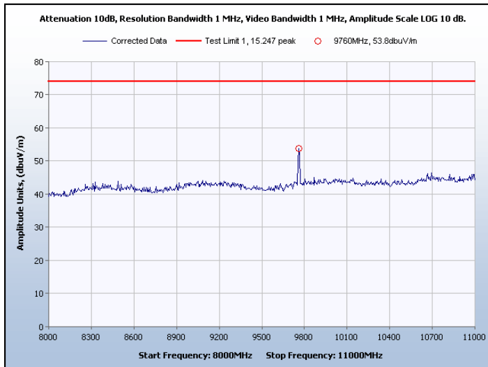
Graph 36. Spurious Radiated Emissions, Channel 7, Peak
