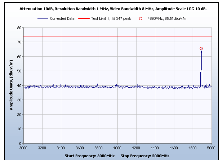
Graph 45. Spurious Radiated Emissions, Channel 8, Peak
