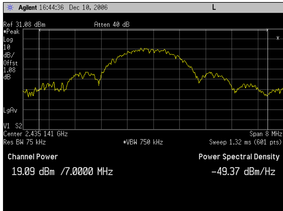
Graph 73. Peak Power Output, Channel 6
