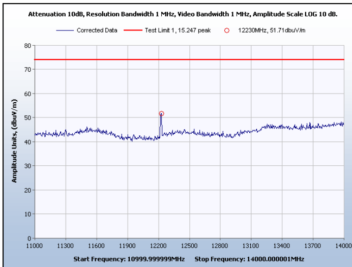
Graph 52. Spurious Radiated Emissions, Channel 8, Peak
