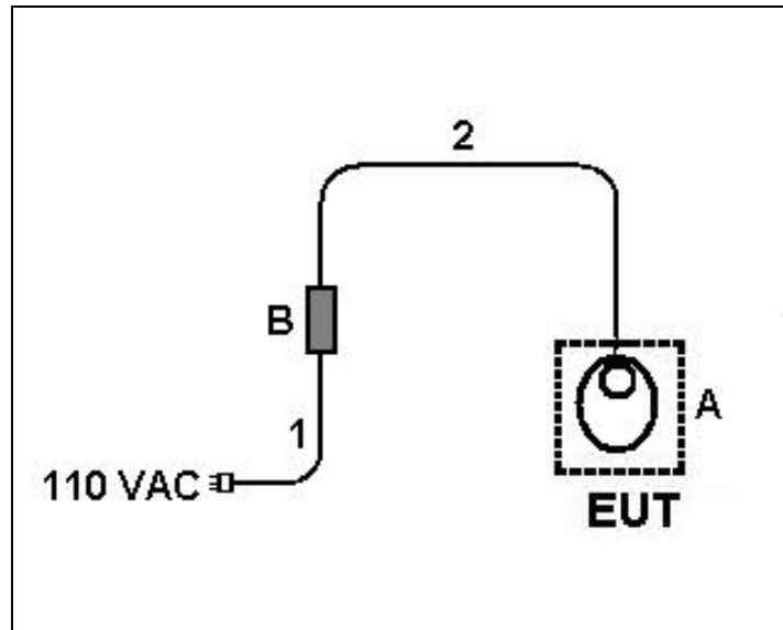
Figure 1. Block Diagram of Test Configuration (Radiated Emissions)
