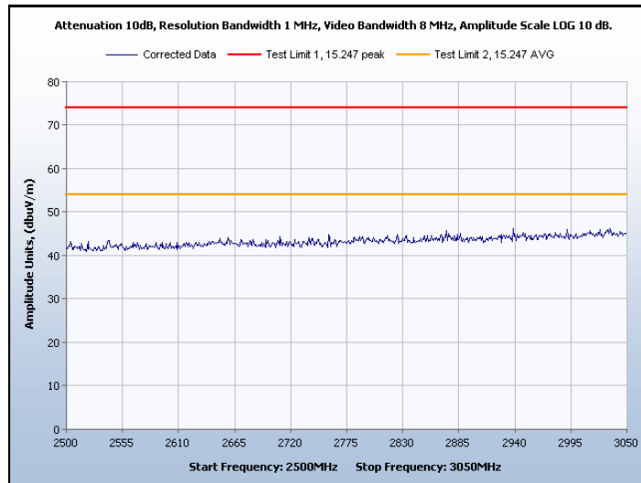
Graph 56. Spurious Radiated Emissions, Channel 15, Peak and Average
