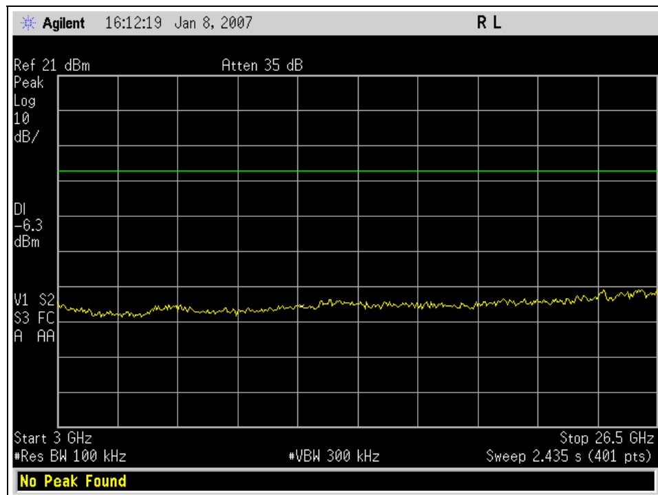
Graph 86. Spurious Conducted Emissions, Channel 7, Mid
