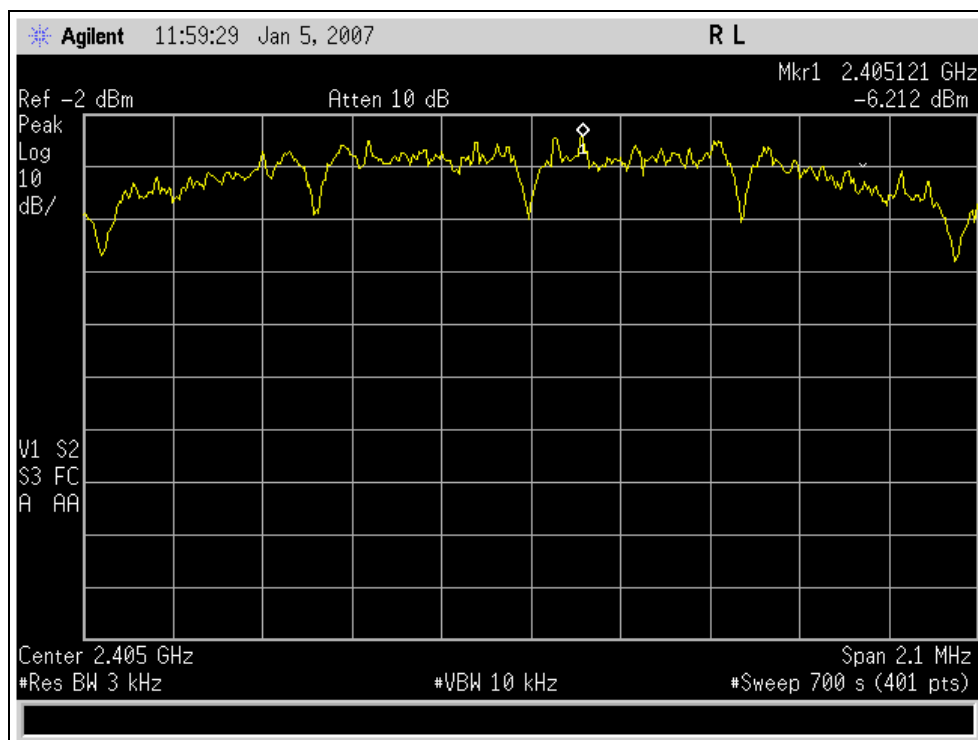
Graph 91. Peak Power Spectral Density, Channel 0
