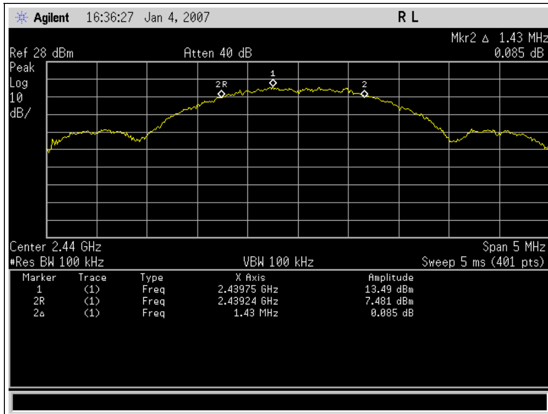
Graph 64. 6 dB Bandwidth, Channel 7
