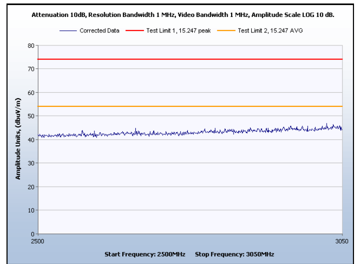
Graph 19. Spurious Radiated Emissions, Channel 0, Peak and Average
