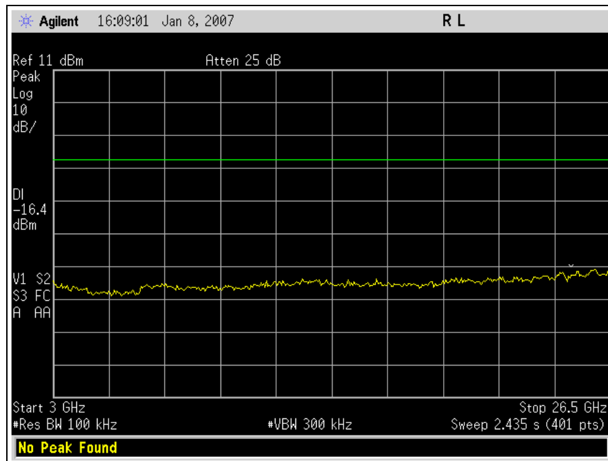
Graph 84. Spurious Conducted Emissions, Channel 0, Mid
