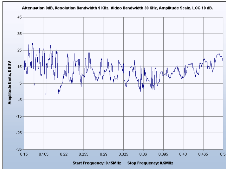
Graph 13. Conducted Emissions, Low Phase
