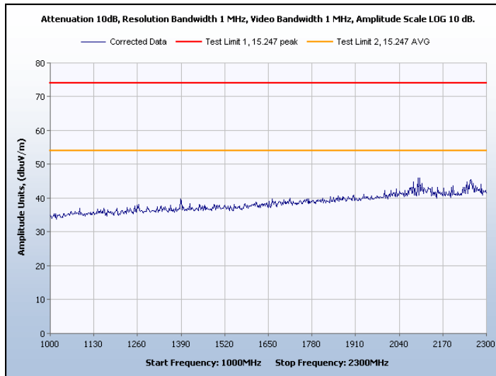
Graph 18. Spurious Radiated Emissions, Channel 0, Peak and Average
