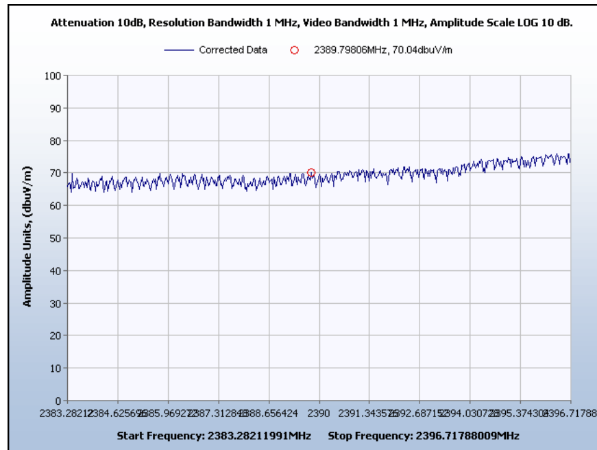
Graph 7. Band Edge Peak Emissions, Channel 0
