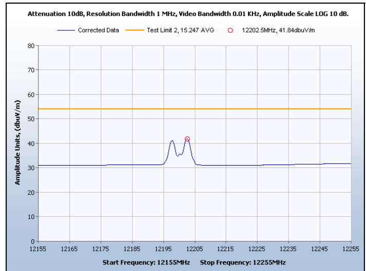
Graph 37. Spurious Radiated Emissions, Channel 7, Average
