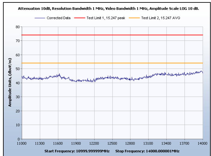
Graph 61. Spurious Radiated Emissions, Channel 15, Peak and Average
