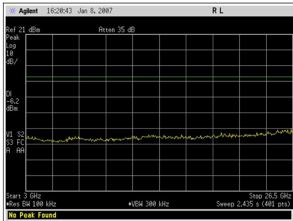
Graph 88. Spurious Conducted Emissions, Channel 8, Mid
