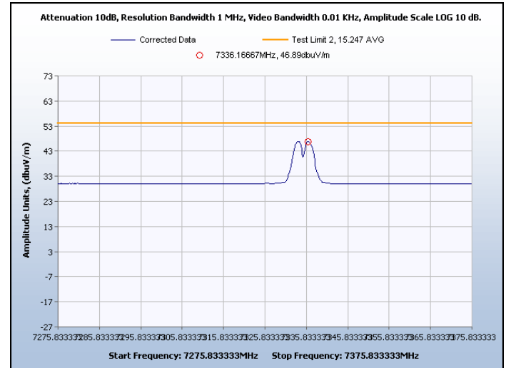
Graph 47. Spurious Radiated Emissions, Channel 8, Average
