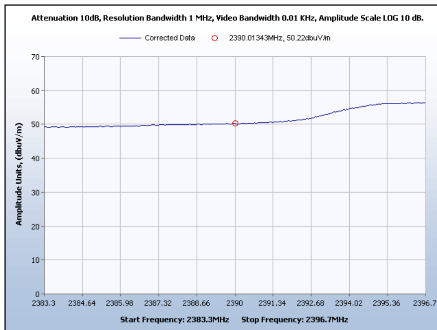
Graph 2. Band Edge Average Emissions, Channel 1
