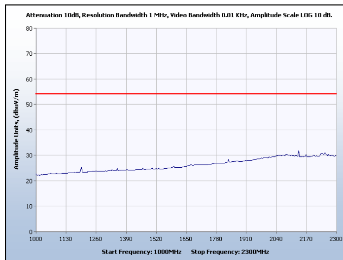
Graph 27. Spurious Radiated Emissions, Channel 7, Average
