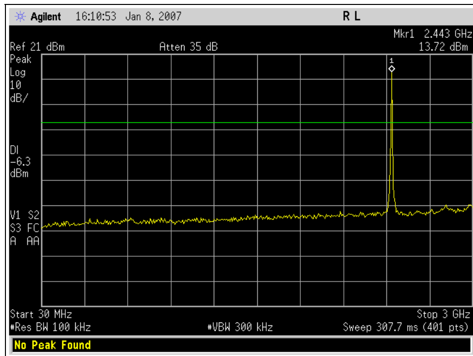
Graph 85. Spurious Conducted Emissions, Channel 7, Low
