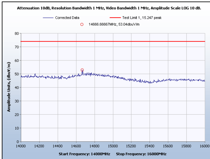
Graph 54. Spurious Radiated Emissions, Channel 8, Peak
