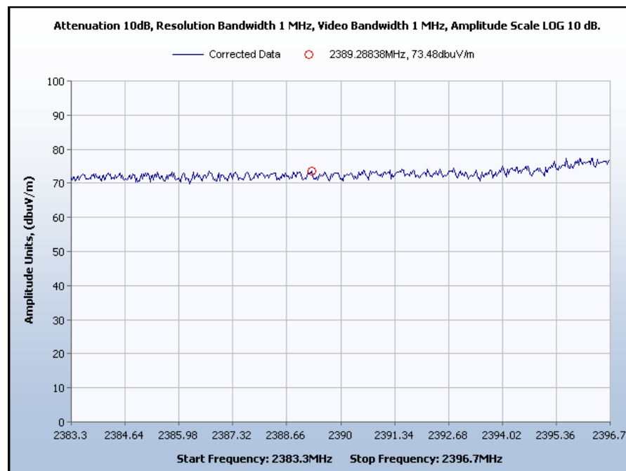
Graph 8. Band Edge Peak Emissions, Channel 1
