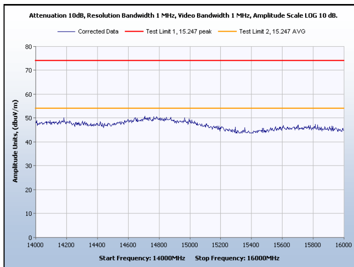
Graph 26. Spurious Radiated Emissions, Channel 0, Peak and Average
