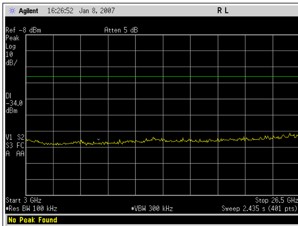
Graph 90. Spurious Conducted Emissions, Channel 15, Mid
