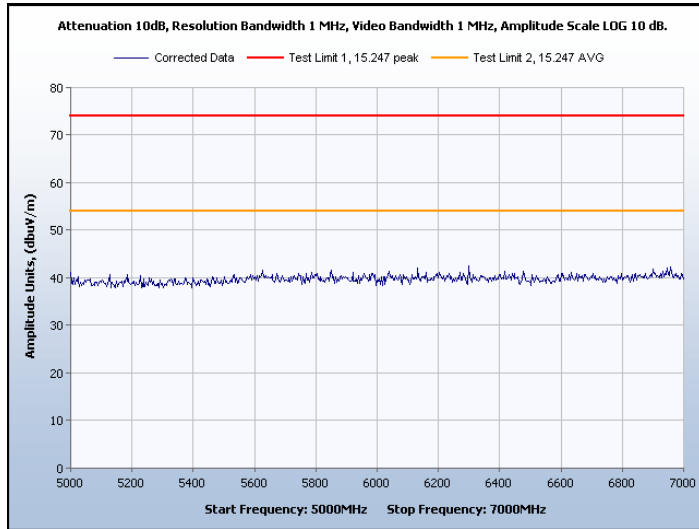
Graph 22. Spurious Radiated Emissions, Channel 0, Peak and Average
