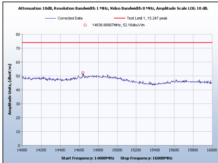
Graph 40. Spurious Radiated Emissions, Channel 7, Peak
