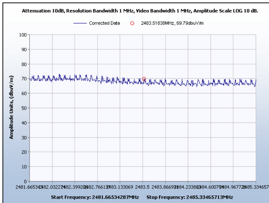
Graph 11. Band Edge Peak Emissions, Channel 14
