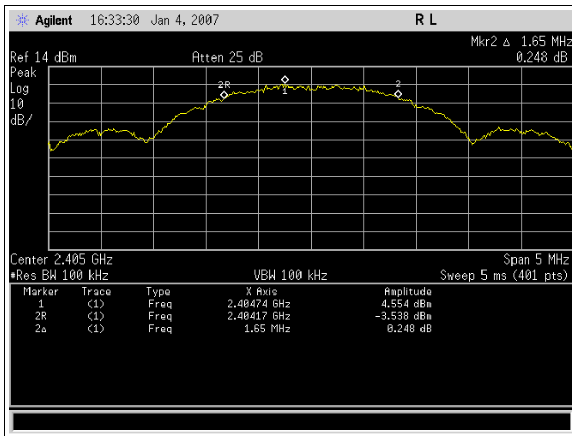
Graph 63. 6 dB Bandwidth, Channel 0
