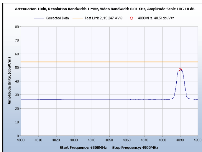
Graph 44. Spurious Radiated Emissions, Channel 8, Average
