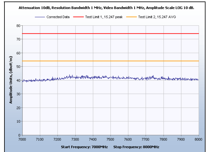
Graph 59. Spurious Radiated Emissions, Channel 15, Peak and Average
