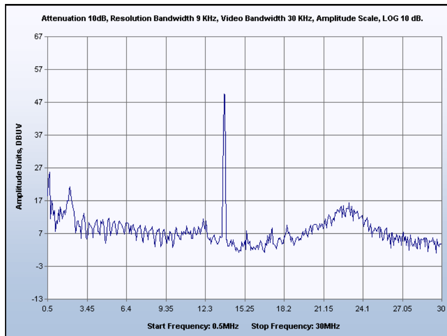
Graph 14. Conducted Emission, High Phase
