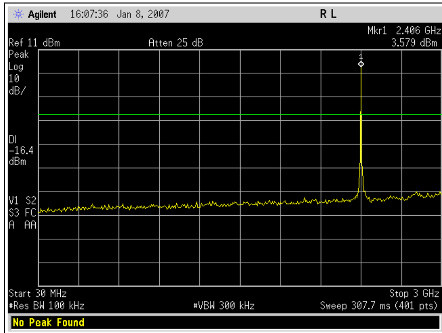
Graph 83. Spurious Conducted Emissions, Channel 0, Low
