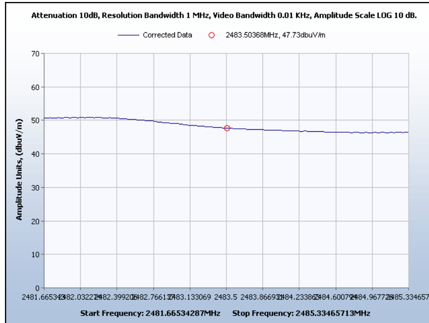
Graph 5. Band Edge Average Emissions, Channel 14
