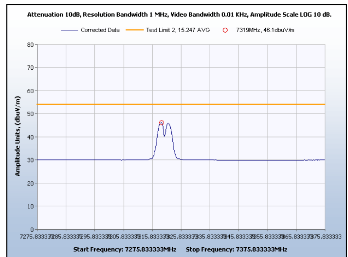
Graph 33. Spurious Radiated Emissions, Channel 7, Average
