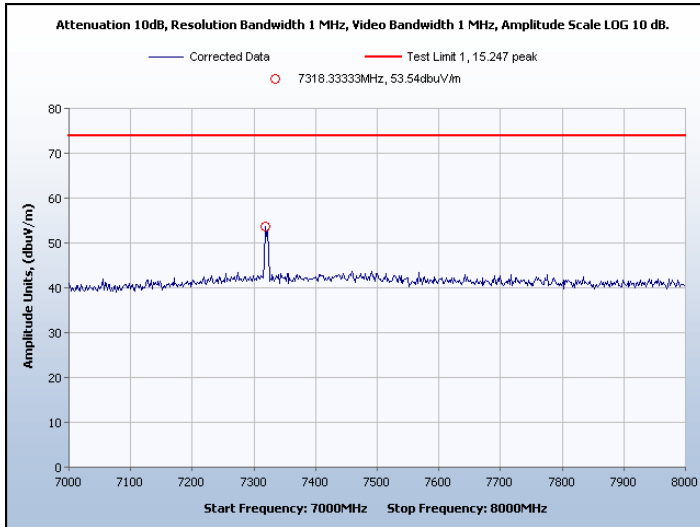
Graph 34. Spurious Radiated Emissions, Channel 7, Peak
