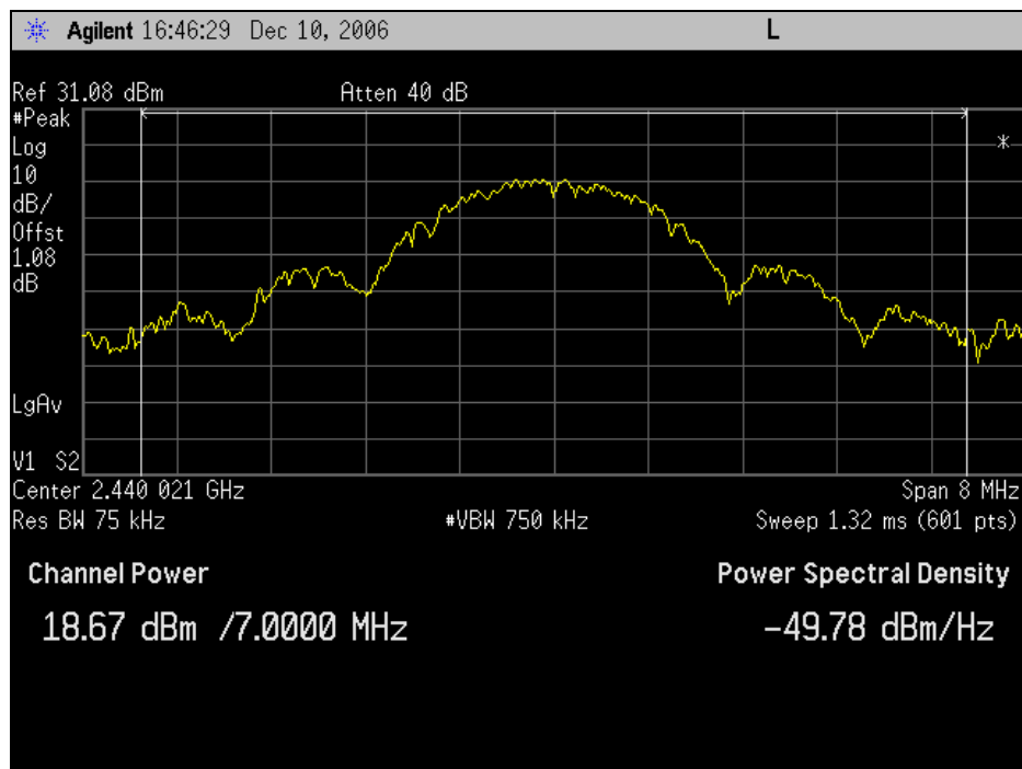
Graph 74. Peak Power Output, Channel 7
