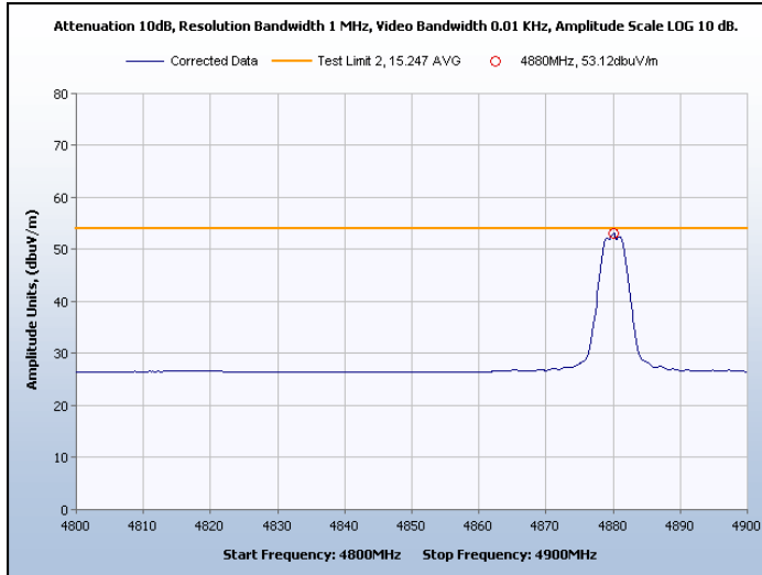
Graph 30. Spurious Radiated Emissions, Channel 7, Average
