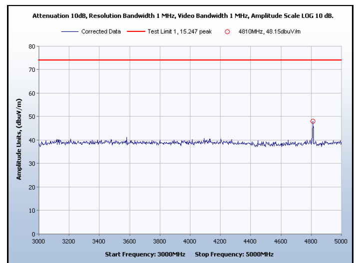
Graph 21. Spurious Radiated Emissions, Channel 0, Peak
