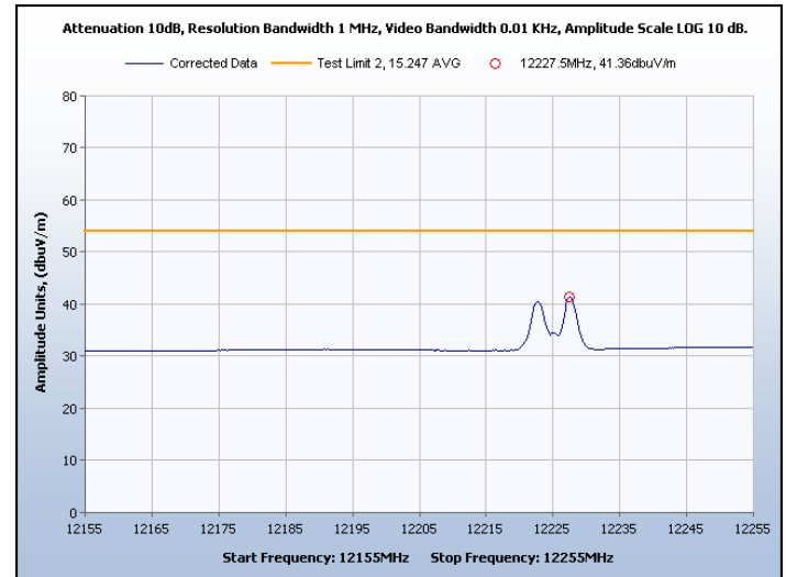
Graph 51. Spurious Radiated Emissions, Channel 8, Average
