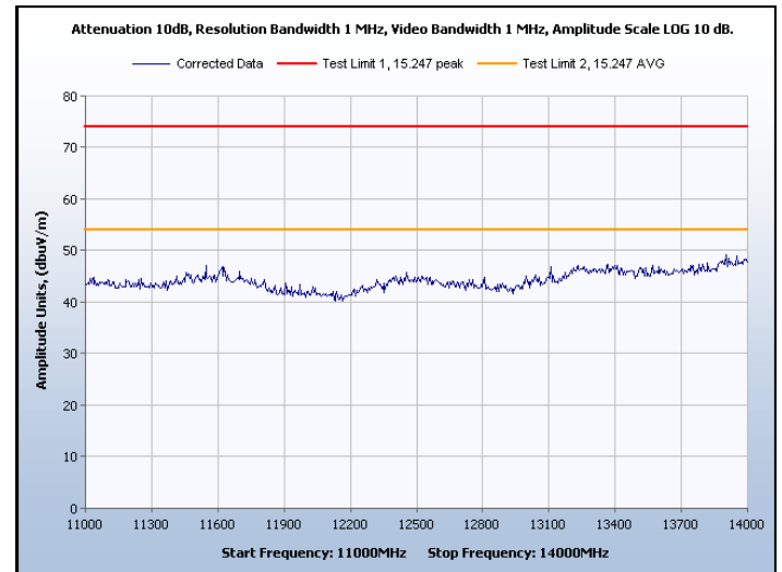
Graph 25. Spurious Radiated Emissions, Channel 0, Peak and Average
