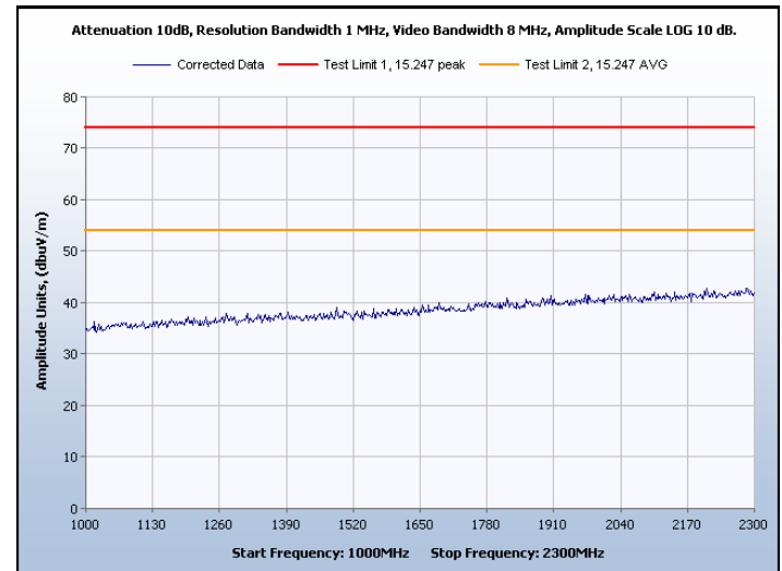
Graph 55. Spurious Radiated Emissions, Channel 15, Peak and Average
