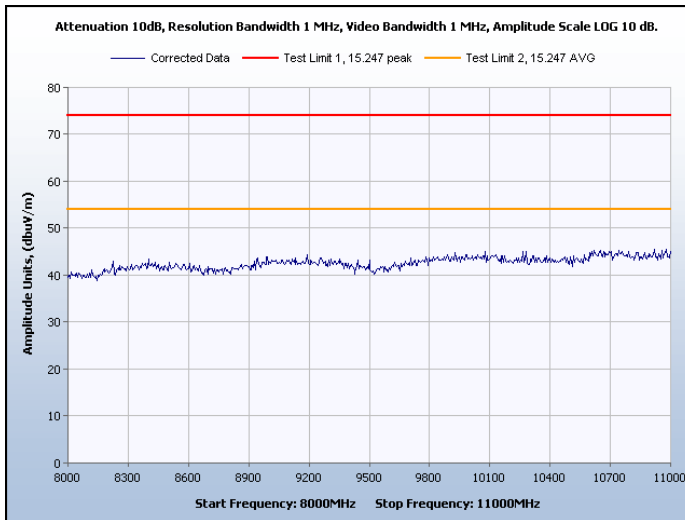
Graph 60. Spurious Radiated Emissions, Channel 15, Peak and Average
