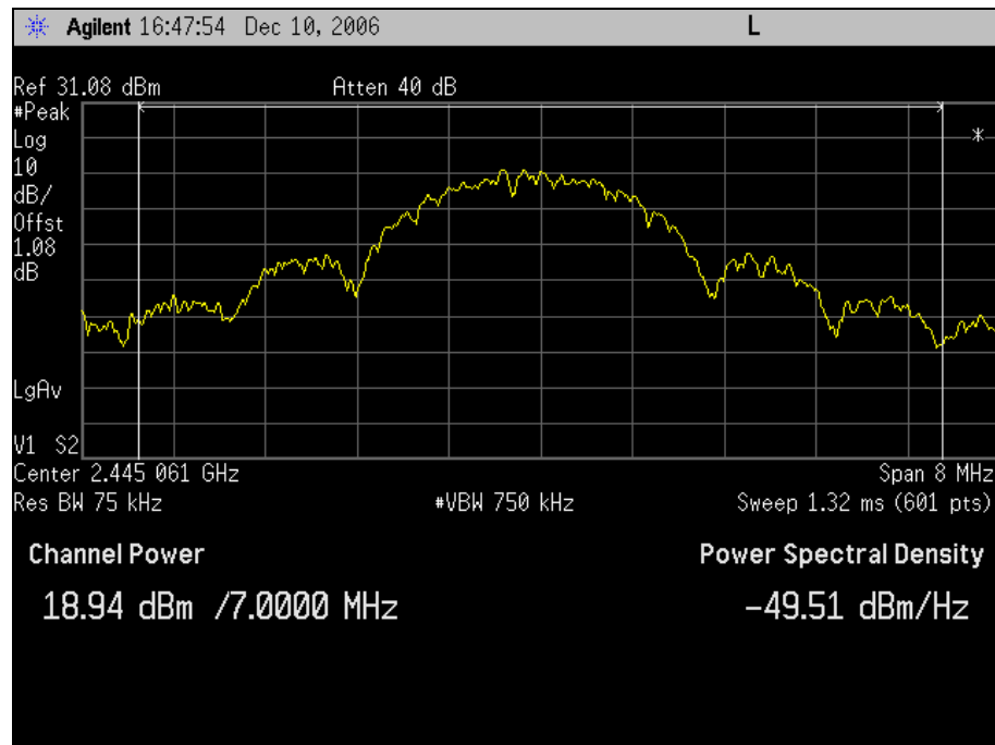
Graph 75. Peak Power Output, Channel 8
