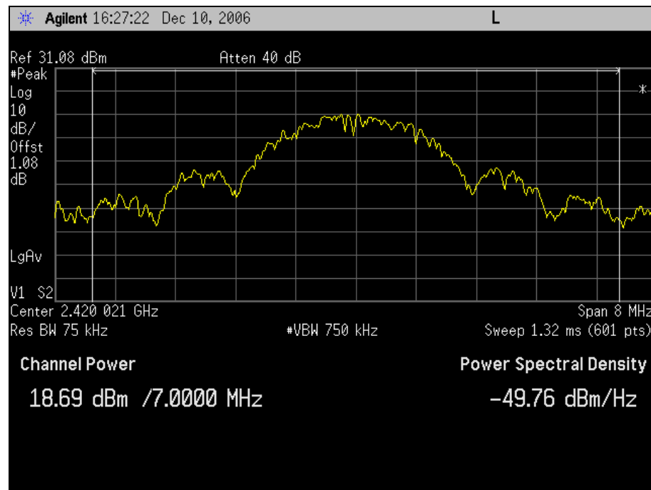
Graph 70. Peak Power Output, Channel 3
