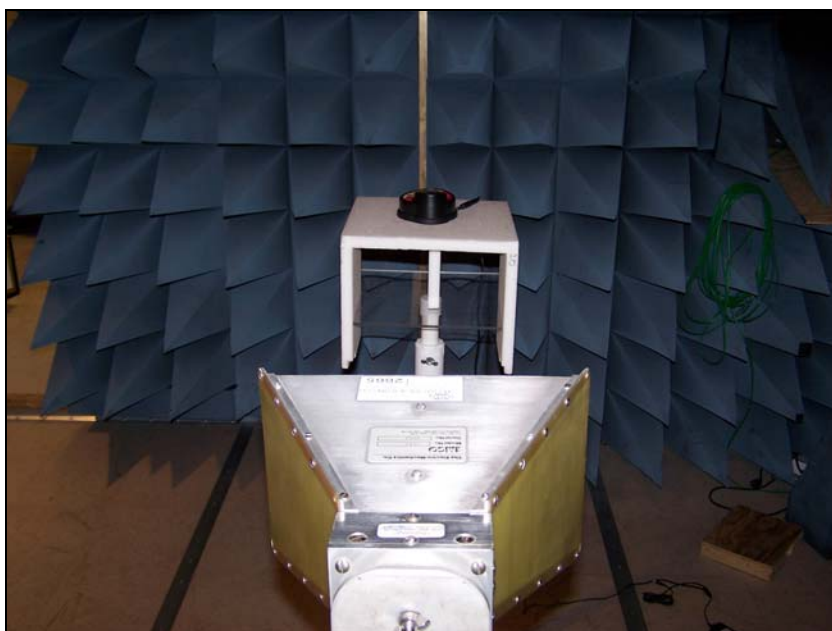
Photograph 3. Spurious Radiated Emissions, Test Setup
