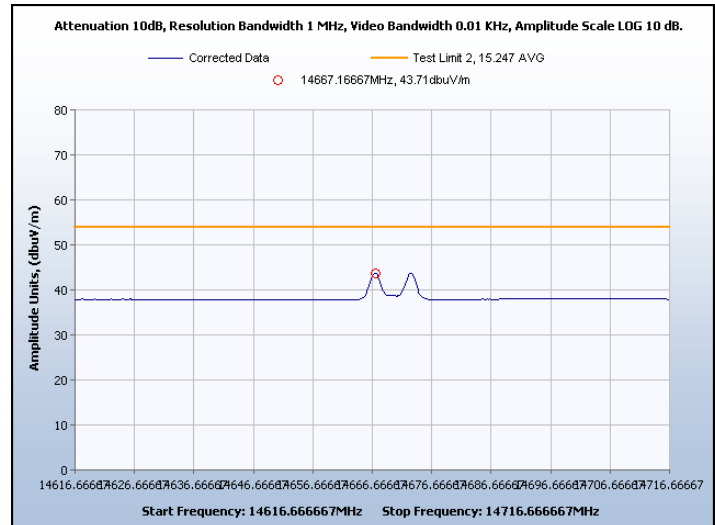
Graph 53. Spurious Radiated Emissions, Channel 8, Average
