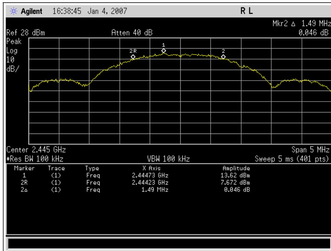
Graph 65. 6 dB Bandwidth, Channel 8
