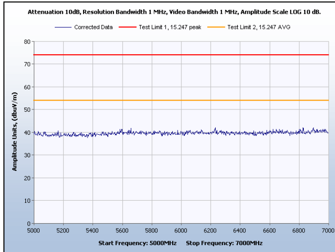
Graph 58. Spurious Radiated Emissions, Channel 15, Peak and Average
