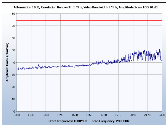
Graph 28. Spurious Radiated Emissions, Channel 7, Peak
