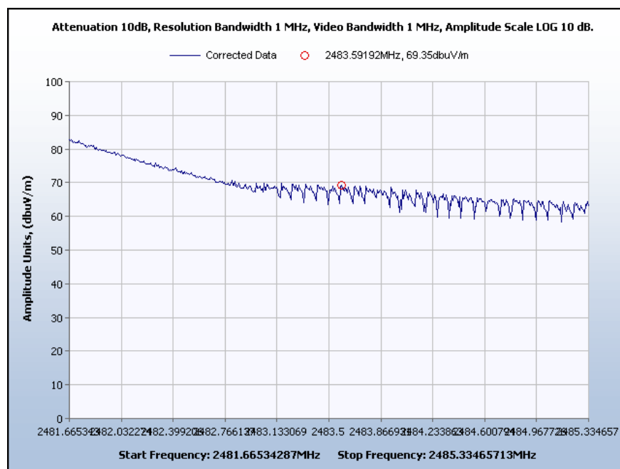
Graph 12. Band Edge Peak Emissions, Channel 15
