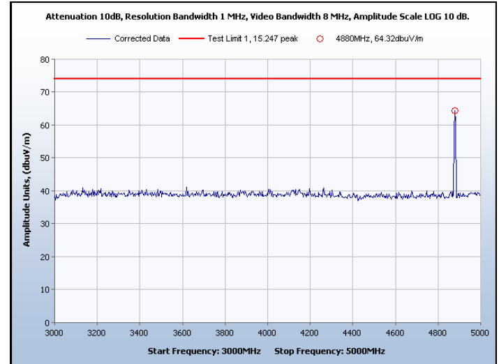
Graph 31. Spurious Radiated Emissions, Channel 7, Peak
