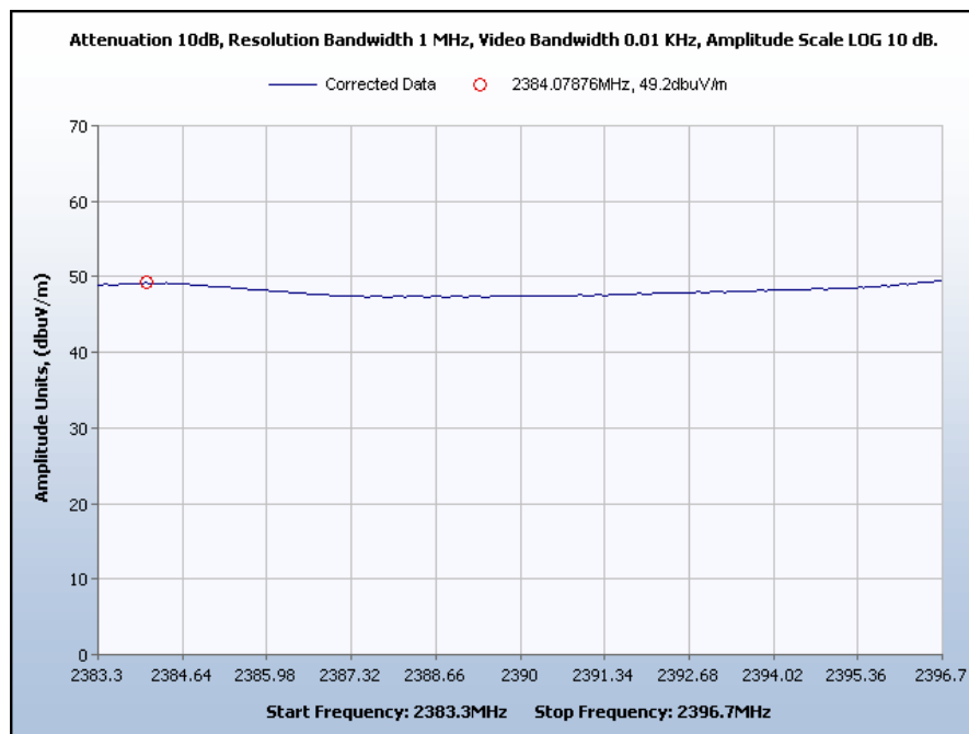
Graph 3. Band Edge Average Emissions, Channel 2
