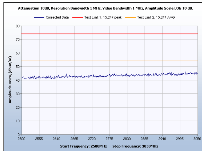
Graph 29. Spurious Radiated Emissions, Channel 7, Peak and Average
