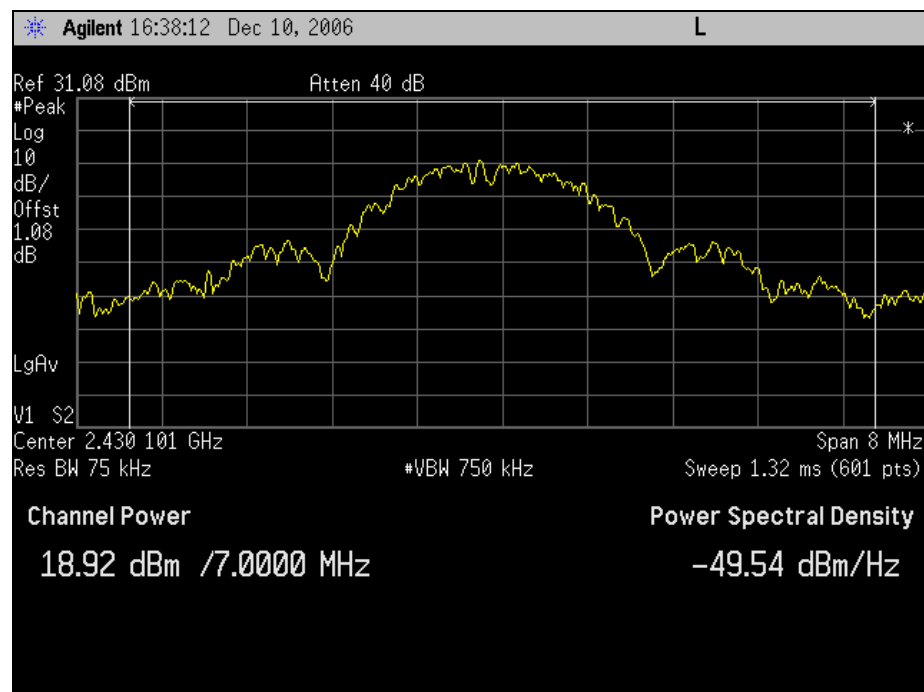
Graph 72. Peak Power Output, Channel 5
