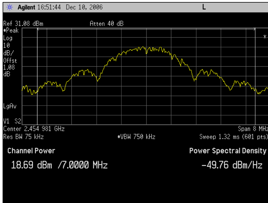
Graph 77. Peak Power Output, Channel 10
