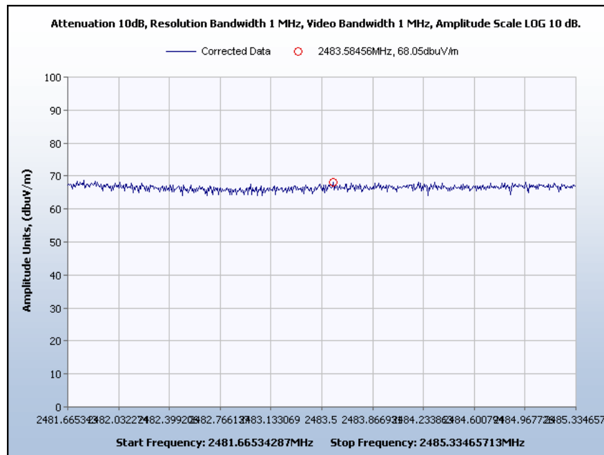
Graph 10. Band Edge Peak Emissions, Channel 13
