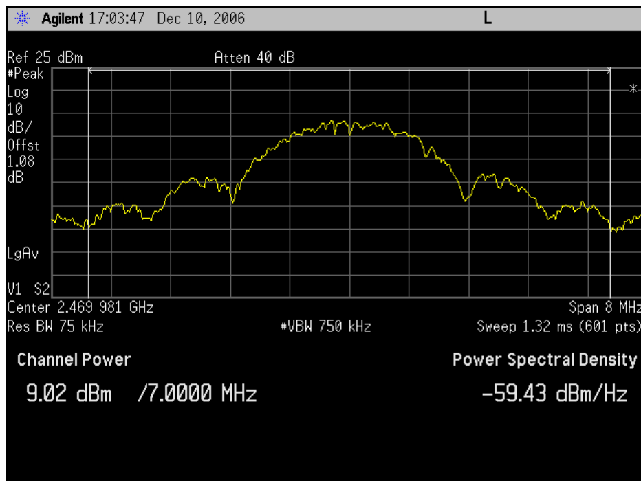
Graph 80. Peak Power Output, Channel 13
