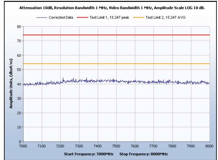
Graph 23. Spurious Radiated Emissions, Channel 0, Peak and Average
