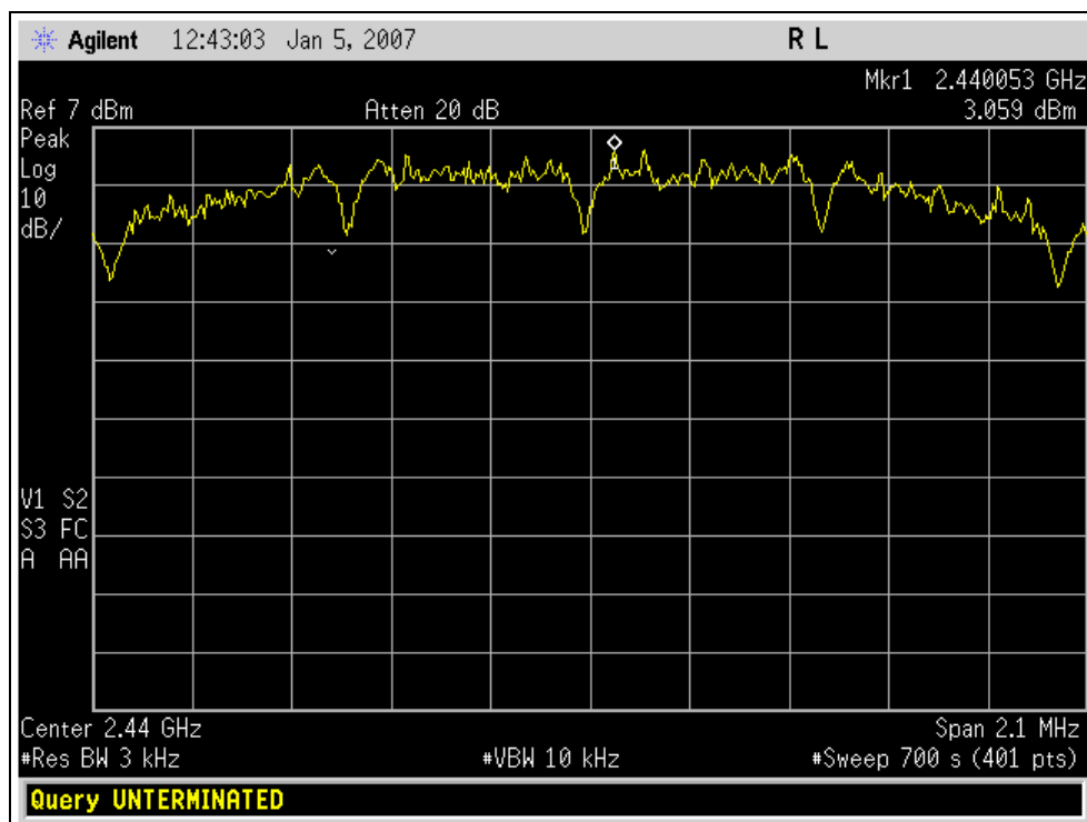
Graph 92. Peak Power Spectral Density, Channel 7
