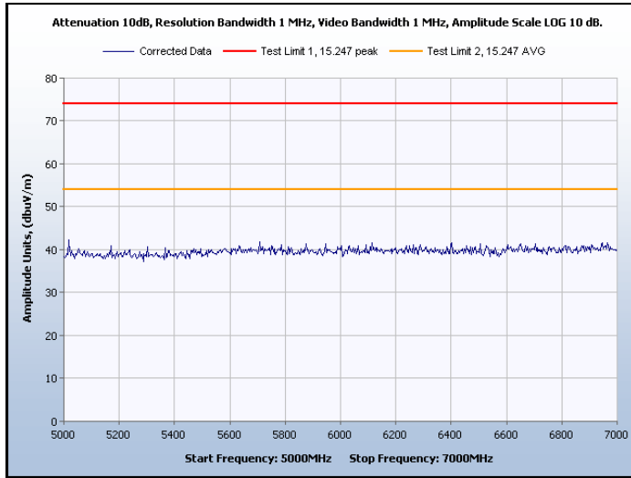
Graph 46. Spurious Radiated Emissions, Channel 8, Peak and Average
