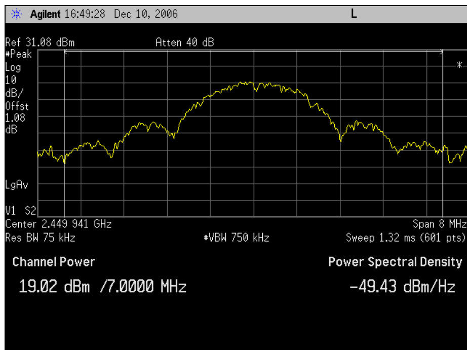
Graph 76. Peak Power Output, Channel 9
