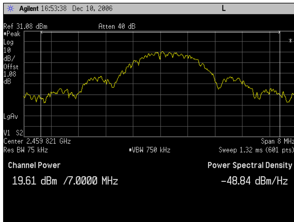
Graph 78. Peak Power Output, Channel 11
