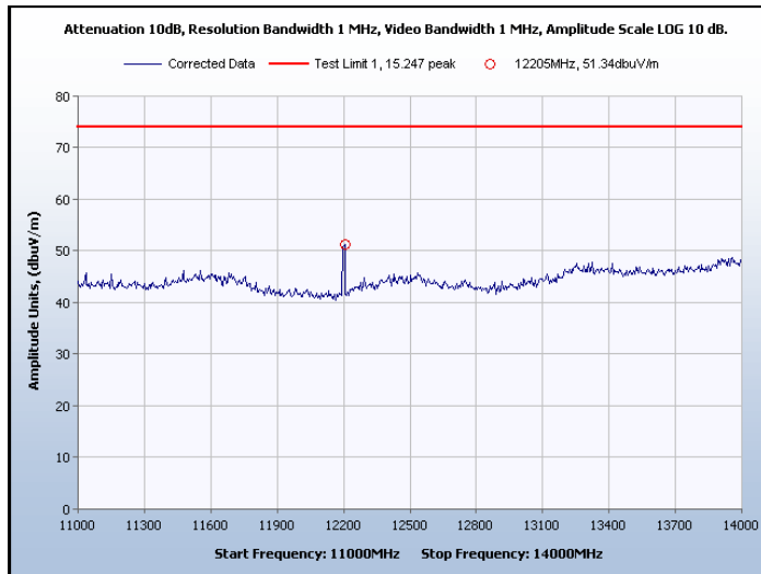
Graph 38. Spurious Radiated Emissions, Channel 7, Peak
