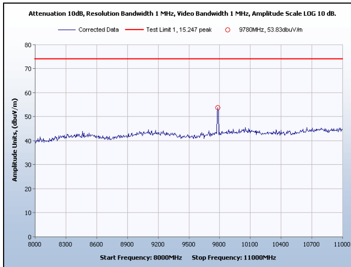
Graph 50. Spurious Radiated Emissions, Channel 8, Peak
