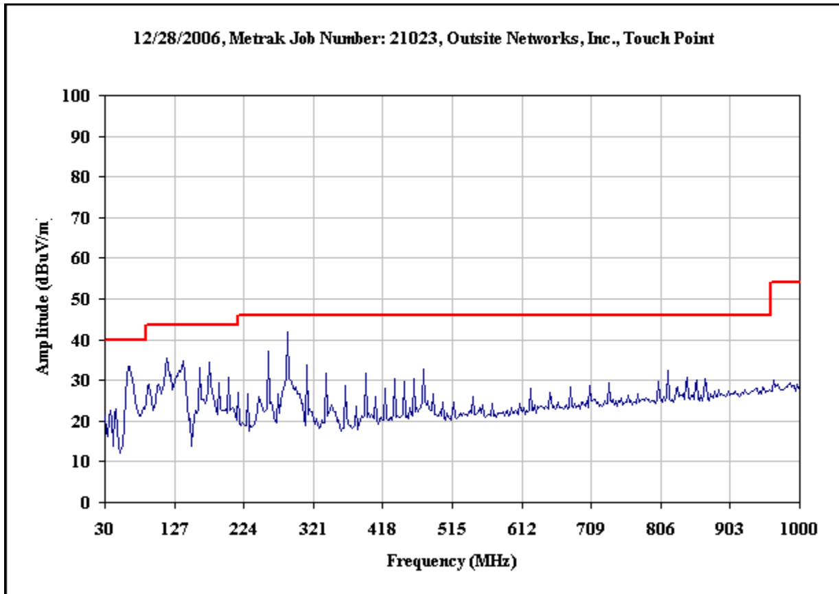
Graph 17. Radiated Emissions (30 MHz to 1 GHz), Pre-Scan
