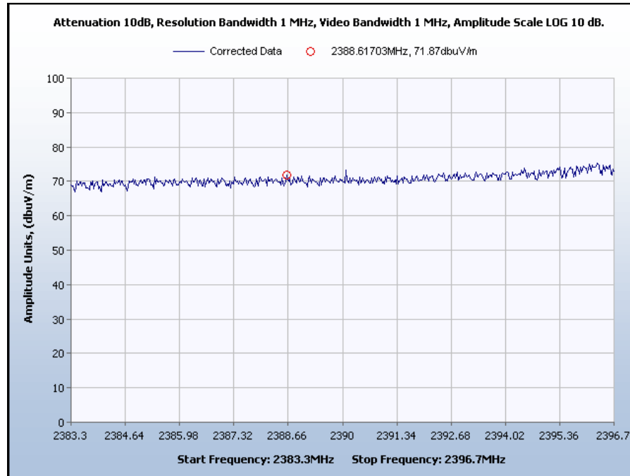
Graph 9. Band Edge Peak Emissions, Channel 2
