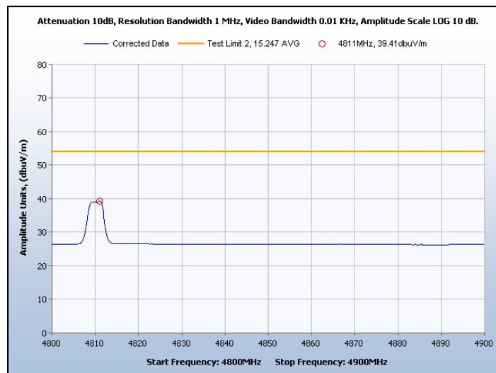
Graph 20. Spurious Radiated Emissions, Channel 0, Average
