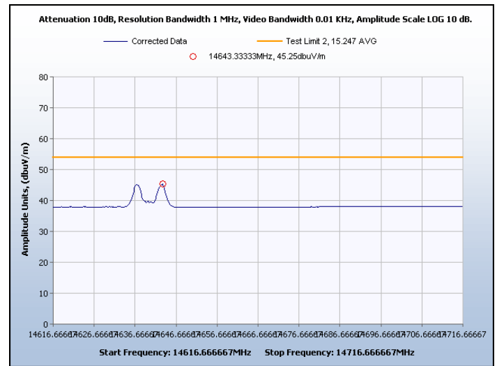
Graph 39. Spurious Radiated Emissions, Channel 7, Average
