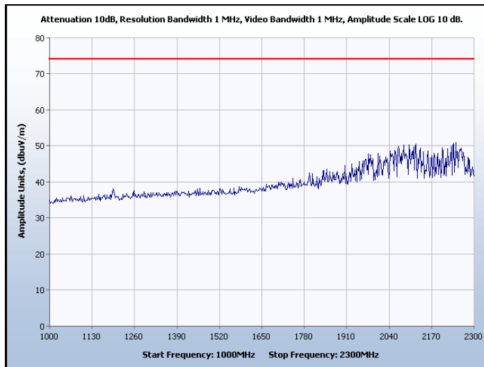
Graph 42. Spurious Radiated Emissions, Channel 8, Peak
