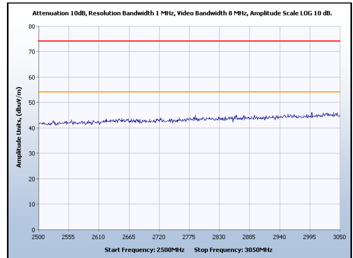
Graph 43. Spurious Radiated Emissions, Channel 8, Peak and Average
