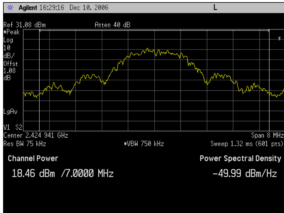
Graph 71. Peak Power Output, Channel 4
