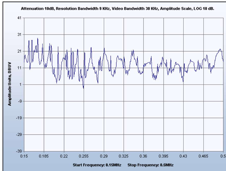
Graph 15. Conducted Emission, Low Neutral
