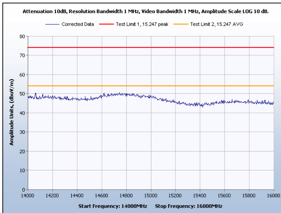
Graph 62. Spurious Radiated Emissions, Channel 15, Peak and Average
