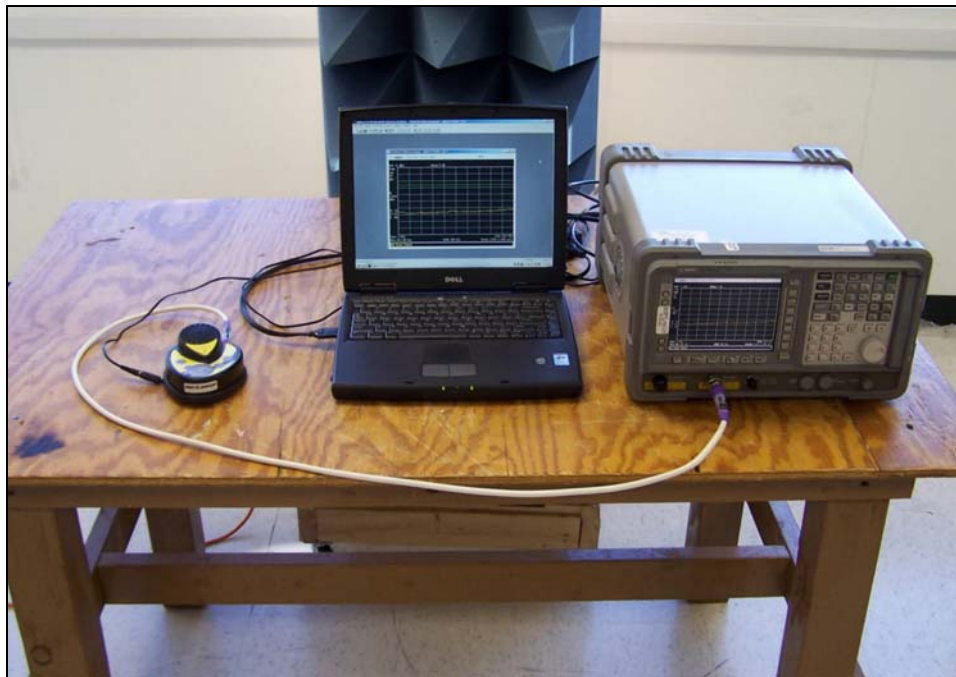
Photograph 6. Spurious Conducted Emissions, Test Setup
