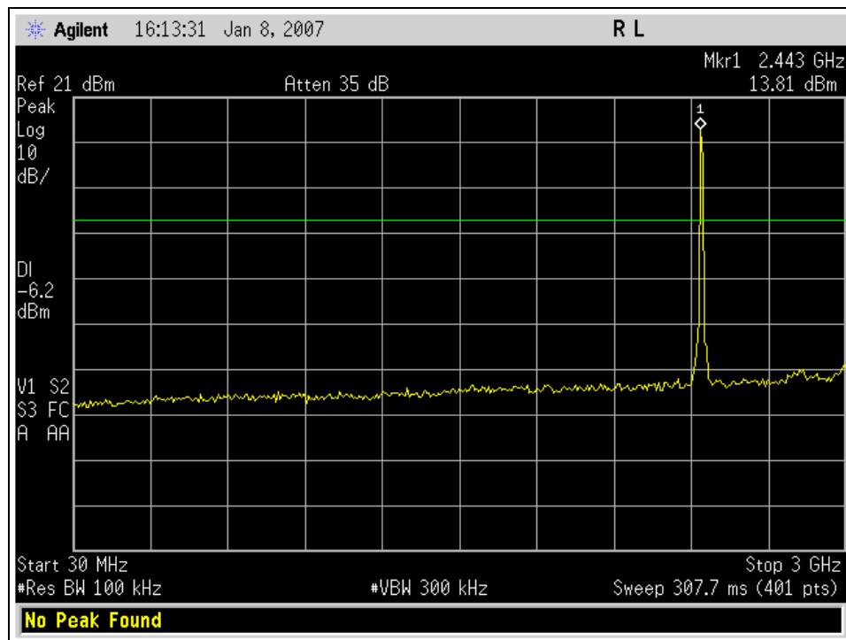
Graph 87. Spurious Conducted Emissions, Channel 8, Low
