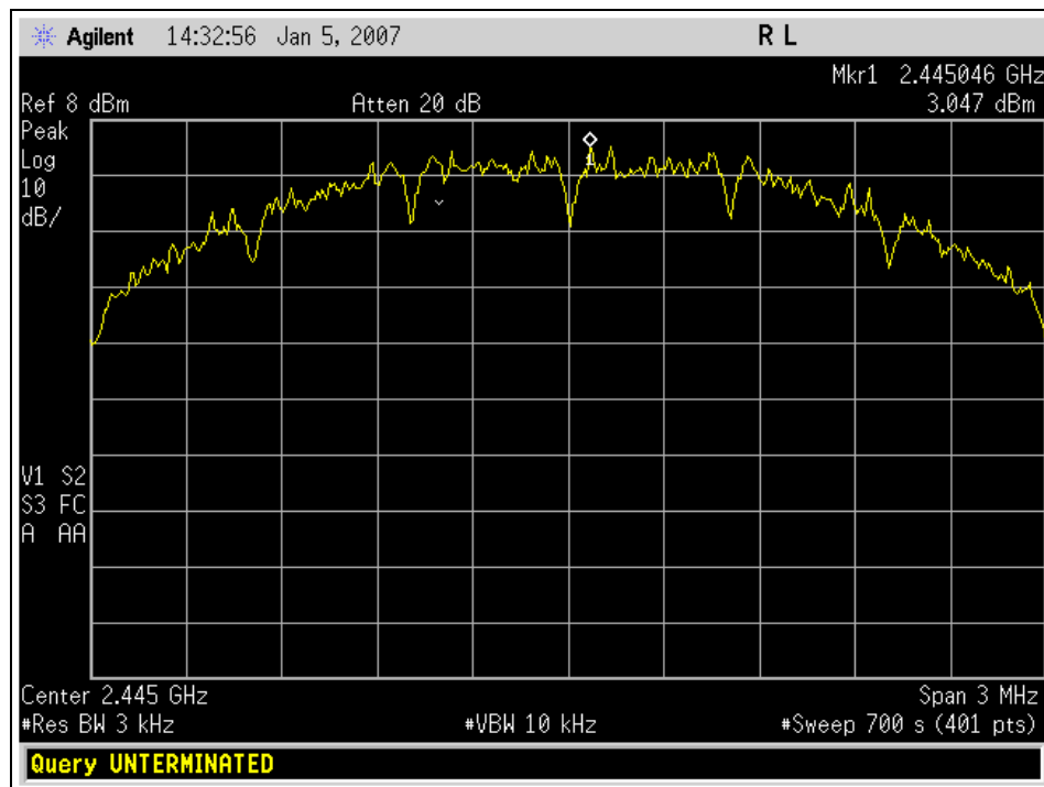
Graph 93. Peak Power Spectral Density, Channel 8
