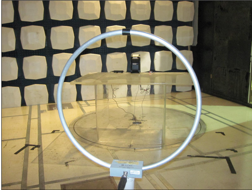
Photograph 6. Radiated Spurious Emissions, Below 30 MHz, Test Setup
