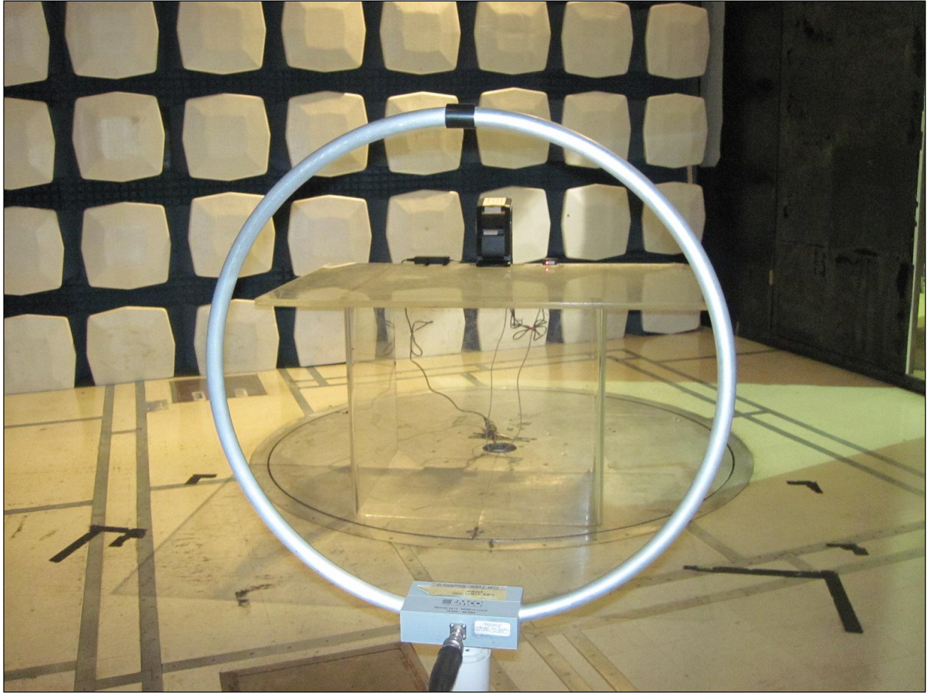
Photograph 5. Field Strength of Fundamental Emission, Test Setup
