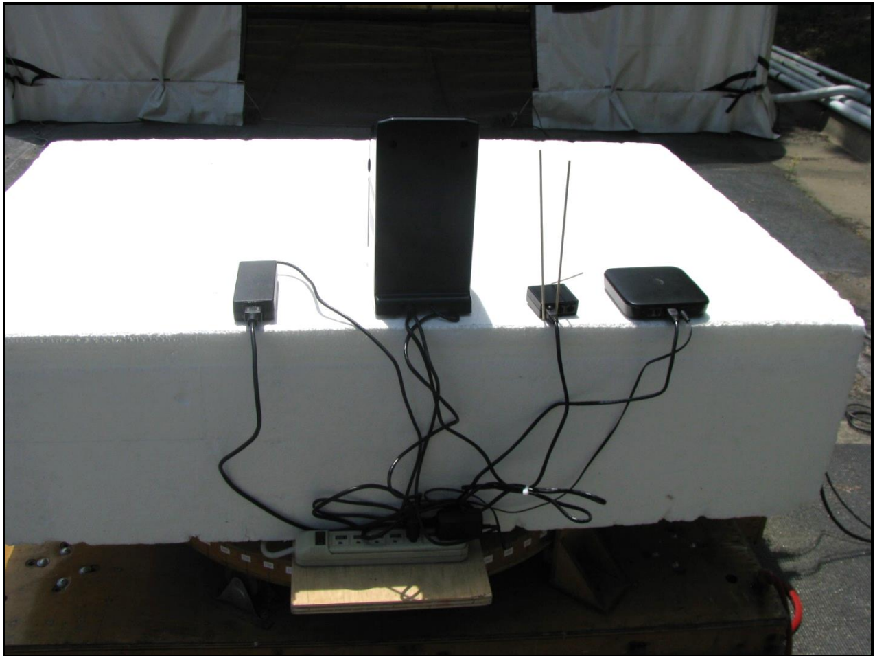
Photograph 3: Radiated Testing – Rear View
