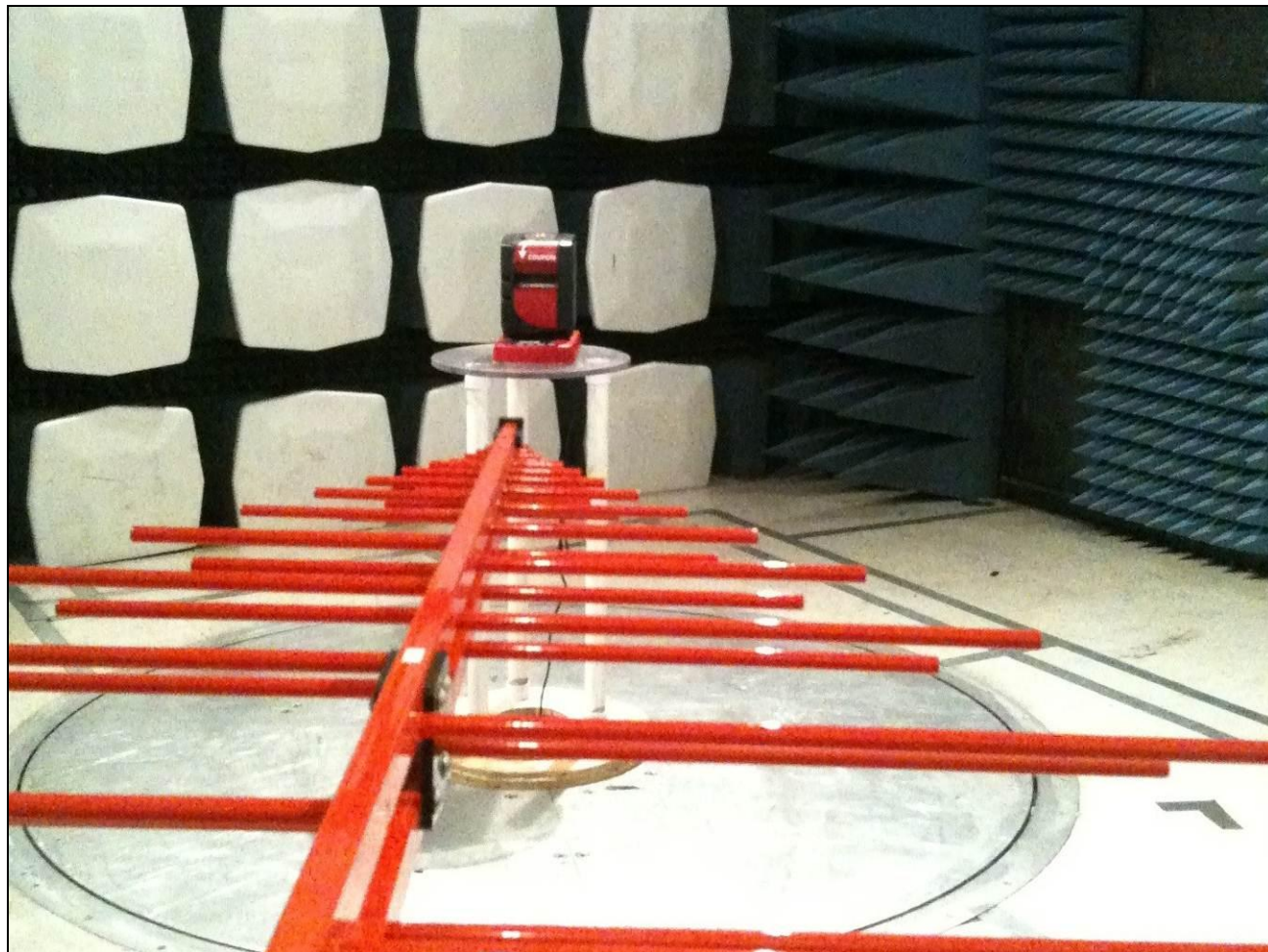
Photograph 3. Radiated Spurious Emissions, Below 1 GHz, Test Setup Photo
