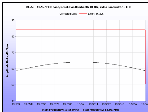
Plot 5. Field Strength of Fundamental Emissions, 13.553 – 13.567 MHz Band
