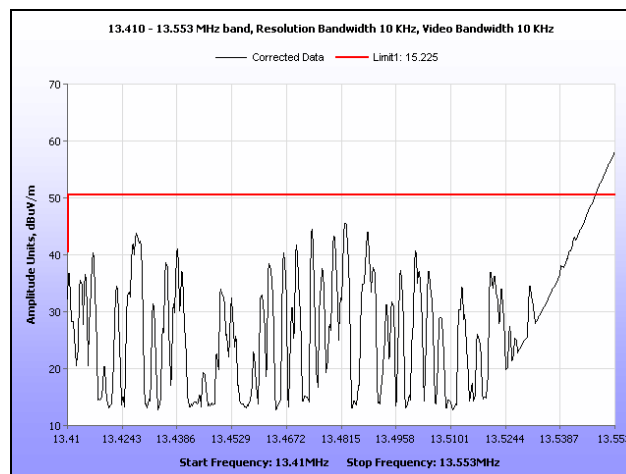
Plot 4. Field Strength of Fundamental Emission, 13.410 – 13.553 MHz Band
