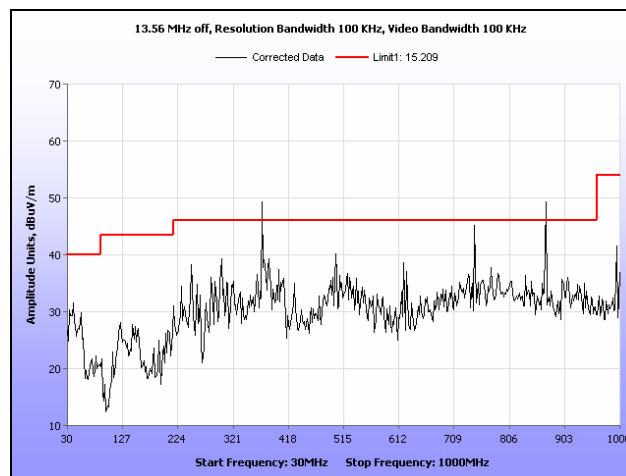
Plot 12. Field Strength of Spurious Emissions, 30 MHz – 1 GHz, 13.56 MHz Off
