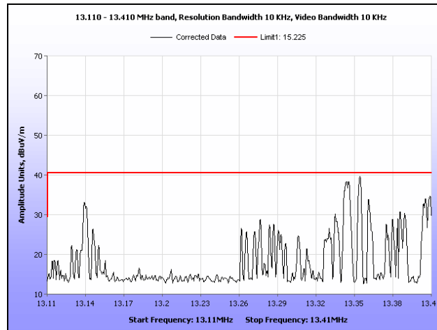
Plot 3. Field Strength of Fundamental Emission, 13.110 – 13.410 MHz Band
