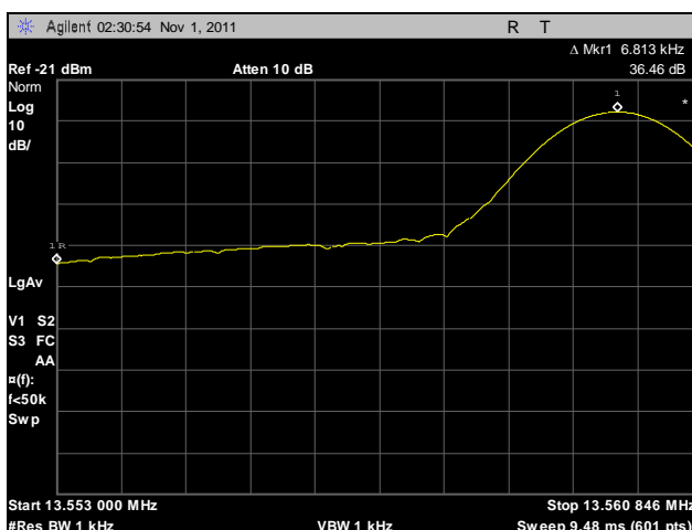
Plot 10. Field Strength of Fundamental Emission, Delta Low in 1 kHz RBW
