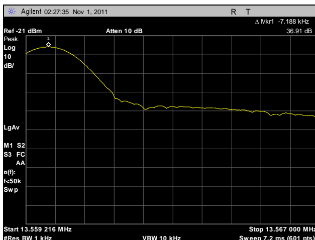
Plot 9. Field Strength of Fundamental Emission, Delta High in 1 kHz RBW
