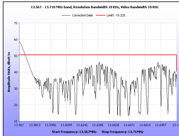
Plot 6. Field Strength of Fundamental Emission, 13.567 – 13.710 MHz Band
