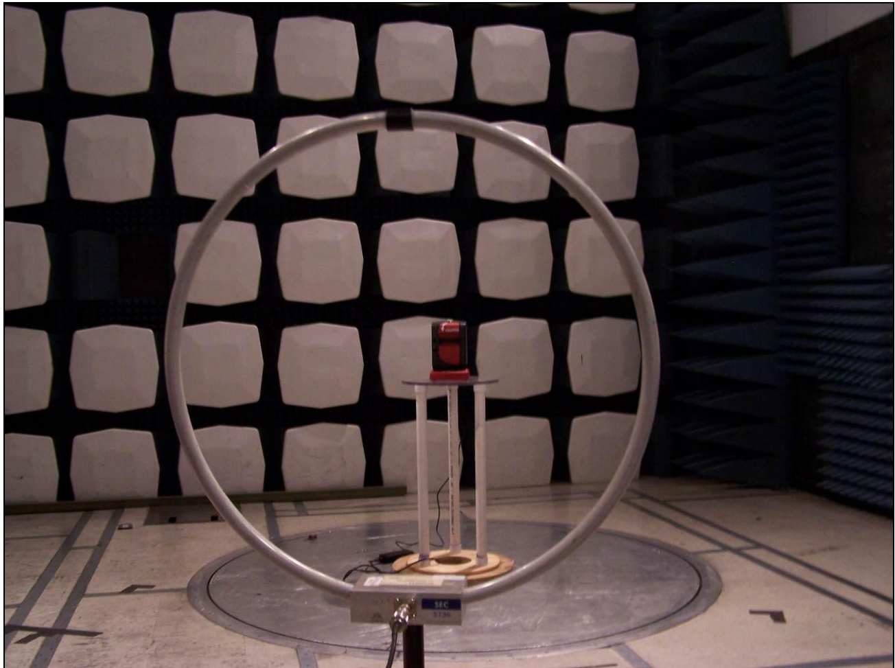
Photograph 2. Field Strength of Fundamental Emission, Test Setup
