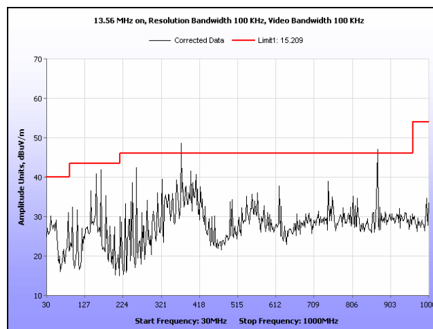
Plot 13. Field Strength of Spurious Emissions, 30 MHz – 1 GHz, 13.56 MHz On
