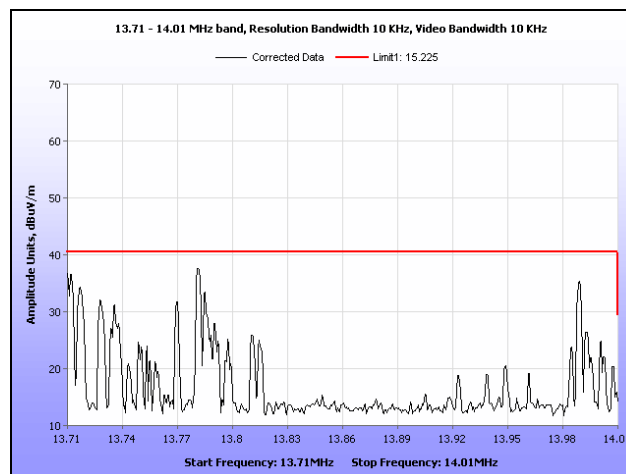
Plot 7. Field Strength of Fundamental Emission, 13.710 – 14.010 MHz Band
