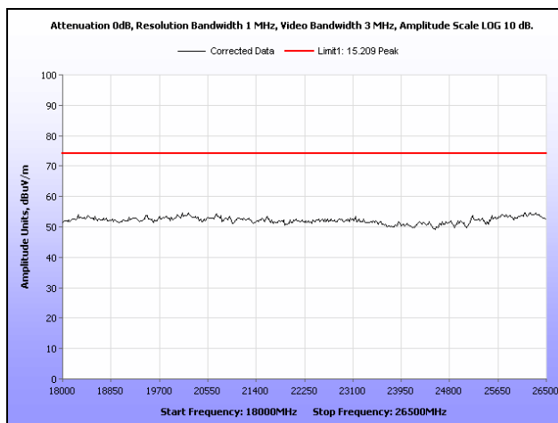
Plot 19. Radiated Spurious Emissions, Low Channel, 18 GHz – 26.5GHz, Peak
