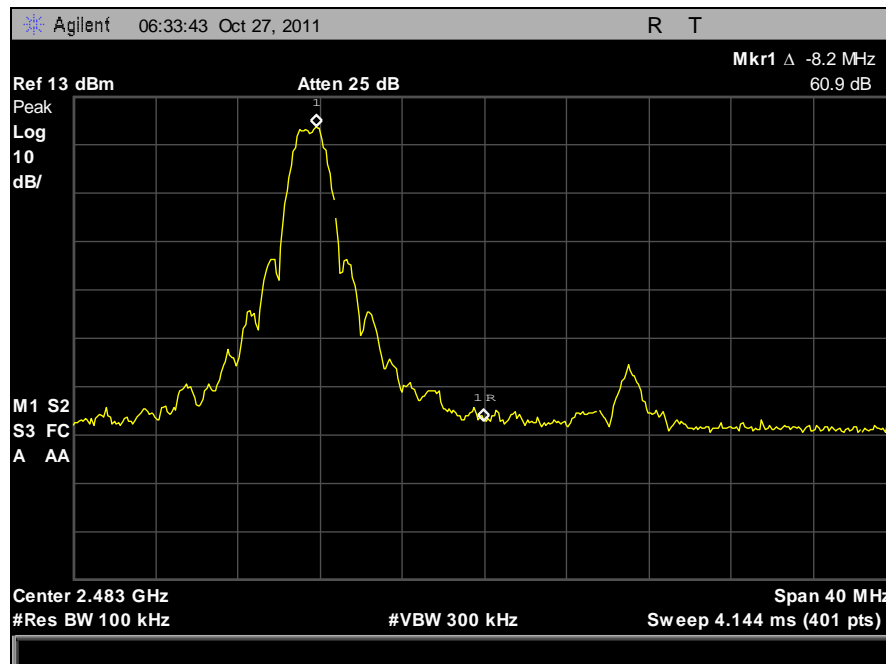
Plot 42. Conducted Band Edge, High Channel
