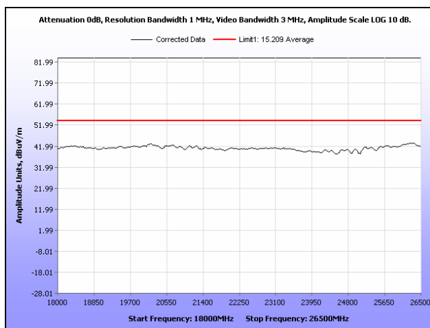
Plot 30. Radiated Spurious Emissions, High Channel, 18 GHz – 26.5GHz, Average
