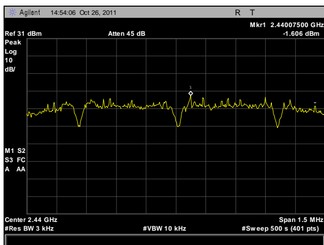
Plot 44. Peak Power Spectral Density, Mid Channel
