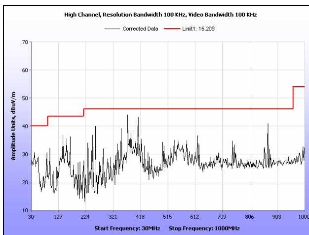
Plot 26. Radiated Spurious Emissions, High Channel, 30 MHz – 1 GHz
