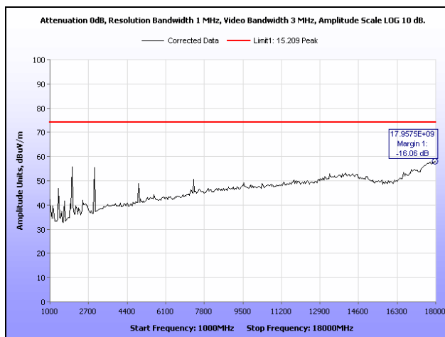
Plot 22. Radiated Spurious Emissions, Mid Channel, 1 GHz – 18 GHz, Peak
