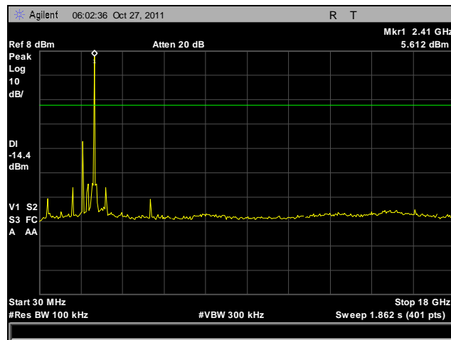
Plot 35. Conducted Spurious Emissions, Low Channel, 30 MHz – 18 GHz
