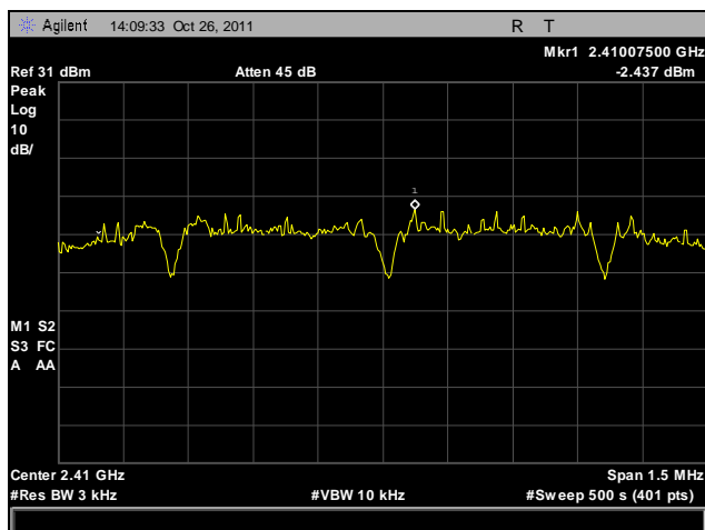
Plot 43. Peak Power Spectral Density, Low Channel
