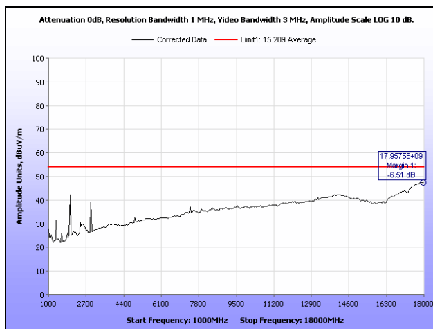
Plot 28. Radiated Spurious Emissions, High Channel, 1 GHz – 18 GHz, Average
