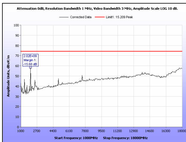
Plot 27. Radiated Spurious Emissions, High Channel, 1 GHz – 18 GHz, Peak
