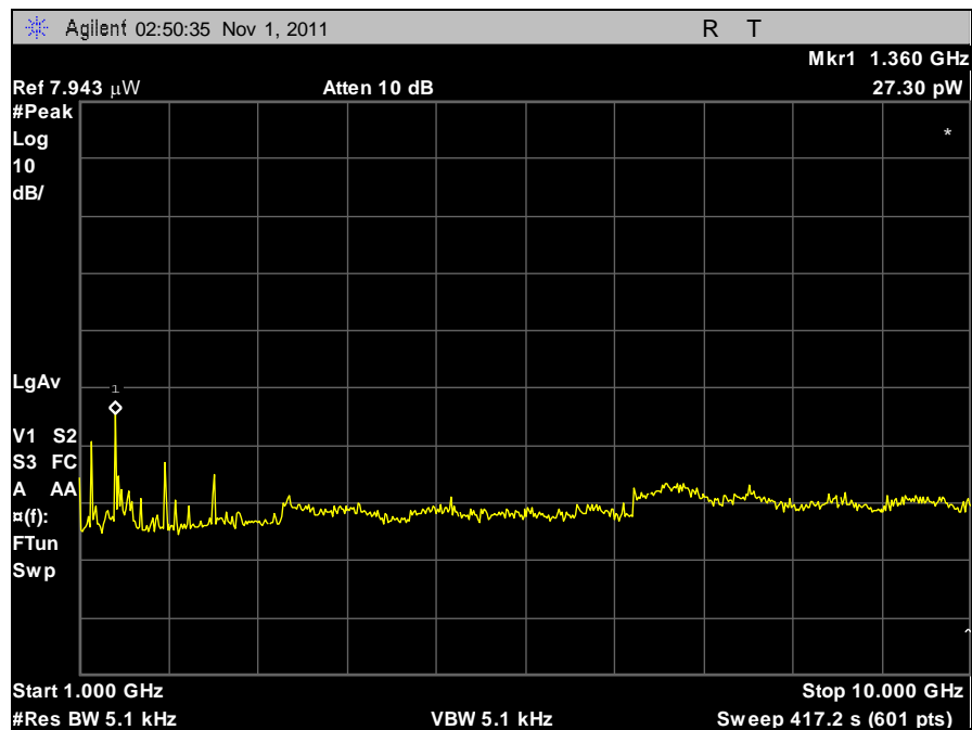
Plot 47. Receiver Spurious Emission, 1 GHz – 10 GHz
