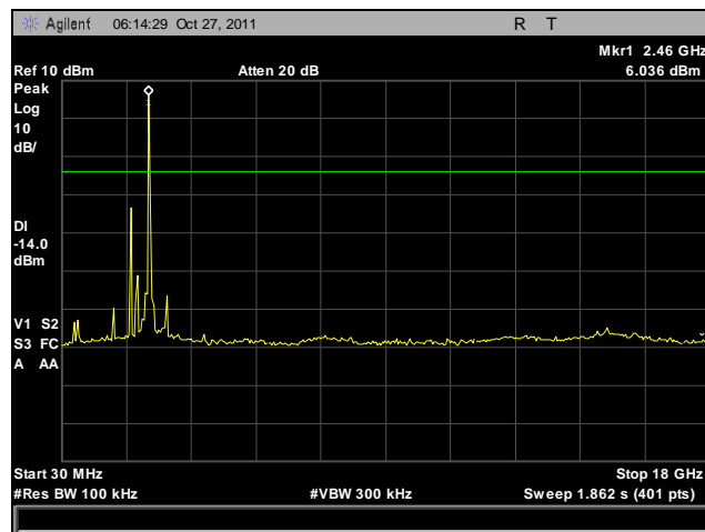
Plot 39. Conducted Spurious Emissions, High Channel, 30 MHz – 18 GHz
