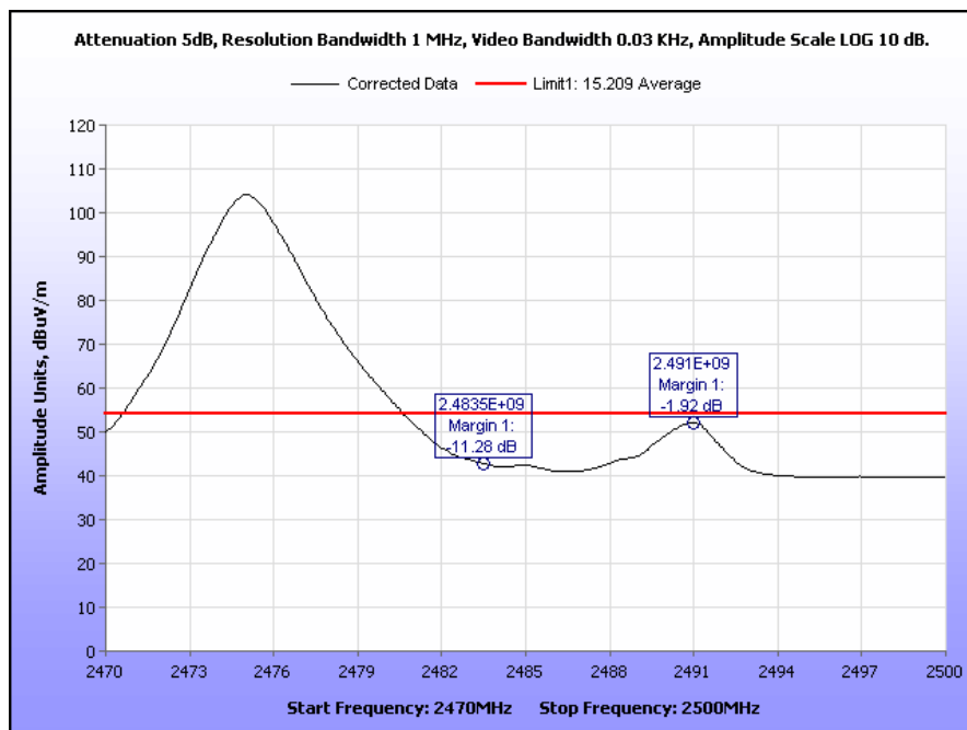
Plot 33. Radiated Restricted Band Edge, High Channel, Average
