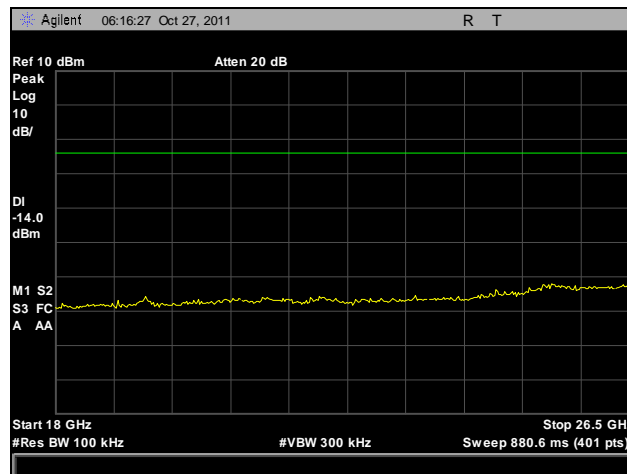
Plot 40. Conducted Spurious Emissions, High Channel, 18 GHz – 26.5 GHz
