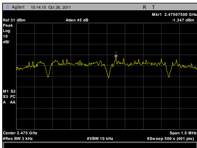
Plot 45. Peak Power Spectral Density, High Channel
