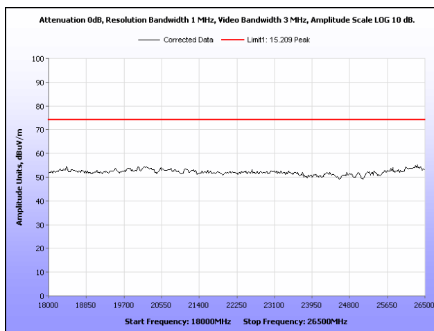
Plot 24. Radiated Spurious Emissions, Mid Channel, 18 GHz – 26.5GHz, Peak
