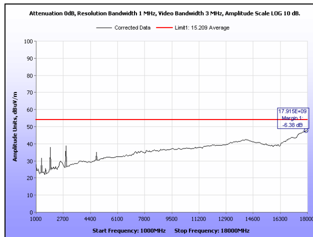
Plot 18. Radiated Spurious Emissions, Low Channel, 1 GHz – 18 GHz, Average
