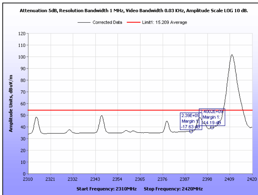
Plot 31. Radiated Restricted Band Edge, Low Channel, Average
