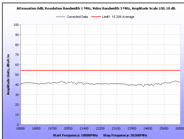
Plot 25. Radiated Spurious Emissions, Mid Channel, 18 GHz – 26.5GHz, Average
