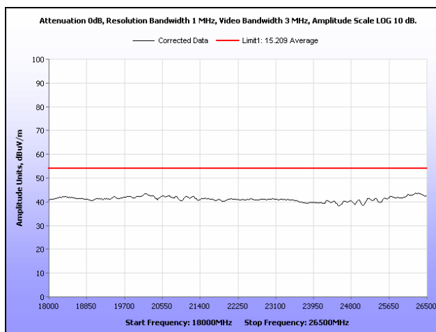
Plot 20. Radiated Spurious Emissions, Low Channel, 18 GHz – 26.5GHz, Average
