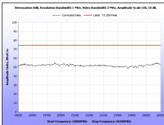
Plot 29. Radiated Spurious Emissions, High Channel, 18 GHz – 26.5GHz, Peak
