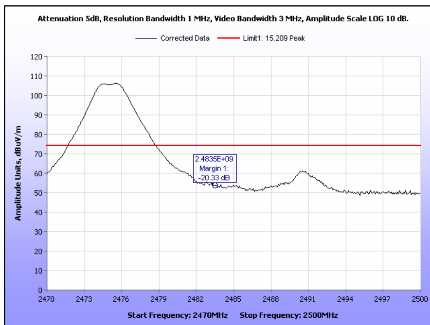
Plot 34. Radiated Restricted Band Edge, High Channel, Peak
