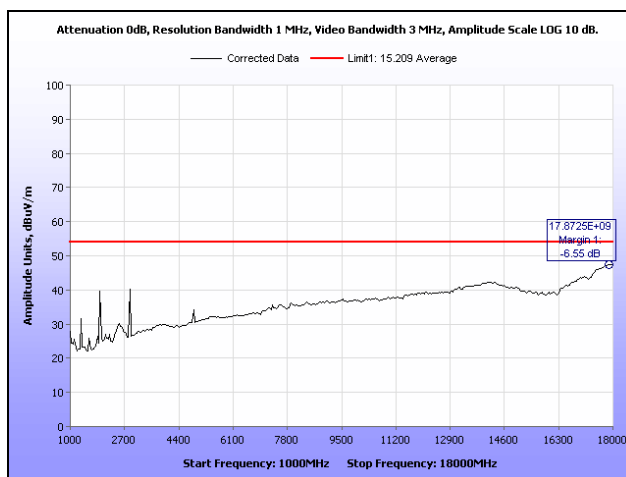
Plot 23. Radiated Spurious Emissions, Mid Channel, 1 GHz – 18 GHz, Average
