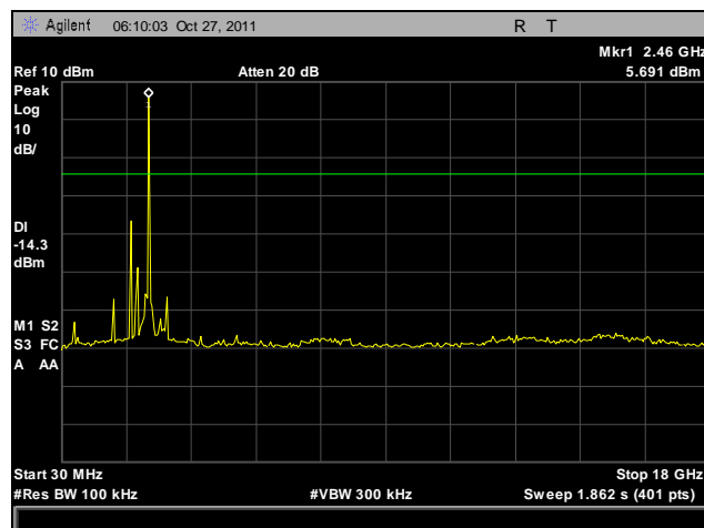
Plot 37. Conducted Spurious Emissions, Mid Channel, 30 MHz – 18 GHz
