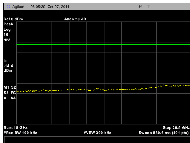
Plot 36. Conducted Spurious Emissions, Low Channel, 18 GHz – 26.5 GHz
