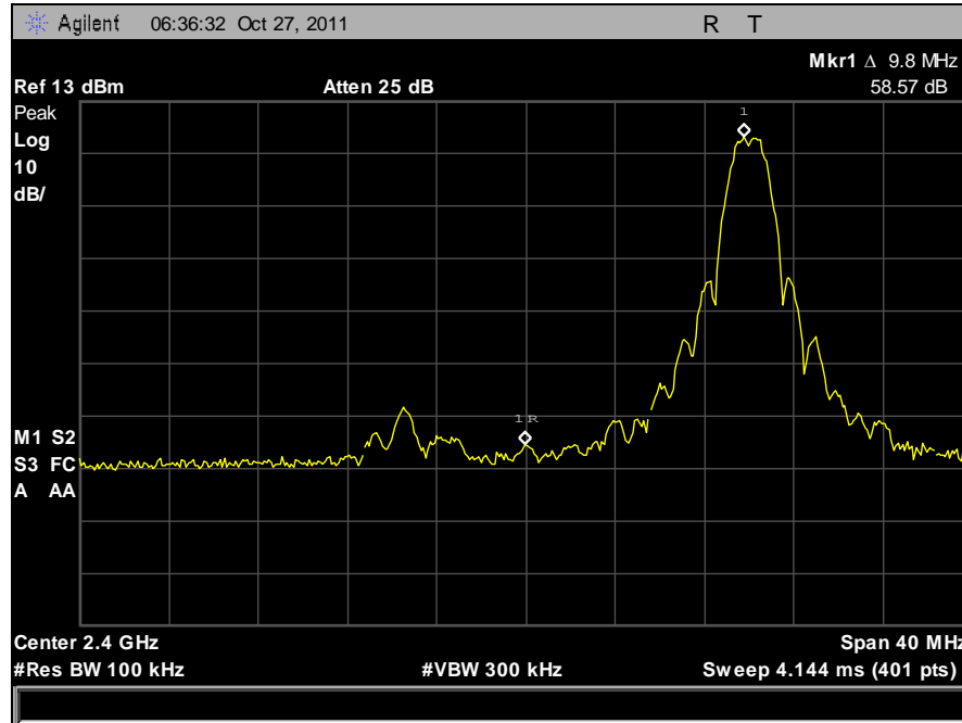
Plot 41. Conducted Band Edge, Low Channel
