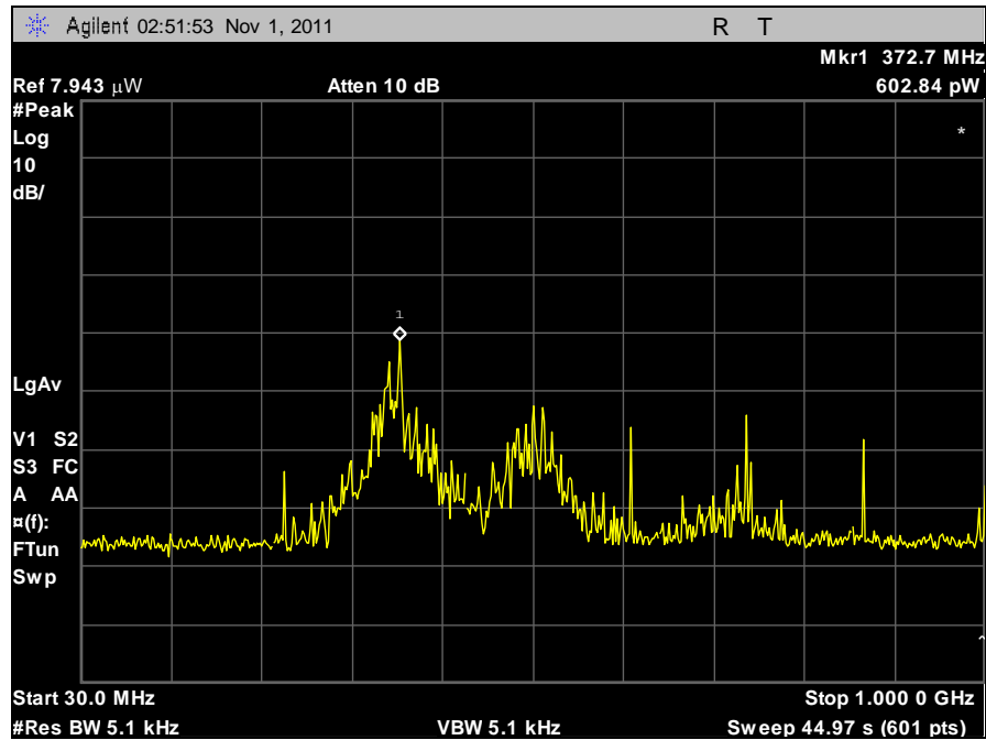
Plot 46. Receiver Spurious Emission, 30 MHz – 1 GHz
