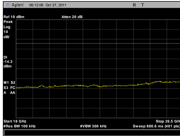
Plot 38. Conducted Spurious Emissions, Mid Channel, 18 GHz – 26.5 GHz
