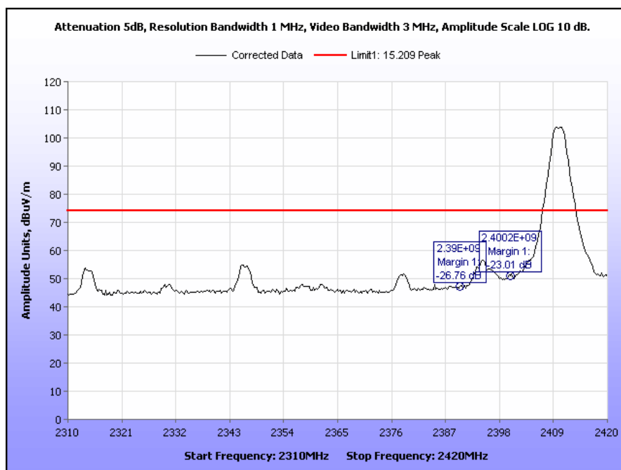
Plot 32. Radiated Restricted Band Edge, Low Channel, Peak
